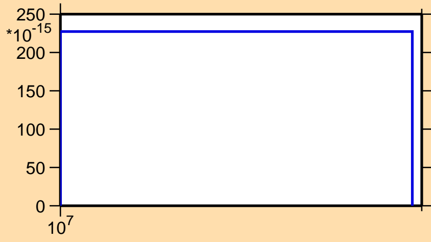
\sigma vs. E for ^{133}\text{Ce}(\text{mt } 45)
