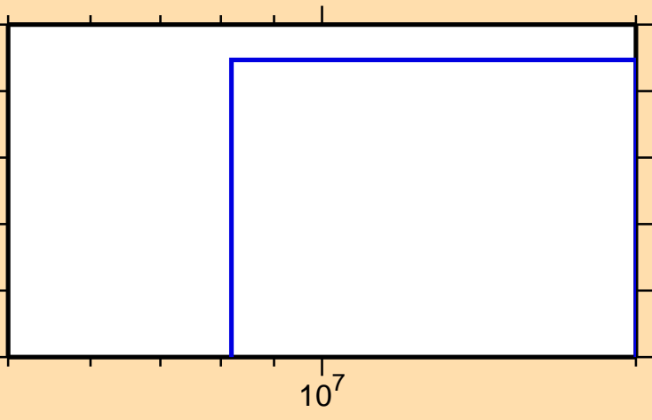
\sigma vs. E for ^{133}\text{Ce}(\text{mt } 45)
