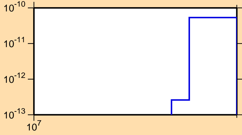
\sigma vs. E for ^{133}\text{Ce}(\text{mt } 34)
