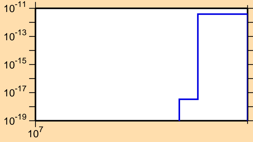
\sigma vs. E for ^{133}\text{Ce}(n,nt)
