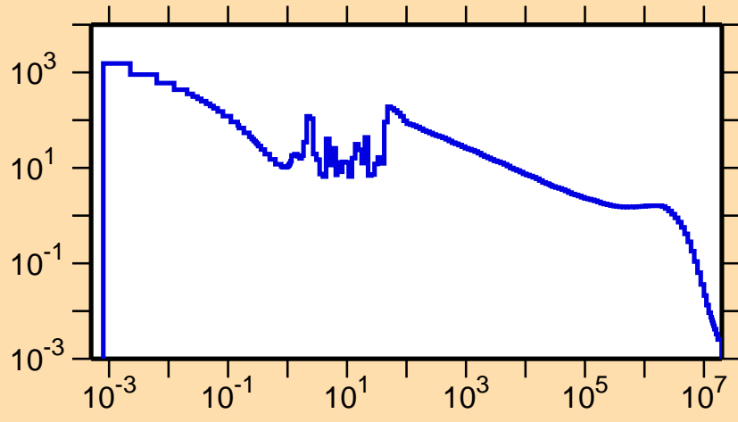
\sigma vs. E for ^{133}\text{Ce}(n,\gamma)
