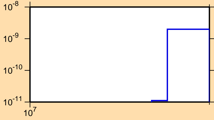
\sigma vs. E for ^{133}\text{Ce}(n,\text{pt})
