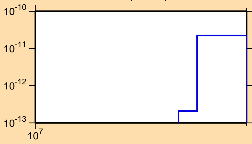
\sigma vs. E for ^{133}\text{Ce} (mt 45)
