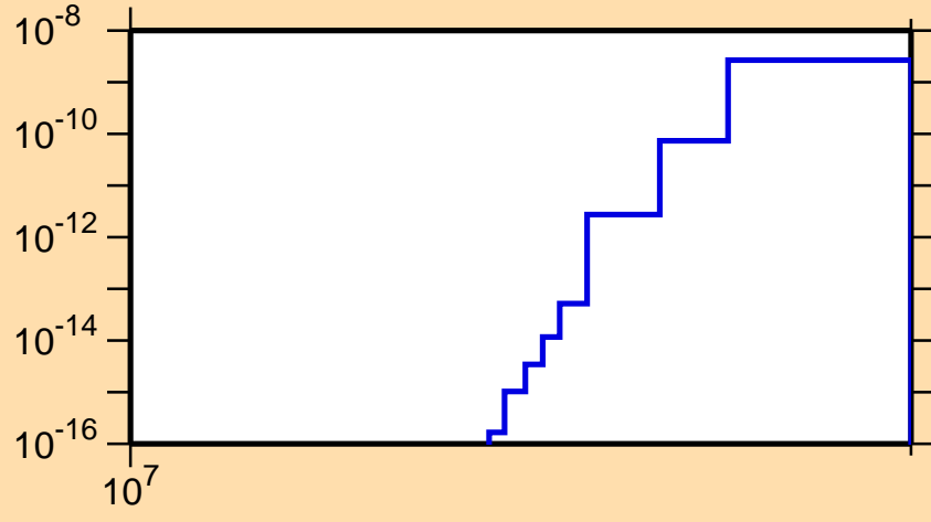
\sigma vs. E for ^{134}\text{Ce}(n,\text{pd})
