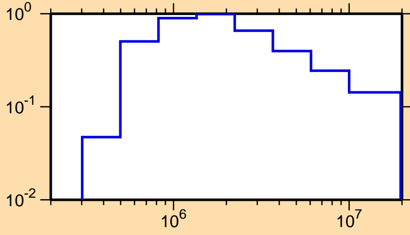
\sigma vs. E for ^{134}\text{Ce}(n,n_1)
