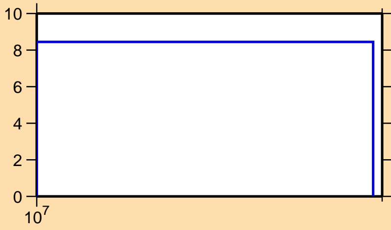
\Delta\sigma/\sigma vs. E for ^{134}\text{Ce}(n,\text{nonel.})
