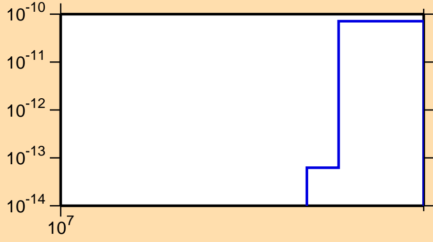
\sigma vs. E for ^{135}\text{Ce}(n,\text{pt})
