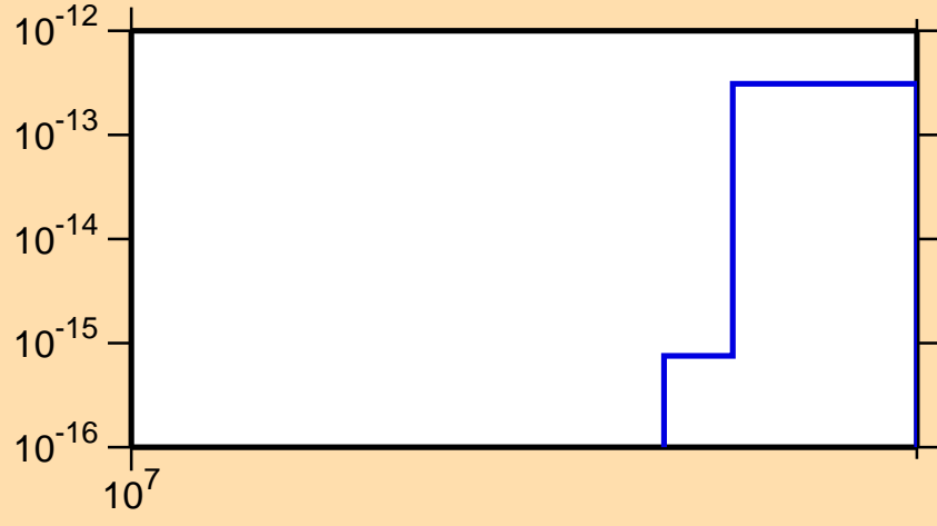
\sigma vs. E for ^{135}\text{Ce}(\text{mt } 45)
