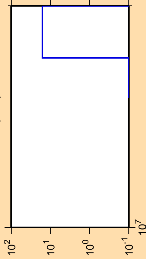
\Delta\sigma/\sigma vs. E for ^{135}\text{Ce}(n,nt)
