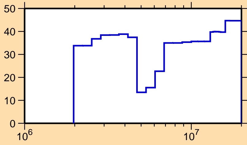
\Delta\sigma/\sigma vs. E for ^{135}\text{Ce}(n,n_1)
