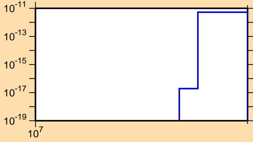
\sigma vs. E for ^{135}\text{Ce}(n,nt)
