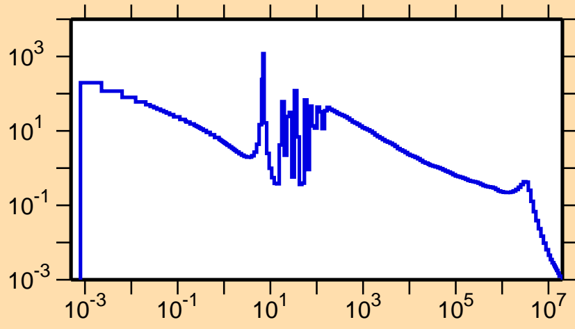
\sigma vs. E for ^{135}\text{Ce}(n,\gamma)
