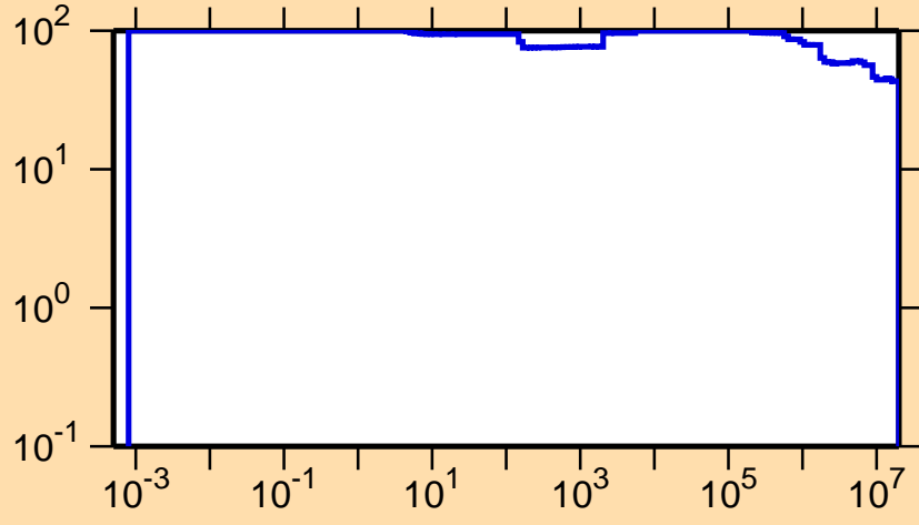
\Delta\sigma/\sigma vs. E for ^{135}\text{Ce}(n,p)
