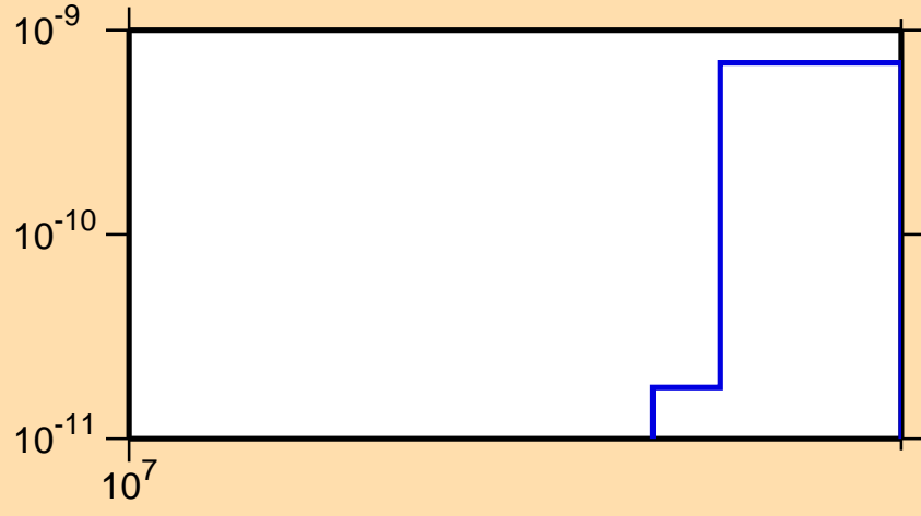
\sigma vs. E for ^{135}\text{Ce}(n,\text{pd})
