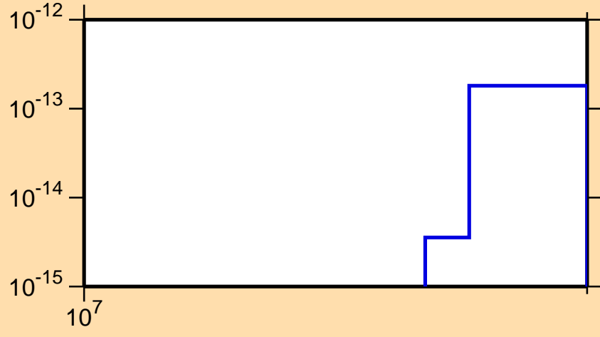
\sigma vs. E for ^{135}\text{Ce}(\text{mt117})
