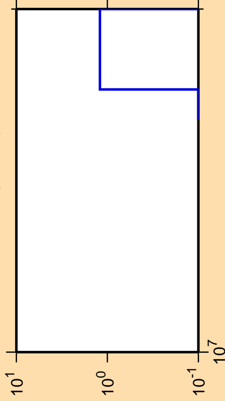
\Delta\sigma/\sigma vs. E for ^{135}\text{Ce}(\text{mt } 45)
