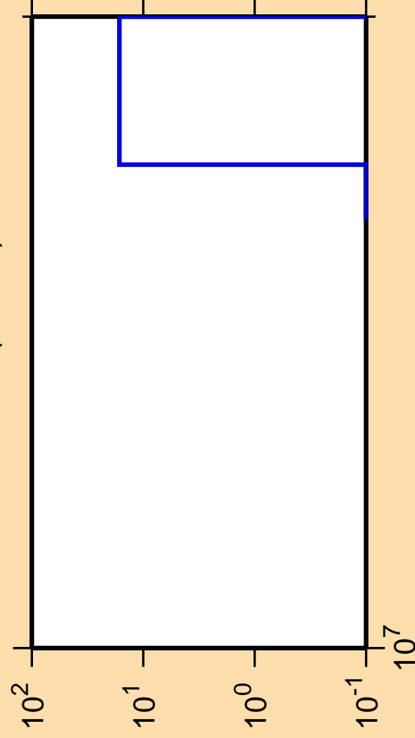
\Delta\sigma/\sigma vs. E for ^{135}\text{Ce}(\text{mt } 34)
