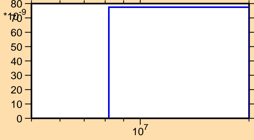
\sigma vs. E for ^{135}\text{Ce}(n,2np)
