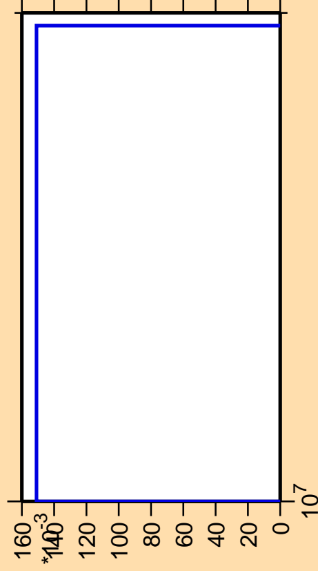
\Delta\sigma/\sigma vs. E for ^{135}\text{Ce} (mt 34)
