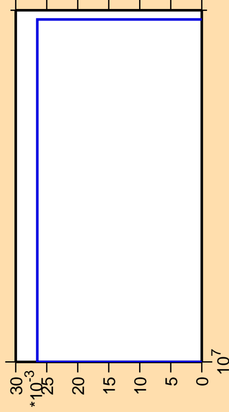
\Delta\sigma/\sigma vs. E for ^{135}\text{Ce} (mt 45)
