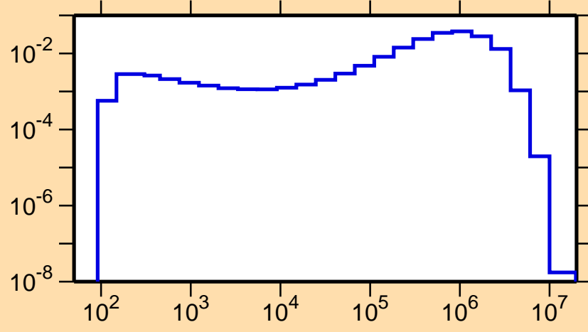
\sigma vs. E for ^{135}\text{Ce}(n,n_3)
