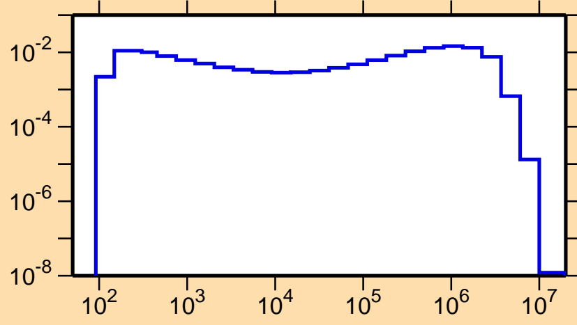
\sigma vs. E for ^{135}\text{Ce}(n,n_2)
