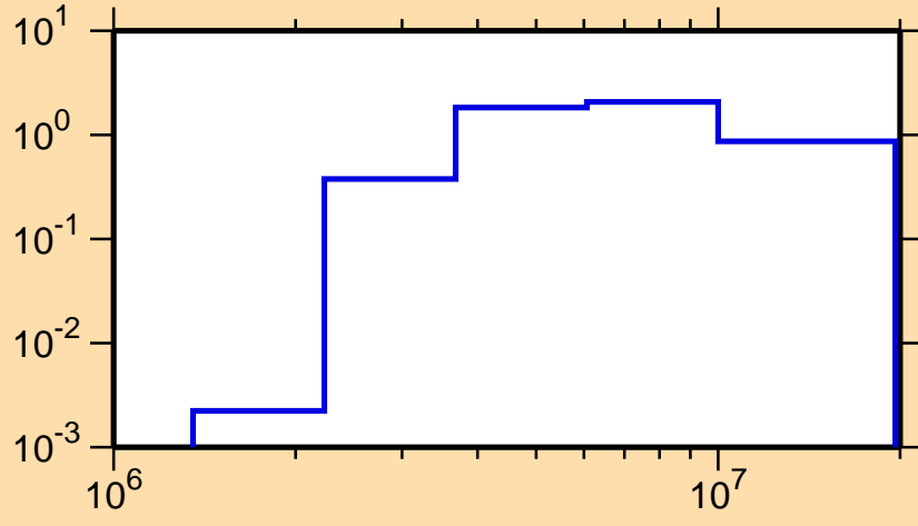
\sigma vs. E for ^{135}\text{Ce}(n,n\text{cont.})
