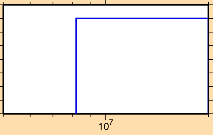
\sigma vs. E for ^{135}\text{Ce}(n,\text{pd})
