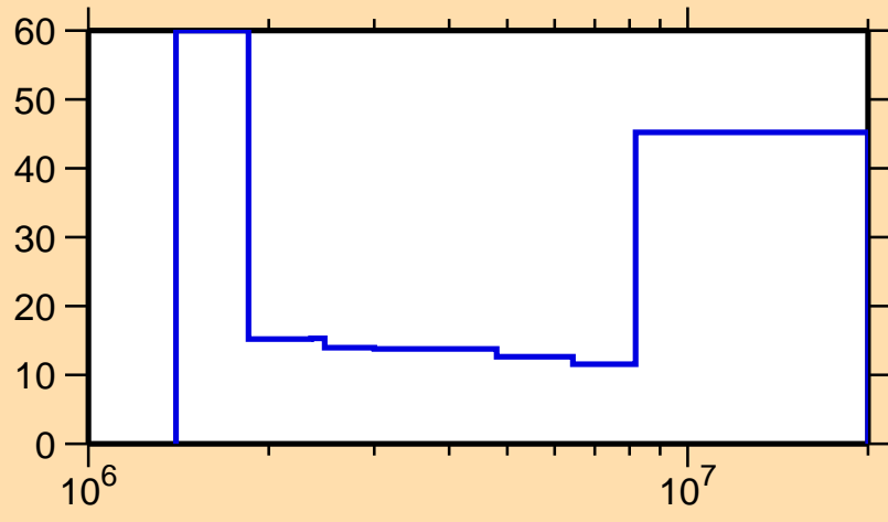
\Delta\sigma/\sigma vs. E for ^{135}\text{Ce}(n,n\text{cont.})
