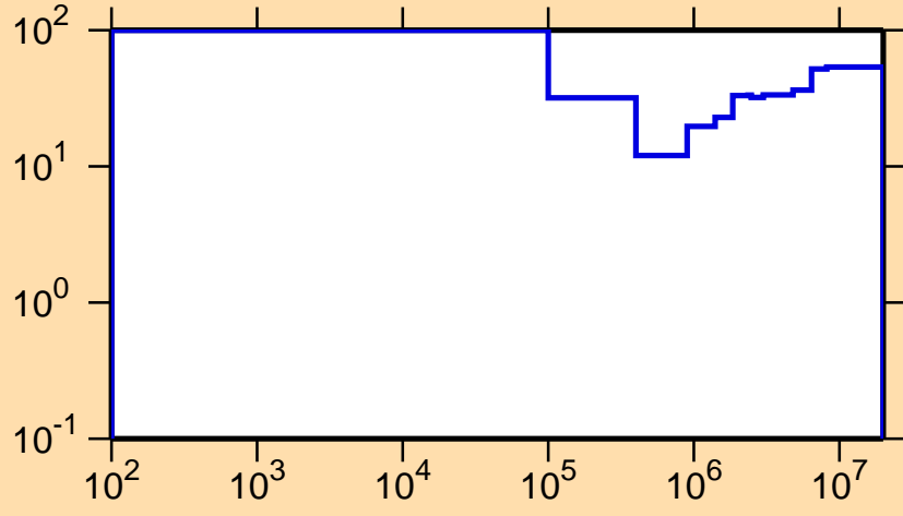
\Delta\sigma/\sigma vs. E for ^{135}\text{Ce}(n,n_1)
