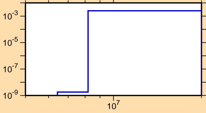
\sigma vs. E for ^{135}\text{Ce}(n,d)
