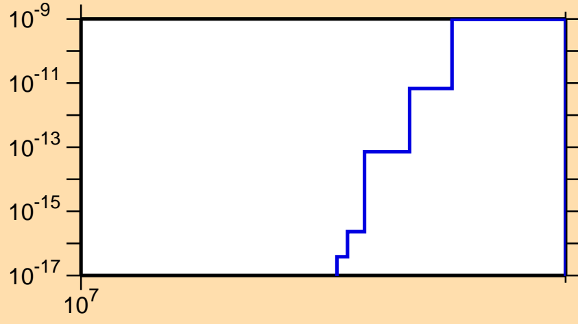
\sigma vs. E for ^{136}\text{Ce}(n,\text{pd})
