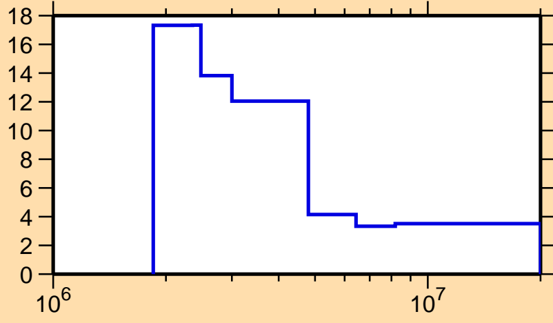
\Delta\sigma/\sigma vs. E for ^{137}\text{Ce}(n,\text{tot.})
