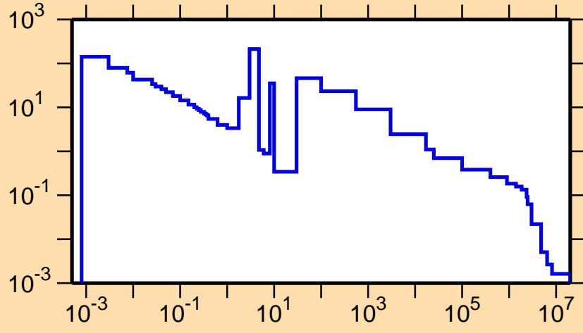
\sigma vs. E for ^{137}\text{Ce}(n,\gamma)
