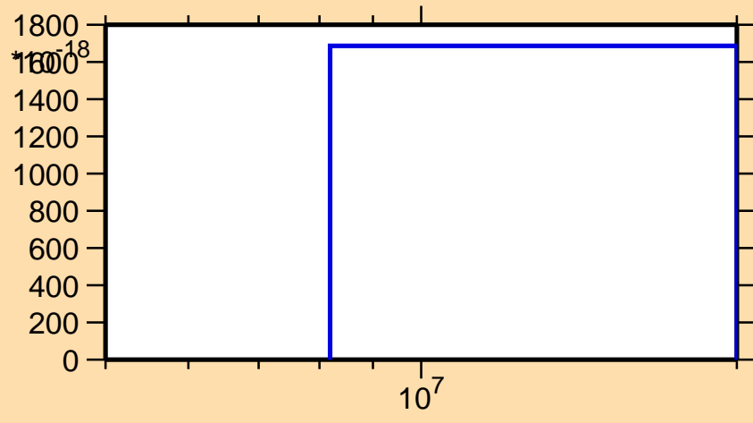
\sigma vs. E for ^{137}\text{Ce} (mt 34)
