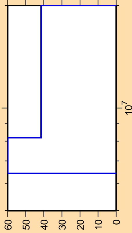
\Delta\sigma/\sigma vs. E for ^{137}\text{Ce}(n,n\alpha)
