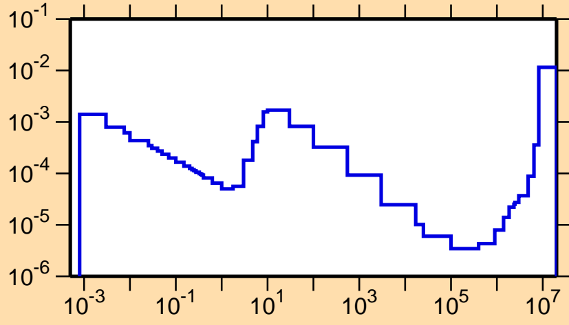
\sigma vs. E for ^{137}\text{Ce}(n,\alpha)
