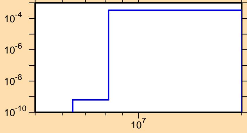
\sigma vs. E for ^{137}\text{Ce}(n,n\alpha)
