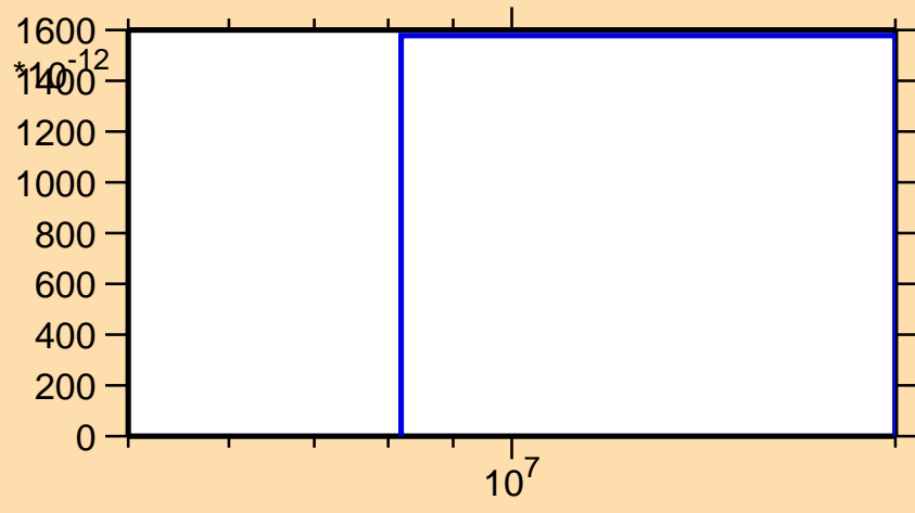
\sigma vs. E for ^{139}\text{Ce}(n,\text{He}3)
