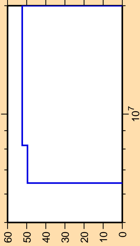
\Delta\sigma/\sigma vs. E for ^{139}\text{Ce}(n,\gamma)
