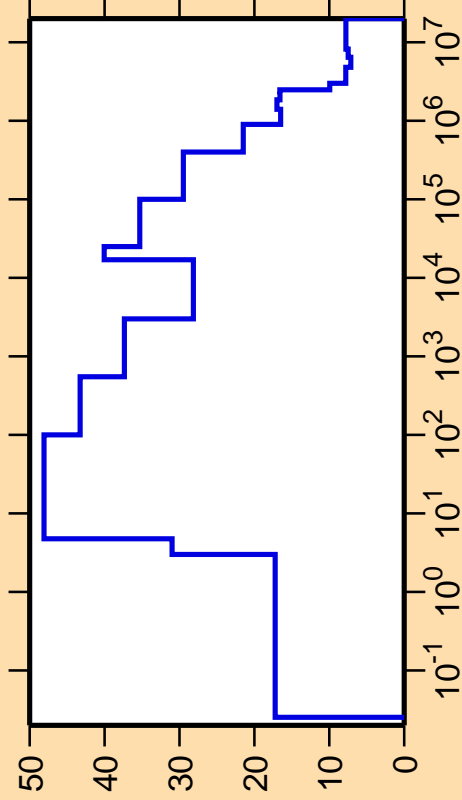
\Delta\sigma/\sigma vs. E for ^{139}\text{Ce}(n,\text{nonel.})
