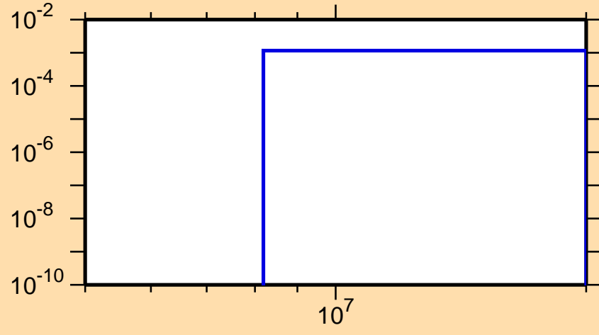
\sigma vs. E for ^{139}\text{Ce}(n,d)
