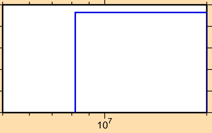
\sigma vs. E for ^{139}\text{Ce}(n,\text{pt})
