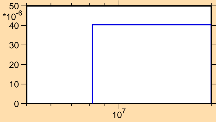
\sigma vs. E for ^{139}\text{Ce}(n,t)
