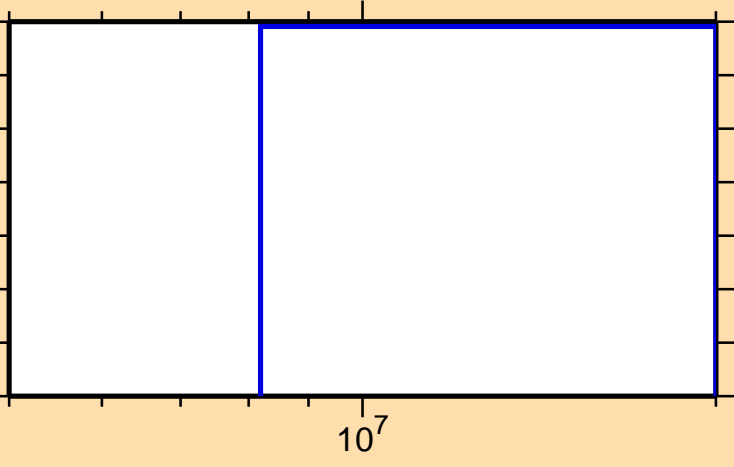
\sigma vs. E for ^{139}\text{Ce}(n,2np)
