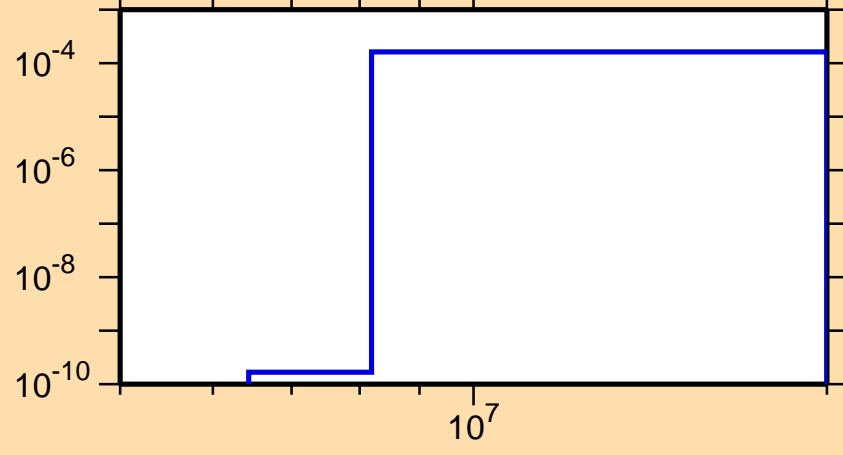
\sigma vs. E for ^{139}\text{Ce}(n,n\alpha)
