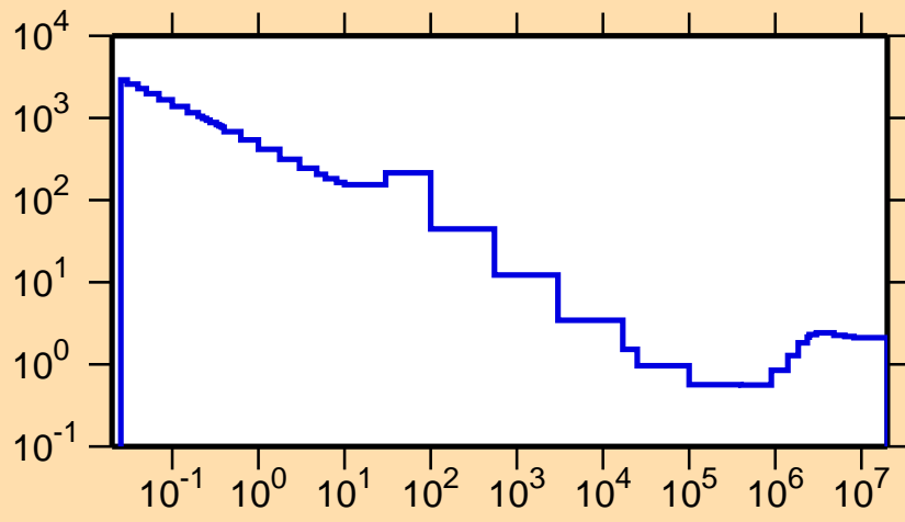
\sigma vs. E for ^{139}\text{Ce}(n,\text{nonel.})
