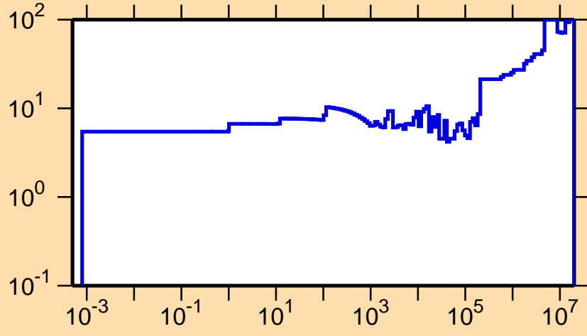
\Delta\sigma/\sigma vs. E for ^{140}\text{Ce}(n,\gamma)
