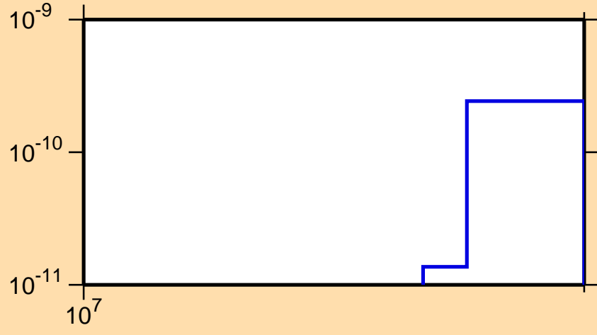
\sigma vs. E for ^{140}\text{Ce}(n,p\alpha)
