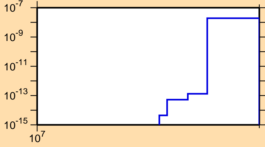
\sigma vs. E for ^{140}\text{Ce}(n,\text{nd})
