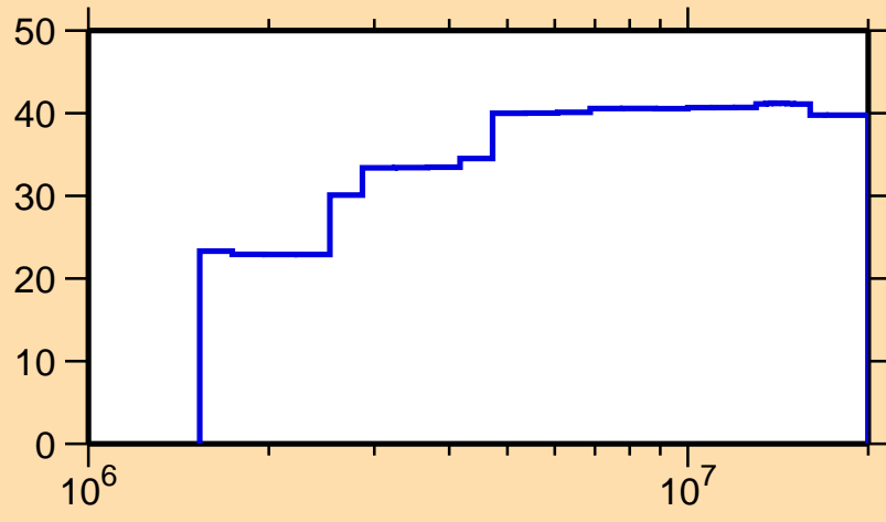
\Delta\sigma/\sigma vs. E for ^{140}\text{Ce}(n,n_1)
