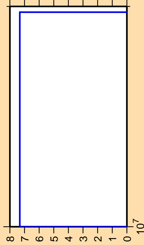
\Delta\sigma/\sigma vs. E for ^{140}\text{Ce}(n,p\alpha)
