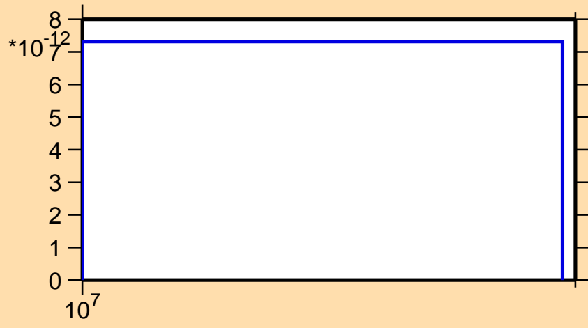
\sigma vs. E for ^{140}\text{Ce}(n,2n\alpha)
