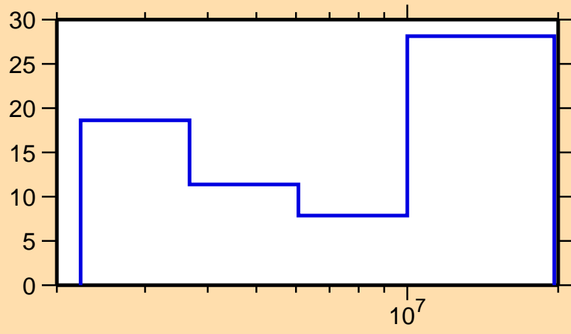
\Delta\sigma/\sigma vs. E for ^{140}\text{Ce}(n,n\text{cont.})
