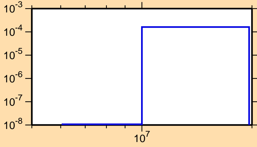
\sigma vs. E for ^{140}\text{Ce}(n,n\alpha)
