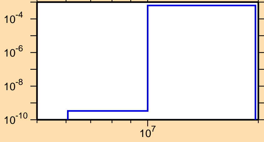
\sigma vs. E for ^{140}\text{Ce}(n,d)
