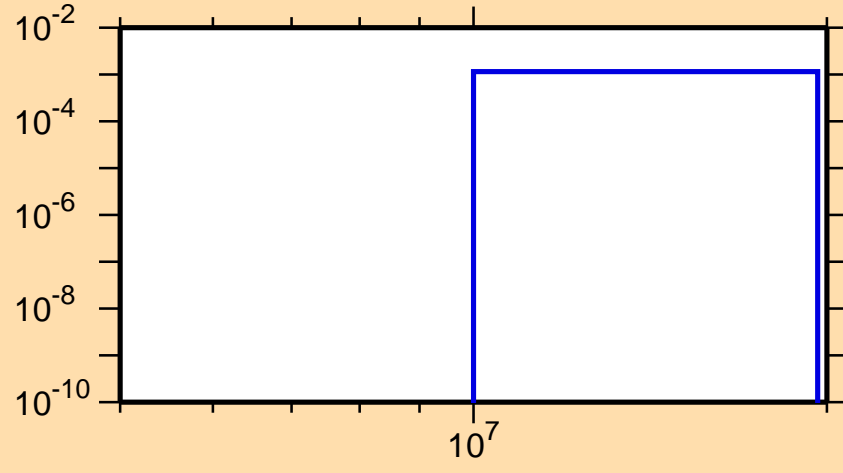
\sigma vs. E for ^{140}\text{Ce}(n,np)
