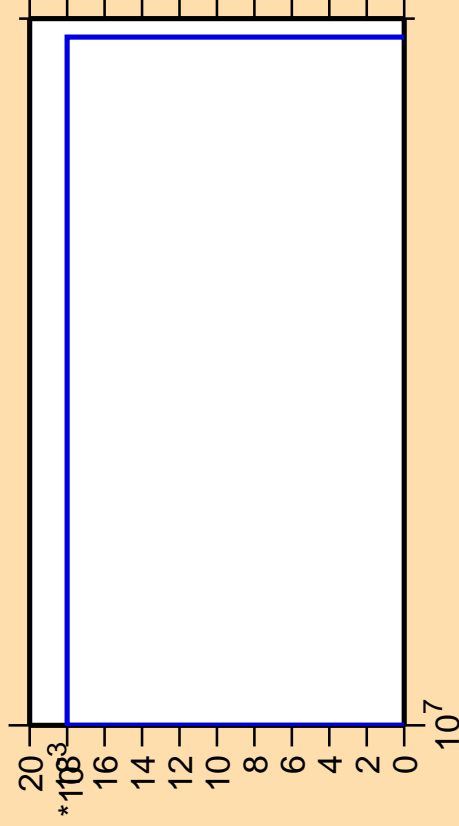
\Delta\sigma/\sigma vs. E for ^{140}\text{Ce}(n,\text{pd})
