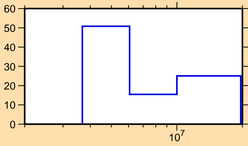
\Delta\sigma/\sigma vs. E for ^{140}\text{Ce}(n,p)
