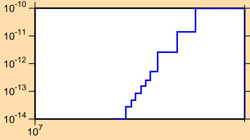
\sigma vs. E for ^{142}\text{Ce}(n,p\alpha)
