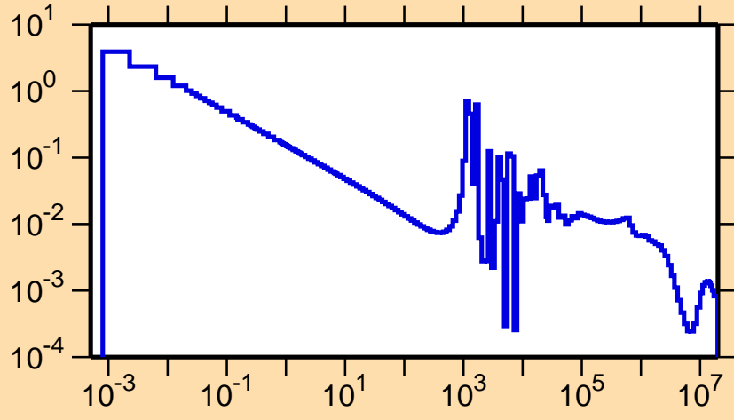
\sigma vs. E for ^{142}\text{Ce}(n,\gamma)
