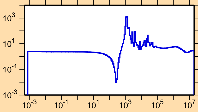
\sigma vs. E for ^{142}\text{Ce}(n,\text{el.})
