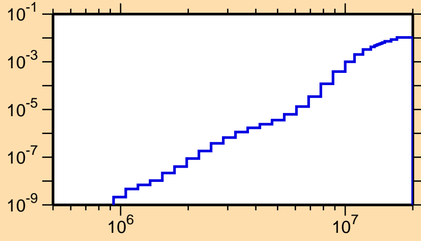
\sigma vs. E for ^{142}\text{Ce}(n,\alpha)
