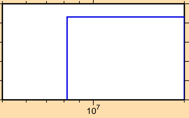
\sigma vs. E for ^{142}\text{Ce} (mt 11)
