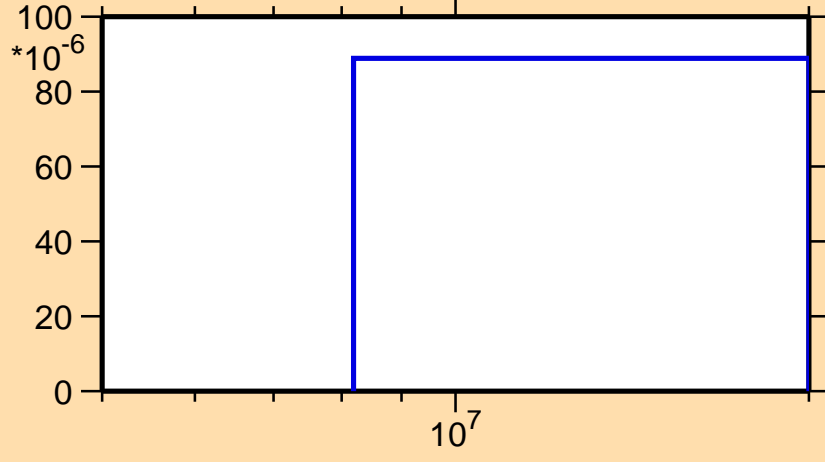
\sigma vs. E for ^{142}\text{Ce}(n,t)
