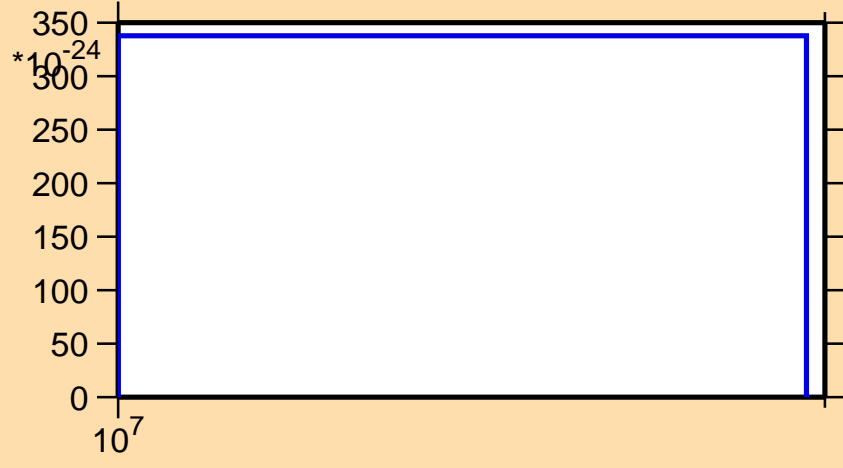
\sigma vs. E for ^{143}\text{Ce}(\text{mt } 11)
