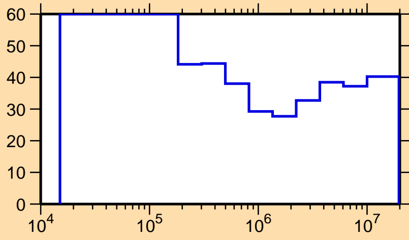
\Delta\sigma/\sigma vs. E for ^{143}\text{Ce}(n,n_1)
