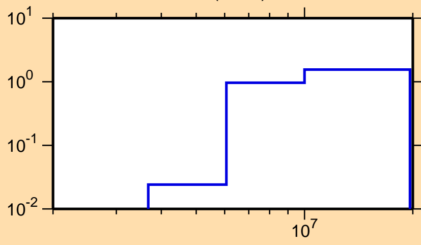
\sigma vs. E for ^{143}\text{Ce}(n,2n)
