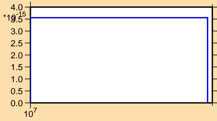
\sigma vs. E for ^{143}\text{Ce}(n,3n\alpha)
