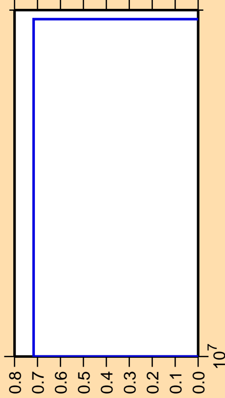
\Delta\sigma/\sigma vs. E for ^{143}\text{Ce}(n,\text{He3})
