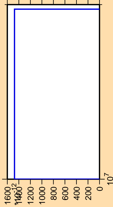
\Delta\sigma/\sigma vs. E for ^{143}\text{Ce}(\text{mt } 11)
