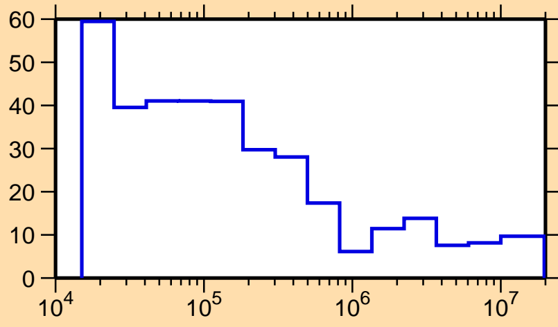
\Delta\sigma/\sigma vs. E for ^{143}\text{Ce}(n,\text{el.})
