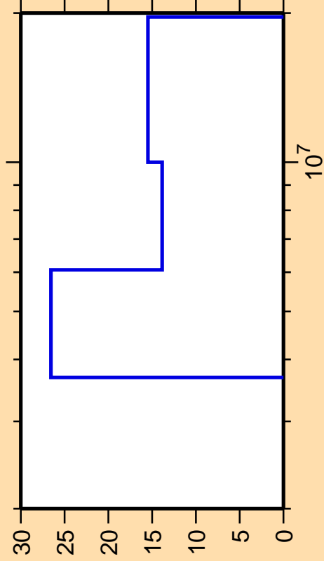
\Delta\sigma/\sigma vs. E for ^{143}\text{Ce}(n,2n)
