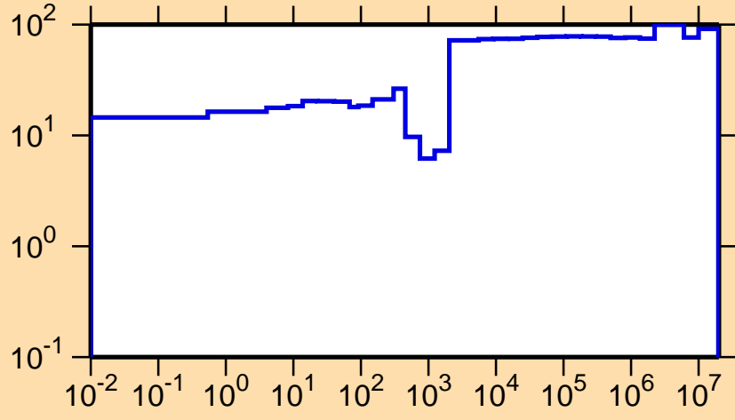
\Delta\sigma/\sigma vs. E for ^{143}\text{Ce}(n,\gamma)
