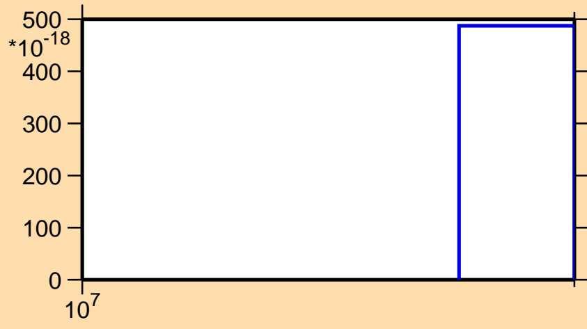
\sigma vs. E for ^{144}\text{Ce} (mt 11)
