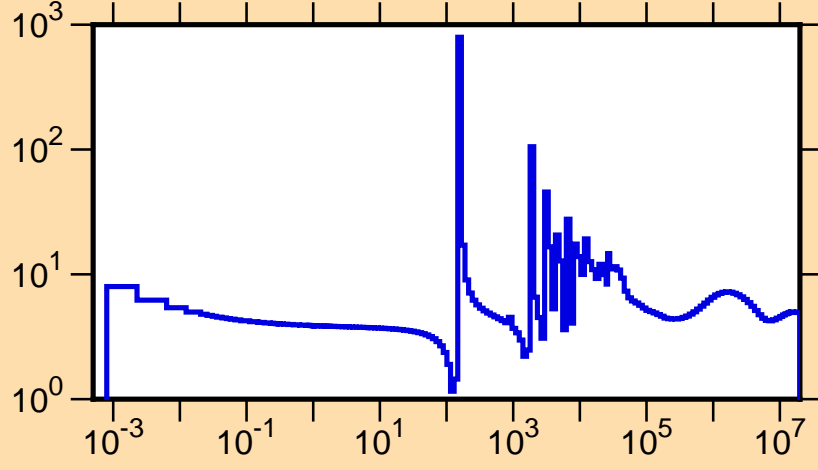
\sigma vs. E for ^{144}\text{Ce}(n,\text{tot.})
