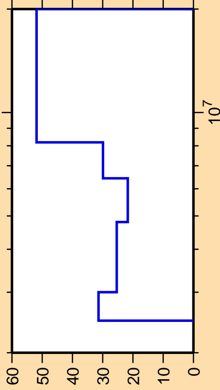
\Delta\sigma/\sigma vs. E for ^{144}\text{Ce}(n,n\text{cont.})
