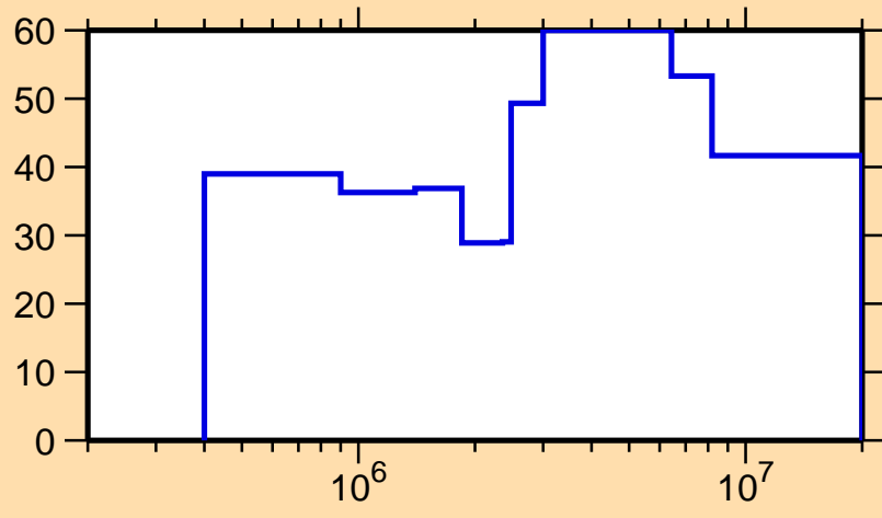
\Delta\sigma/\sigma vs. E for ^{144}\text{Ce}(n,n_1)
