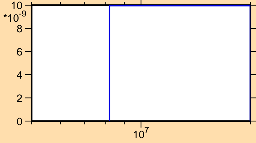
\sigma vs. E for ^{144}\text{Ce}(n,nt)
