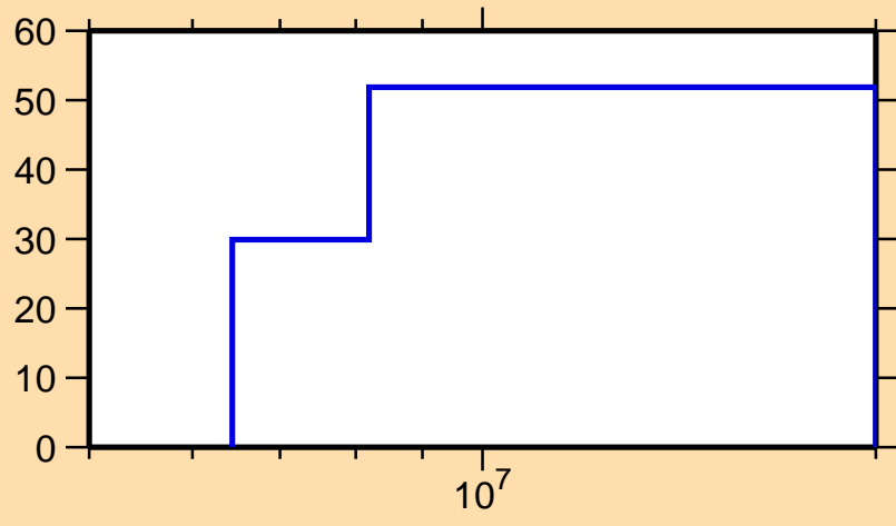
\Delta\sigma/\sigma vs. E for ^{144}\text{Ce}(n,ncont.)
