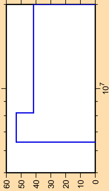
\Delta\sigma/\sigma vs. E for ^{144}\text{Ce}(n,n_1)
