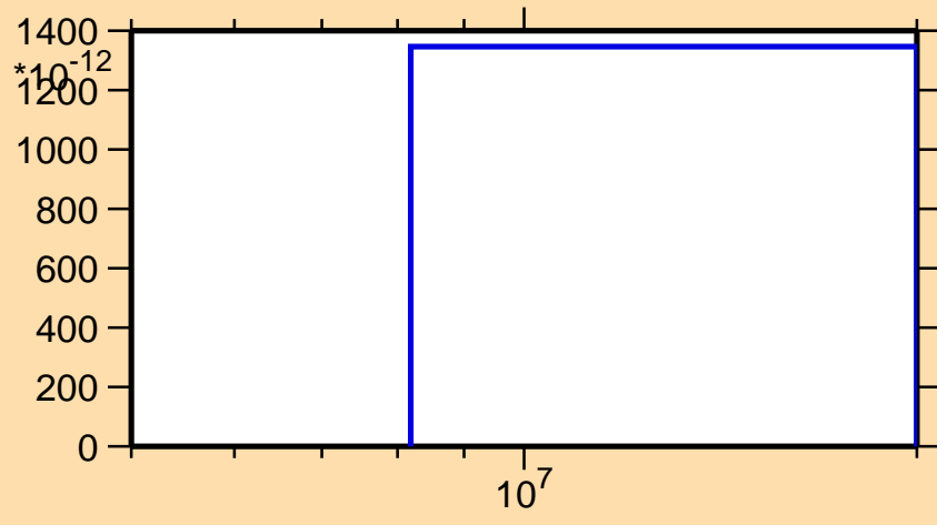
\sigma vs. E for ^{144}\text{Ce}(n,\text{nd})
