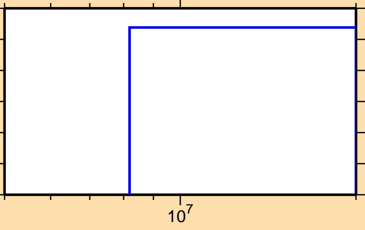
\sigma vs. E for ^{144}\text{Ce}(n,d)
