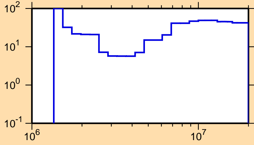
\Delta\sigma/\sigma vs. E for ^{145}\text{Ce}(n,n\text{cont.})
