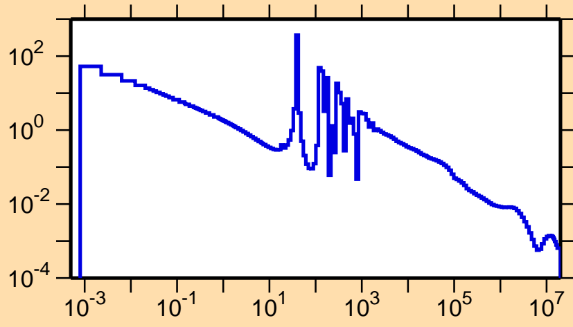
\sigma vs. E for ^{145}\text{Ce}(n,\gamma)
