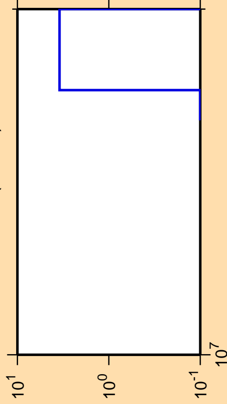
\Delta\sigma/\sigma vs. E for ^{145}\text{Ce}(n,\text{He}3)
