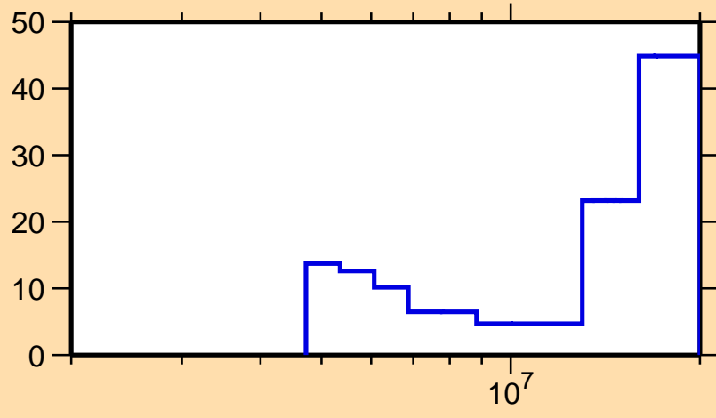
\Delta\sigma/\sigma vs. E for ^{145}\text{Ce}(n,2n)
