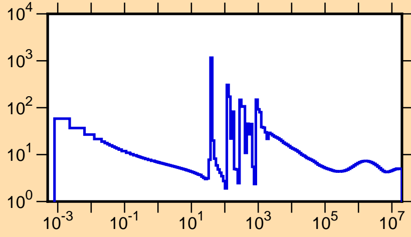
\sigma vs. E for ^{145}\text{Ce}(n,\text{tot.})
