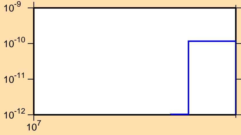
\sigma vs. E for ^{145}\text{Ce}(n,3n\alpha)
