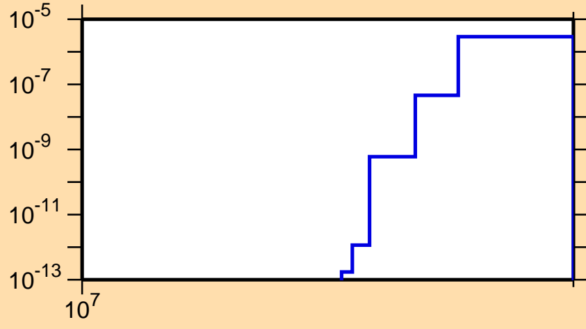
\sigma vs. E for ^{145}\text{Ce}(n,nt)
