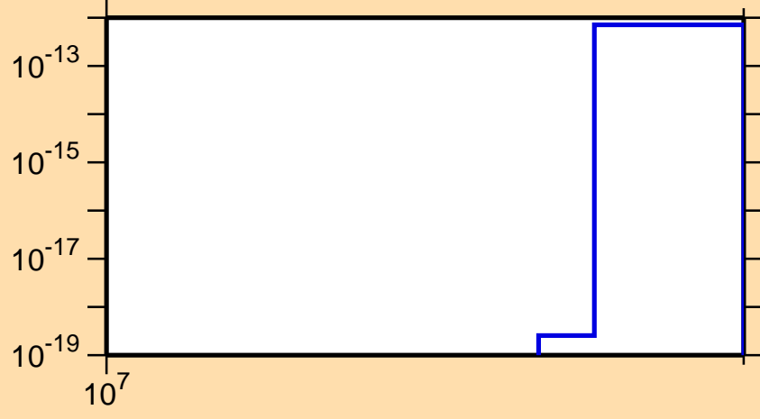
\sigma vs. E for ^{145}\text{Ce}(n,\text{He}3)
