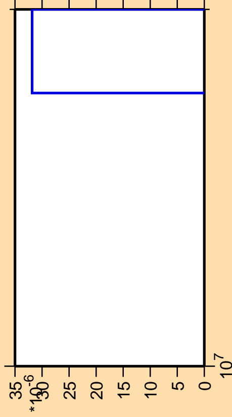
\Delta\sigma/\sigma vs. E for ^{145}\text{Ce} (mt 11)
