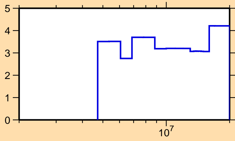
\Delta\sigma/\sigma vs. E for ^{145}\text{Ce}(n,\text{el.})
