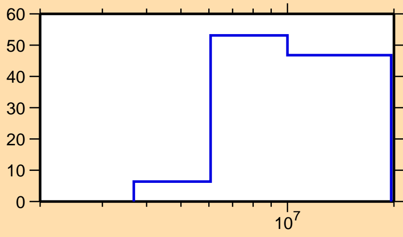
\Delta\sigma/\sigma vs. E for ^{145}\text{Ce}(n,p)
