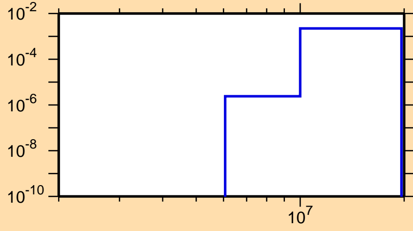
\sigma vs. E for ^{145}\text{Ce}(n,p)
