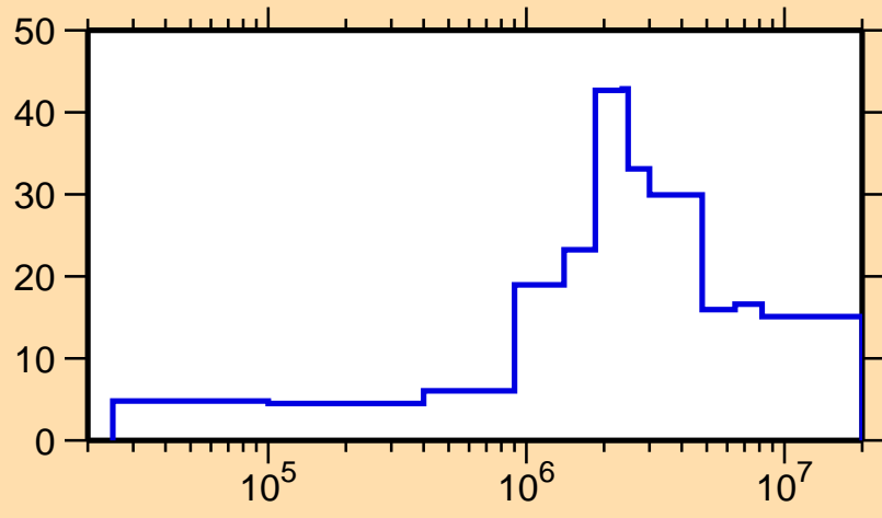
\Delta\sigma/\sigma vs. E for ^{145}\text{Ce}(n,n_1)
