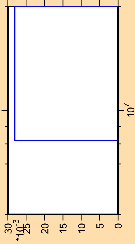
\Delta\sigma/\sigma vs. E for ^{145}\text{Ce}(n,\text{He}3)
