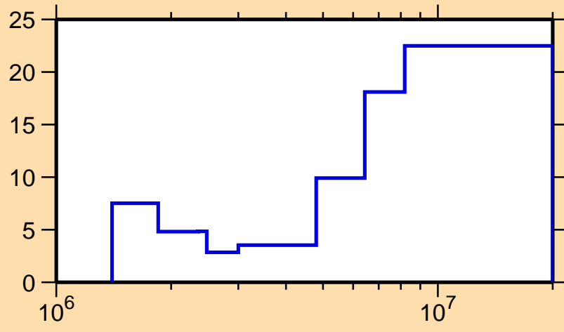
\Delta\sigma/\sigma vs. E for ^{145}\text{Ce}(n,\text{inel.})
