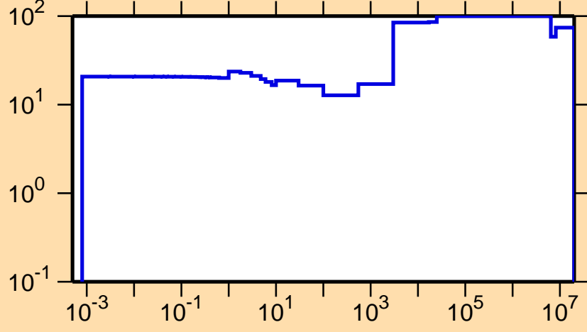
\Delta\sigma/\sigma vs. E for ^{145}\text{Ce}(n,\gamma)
