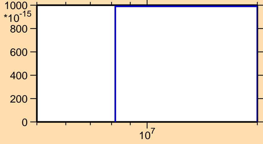
\sigma vs. E for ^{145}\text{Ce}(n,3n\alpha)
