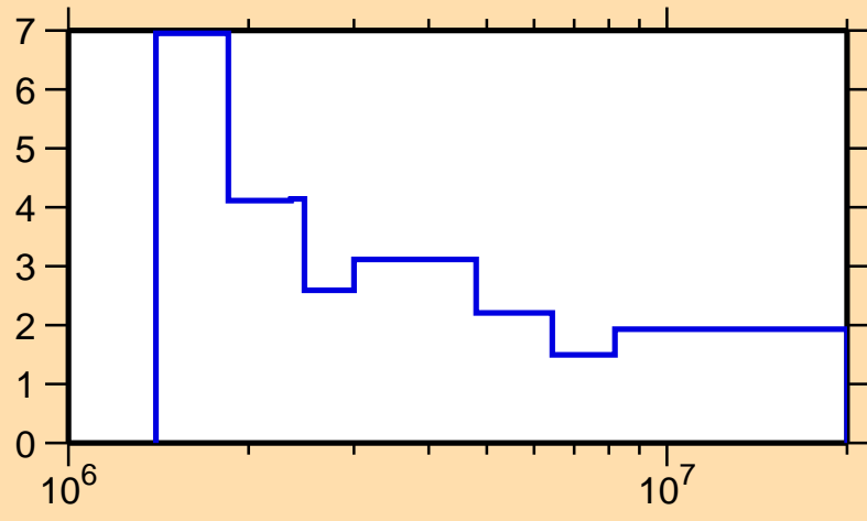
\Delta\sigma/\sigma vs. E for ^{145}\text{Ce}(n,\text{nonel.})
