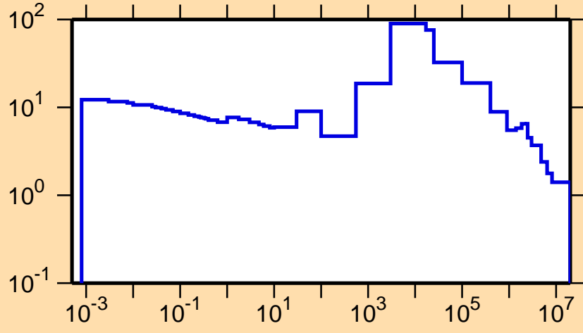
\Delta\sigma/\sigma vs. E for ^{145}\text{Ce}(n,\text{tot.})
