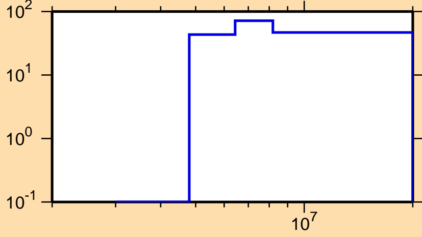
\Delta\sigma/\sigma vs. E for ^{145}\text{Ce}(n,p)
