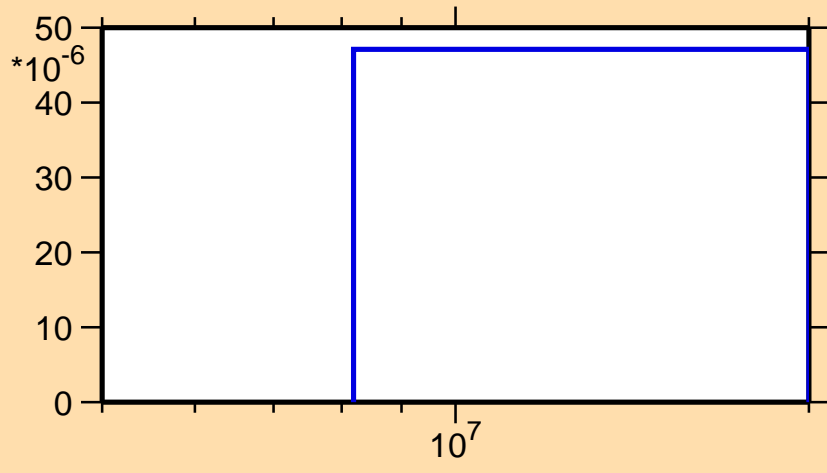
\sigma vs. E for ^{145}\text{Ce}(n,t)
