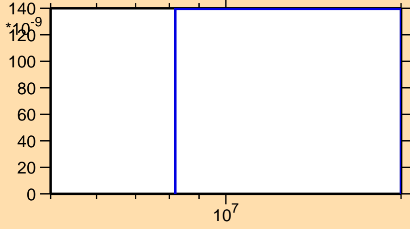
\sigma vs. E for ^{145}\text{Ce}(n,2n\alpha)
