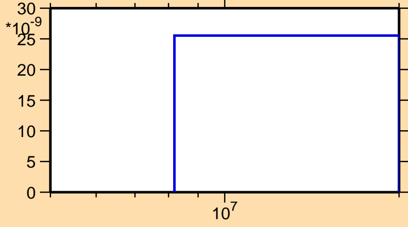
\sigma vs. E for ^{145}\text{Ce}(n,nt)
