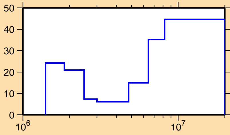
\Delta\sigma/\sigma vs. E for ^{145}\text{Ce}(n,n\text{cont.})
