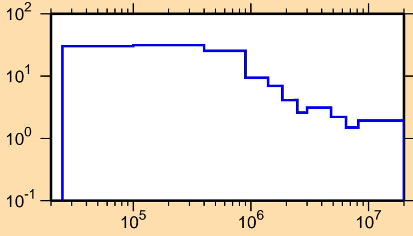
\Delta\sigma/\sigma vs. E for ^{145}\text{Ce}(n,\text{nonel.})
