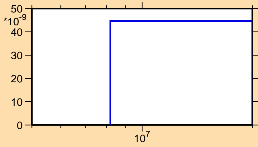
\sigma vs. E for ^{145}\text{Ce}(n,\text{nd})
