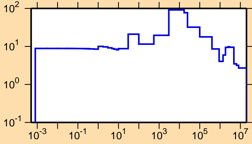
\Delta\sigma/\sigma vs. E for ^{145}\text{Ce}(n,\text{el.})
