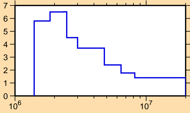
\Delta\sigma/\sigma vs. E for ^{145}\text{Ce}(n,\text{tot.})
