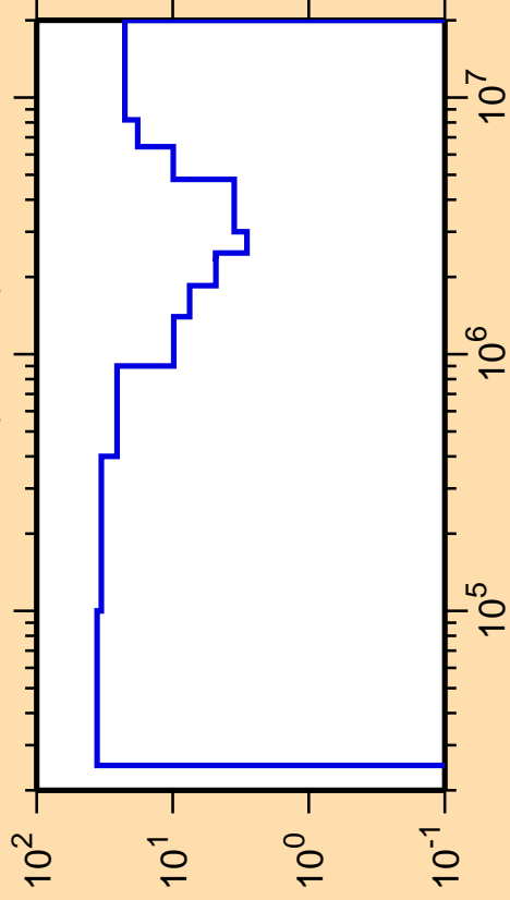
\Delta\sigma/\sigma vs. E for ^{145}\text{Ce}(n,\text{inel.})
