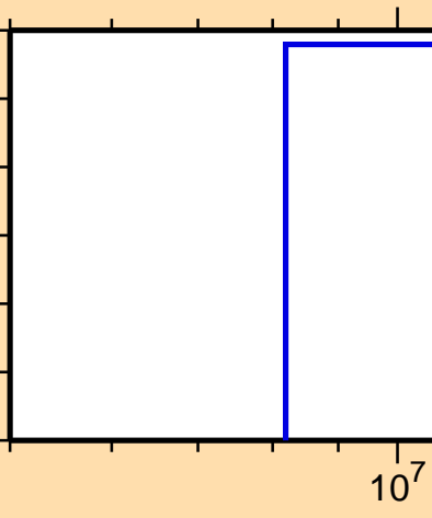
\sigma vs. E for ^{145}\text{Ce}(n,\text{He}3)
