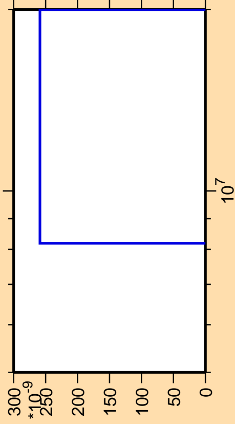
\Delta\sigma/\sigma vs. E for ^{145}\text{Ce}(\text{mt } 11)
