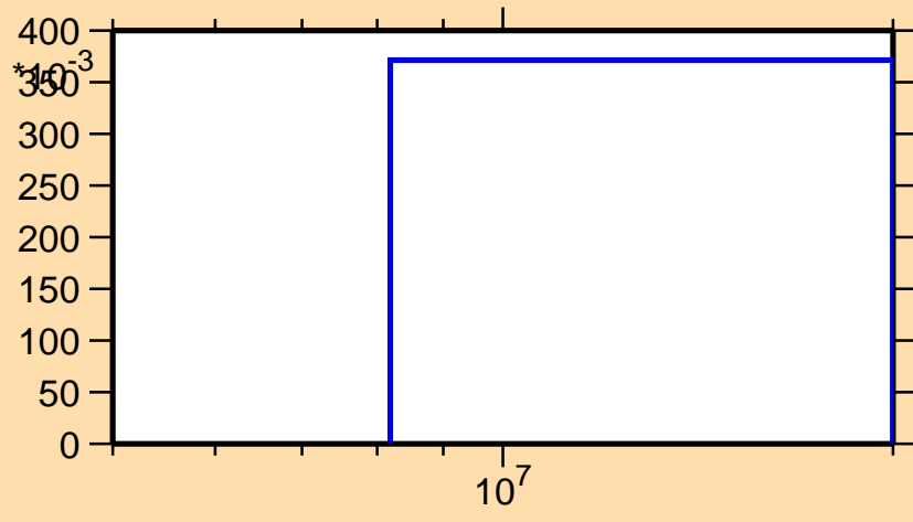
\sigma vs. E for ^{145}\text{Ce}(n,3n)
