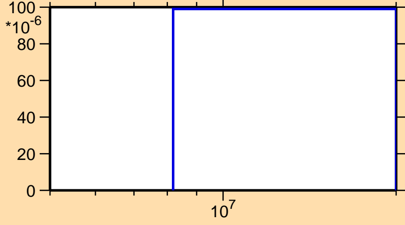
\sigma vs. E for ^{145}\text{Ce}(n,d)
