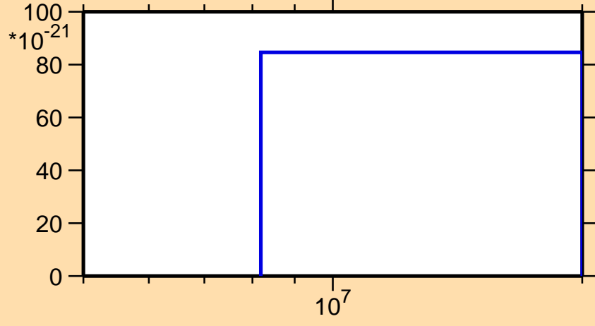
\sigma vs. E for ^{145}\text{Ce}(\text{mt } 11)
