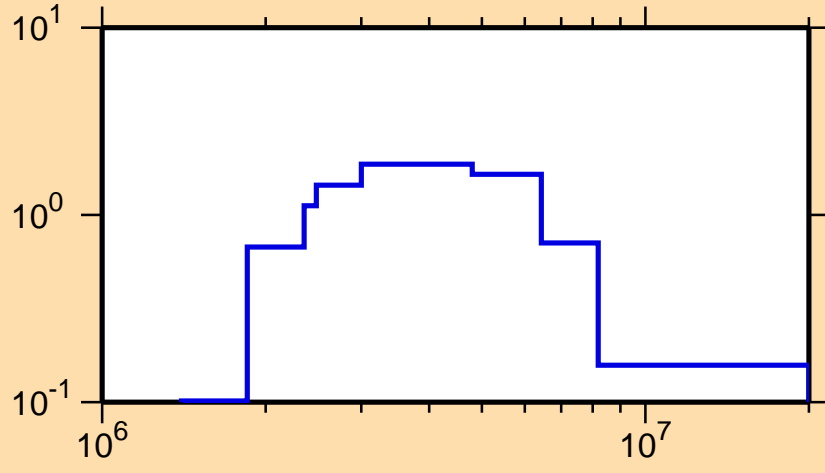
\sigma vs. E for ^{145}\text{Ce}(n,n\text{cont.})
