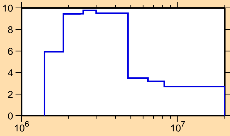
\Delta\sigma/\sigma vs. E for ^{145}\text{Ce}(n,\text{el.})
