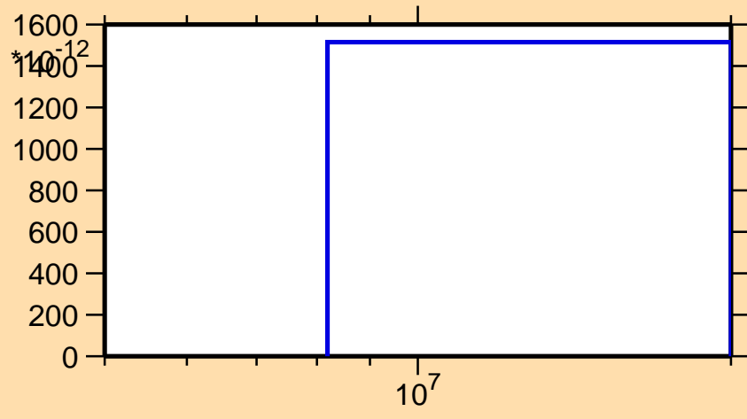
\sigma vs. E for ^{145}\text{Ce}(n,2np)
