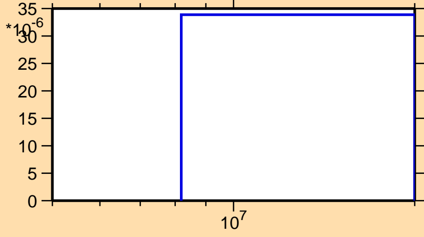
\sigma vs. E for ^{145}\text{Ce}(n,np)
