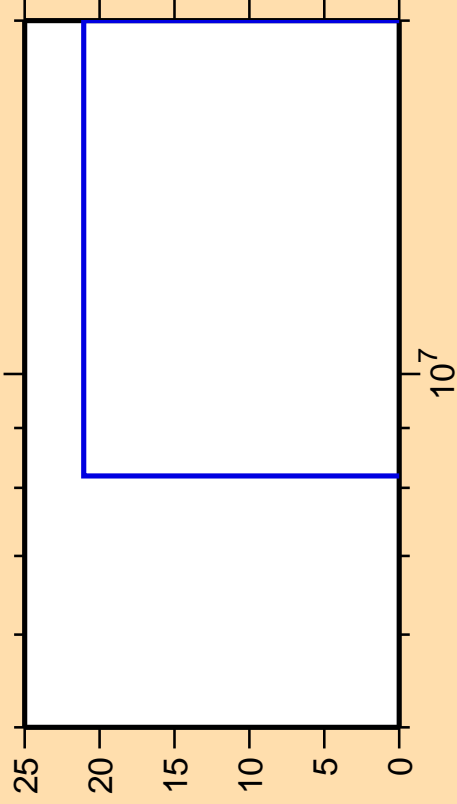
\Delta\sigma/\sigma vs. E for ^{145}\text{Ce}(n,3n)
