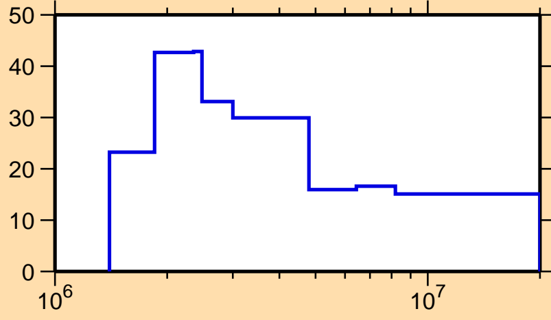
\Delta\sigma/\sigma vs. E for ^{145}\text{Ce}(n,n_1)
