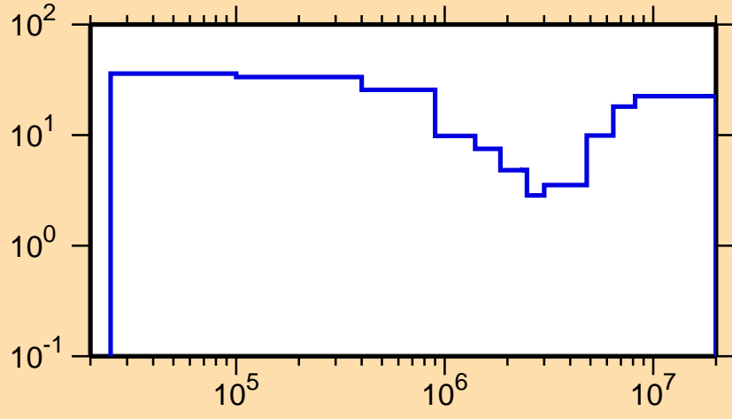
\Delta\sigma/\sigma vs. E for ^{145}\text{Ce}(n,\text{inel.})
