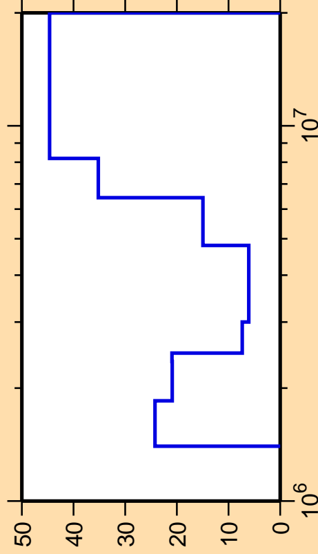
\Delta\sigma/\sigma vs. E for ^{145}\text{Ce}(n,n\text{cont.})
