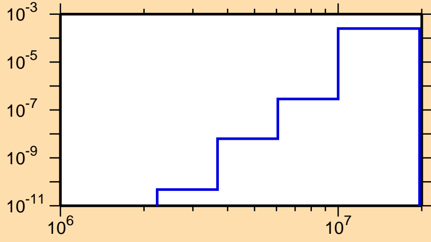
\sigma vs. E for ^{146}\text{Ce}(n,\alpha)
