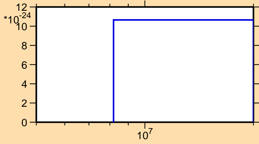
\sigma vs. E for ^{146}\text{Ce}(\text{mt 11})
