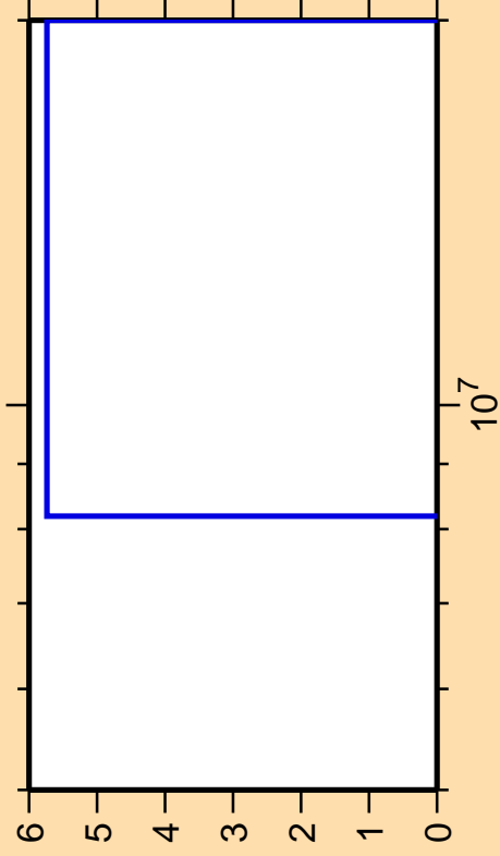
\Delta\sigma/\sigma vs. E for ^{146}\text{Ce}(n,2np)
