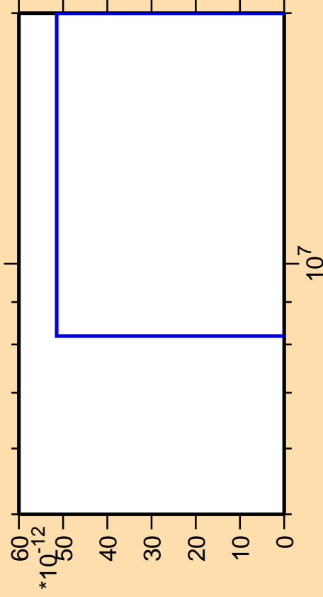
\Delta\sigma/\sigma vs. E for ^{146}\text{Ce}(\text{mt 11})
