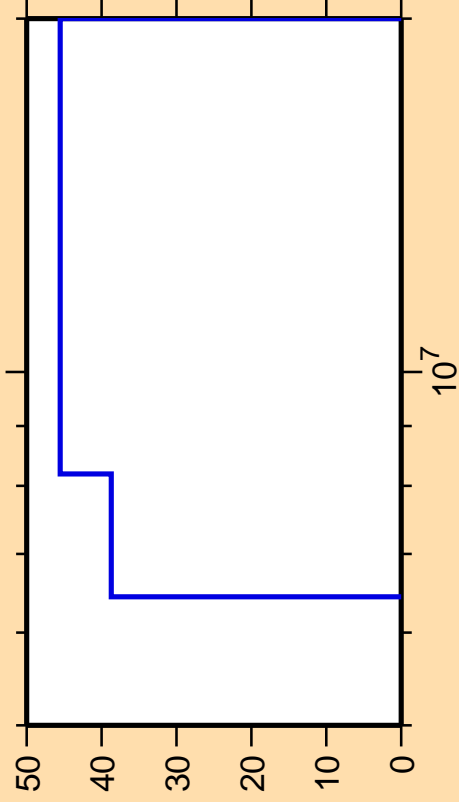
\Delta\sigma/\sigma vs. E for ^{147}\text{Ce}(n,n\alpha)
