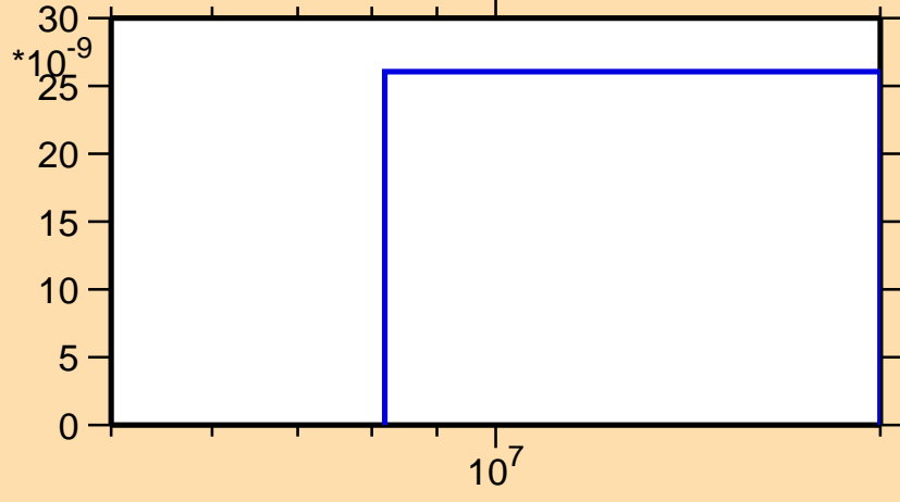
\sigma vs. E for ^{147}\text{Ce}(n,nt)
