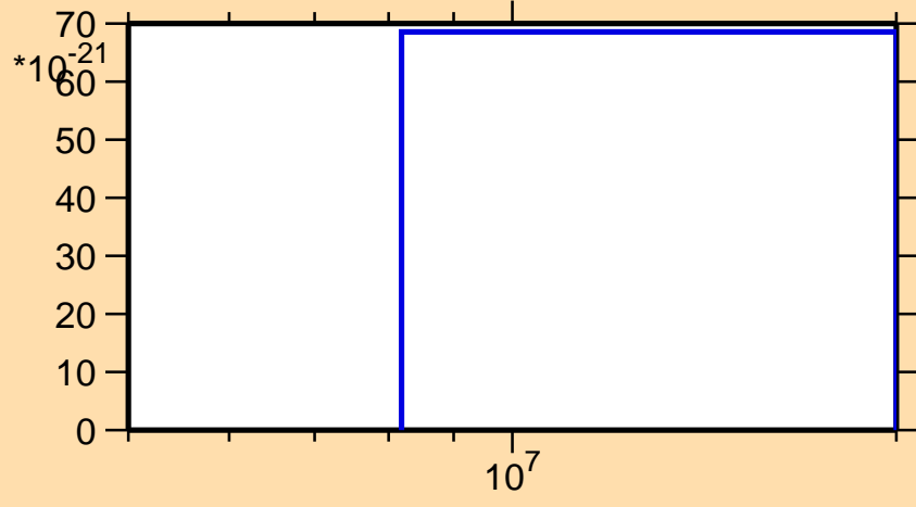
\sigma vs. E for ^{147}\text{Ce}(\text{mt } 11)
