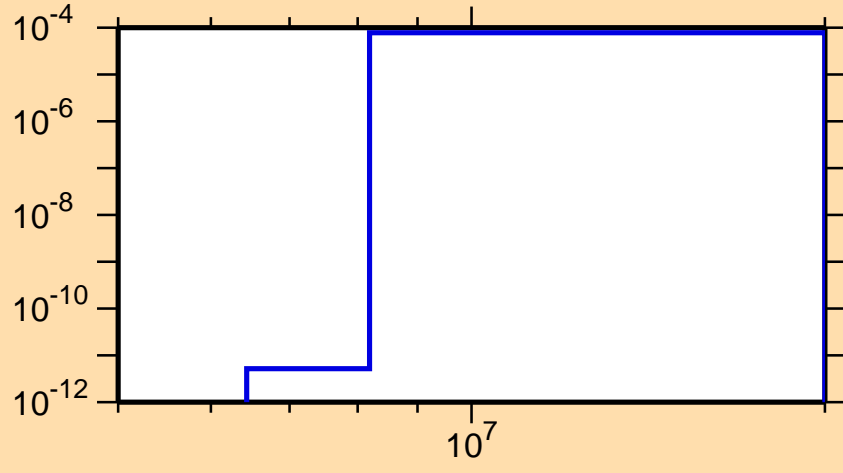
\sigma vs. E for ^{147}\text{Ce}(n,n\alpha)
