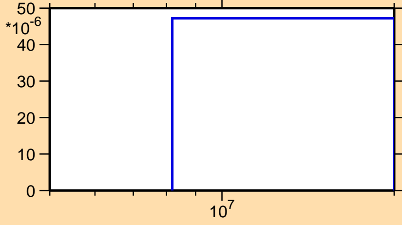
\sigma vs. E for ^{147}\text{Ce}(n,d)
