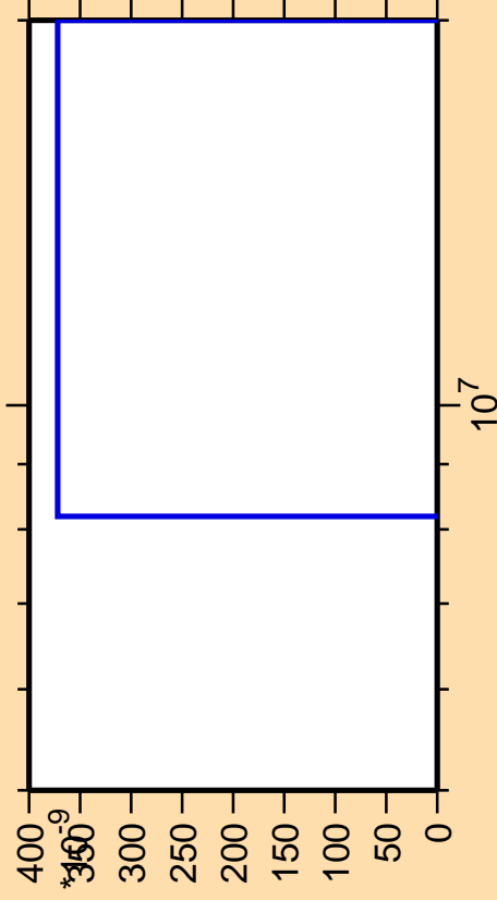
\Delta\sigma/\sigma vs. E for ^{147}\text{Ce}(\text{mt } 11)
