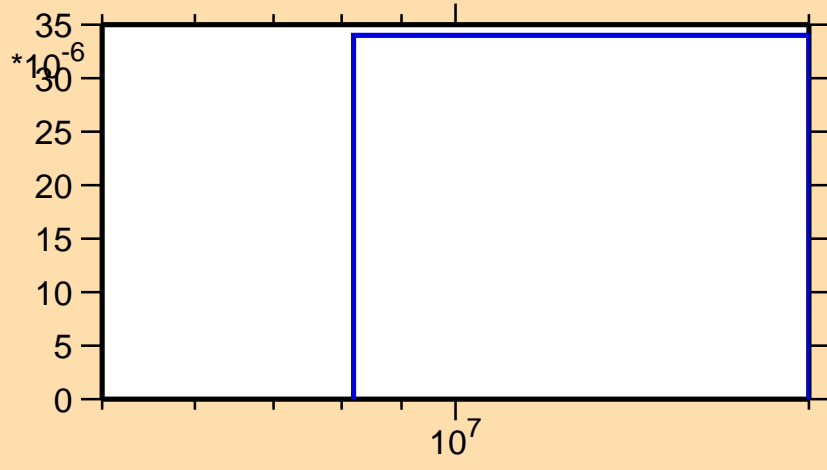
\sigma vs. E for ^{147}\text{Ce}(n,t)
