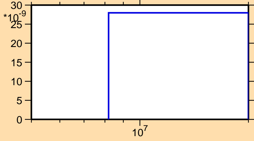
\sigma vs. E for ^{147}\text{Ce}(n,\text{nd})
