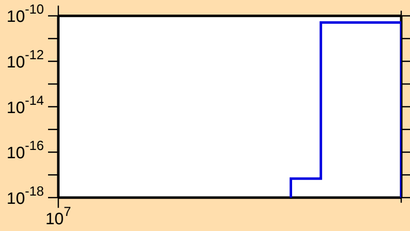
\sigma vs. E for ^{148}\text{Ce}(n,2np)
