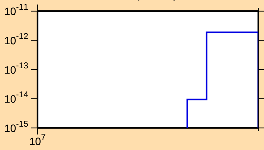
\sigma vs. E for ^{148}\text{Ce}(n,3n\alpha)
