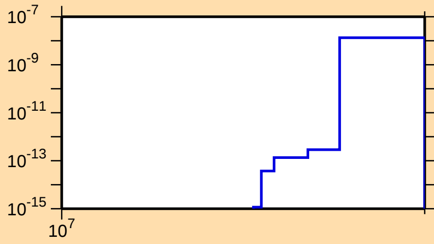
\sigma vs. E for ^{148}\text{Ce}(n,\text{nd})
