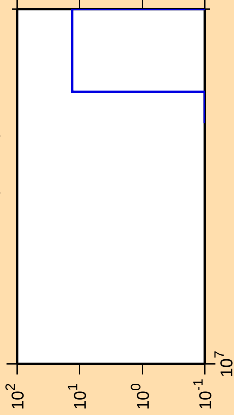
\Delta\sigma/\sigma vs. E for ^{148}\text{Ce}(n,3n\alpha)
