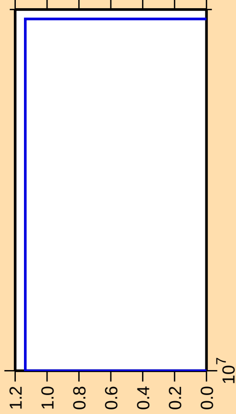
\Delta\sigma/\sigma vs. E for ^{148}\text{Ce}(n,2np)
