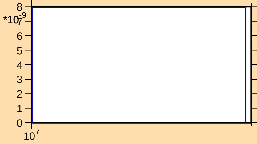
\sigma vs. E for ^{148}\text{Ce}(n,nt)
