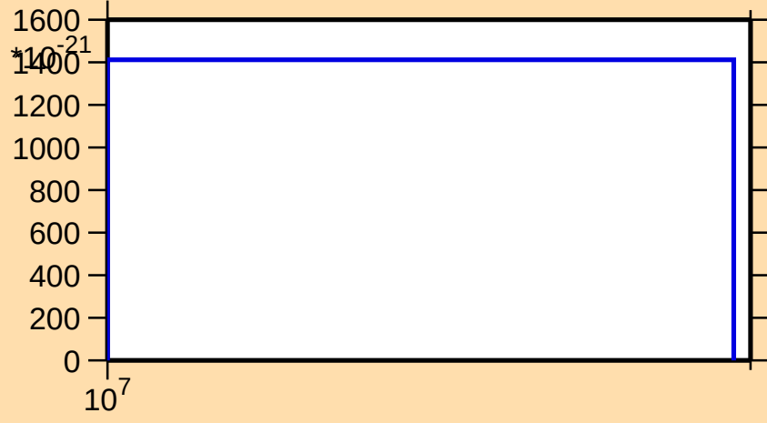
\sigma vs. E for ^{148}\text{Ce}(\text{mt 11})
