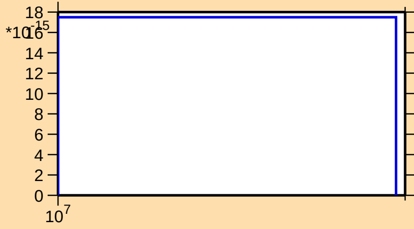
\sigma vs. E for ^{148}\text{Ce}(n,3n\alpha)
