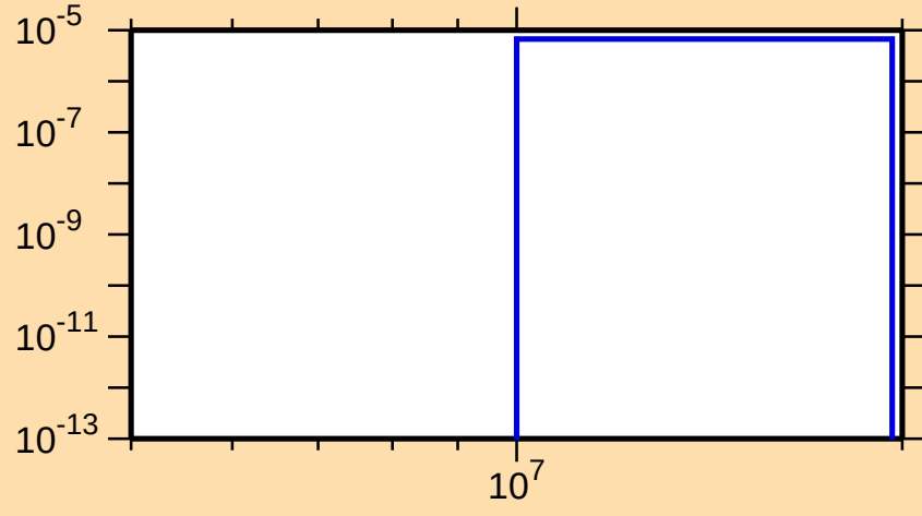
\sigma vs. E for ^{148}\text{Ce}(n,t)
