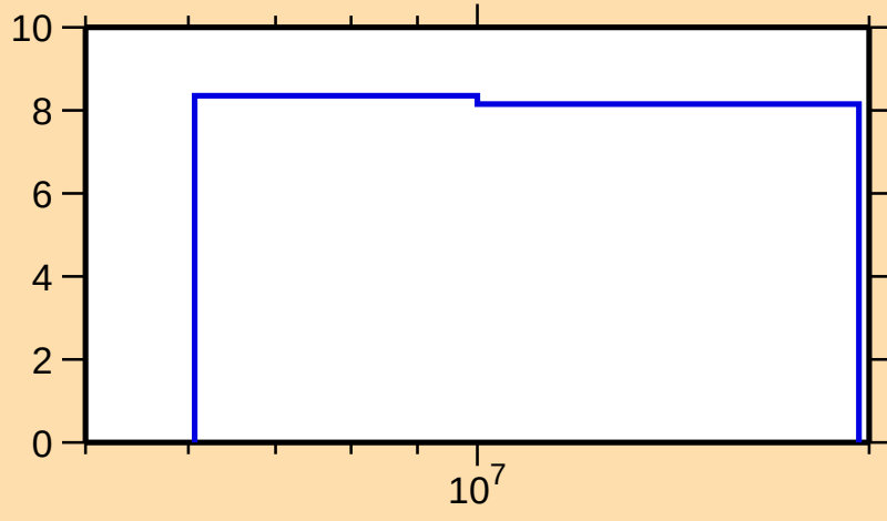
\Delta\sigma/\sigma vs. E for ^{148}\text{Ce}(n,\text{nonel.})
