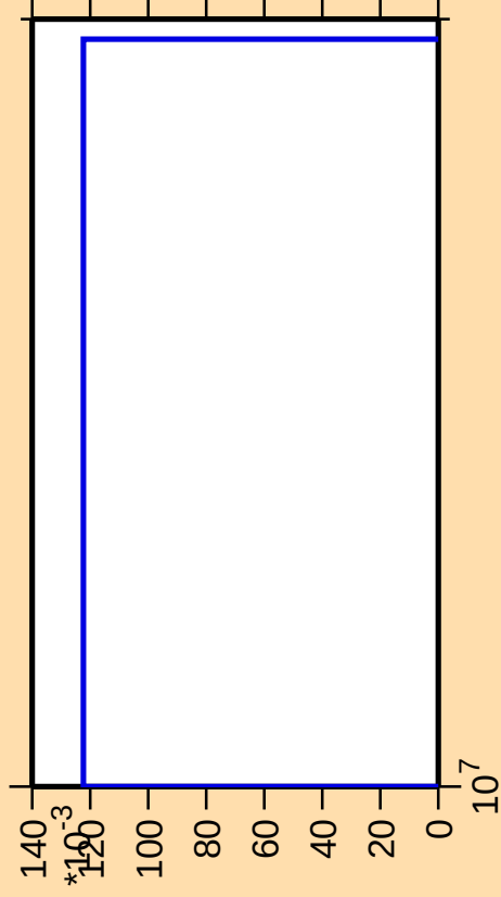
\Delta\sigma/\sigma vs. E for ^{148}\text{Ce}(n,3n\alpha)
