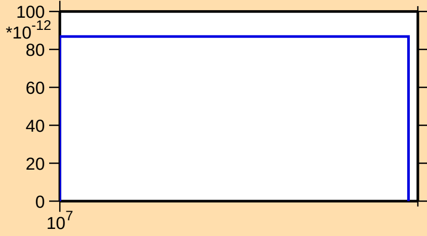
\sigma vs. E for ^{148}\text{Ce}(n,\text{nd})
