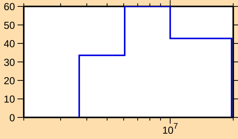
\Delta\sigma/\sigma vs. E for ^{148}\text{Ce}(n,n\text{cont.})
