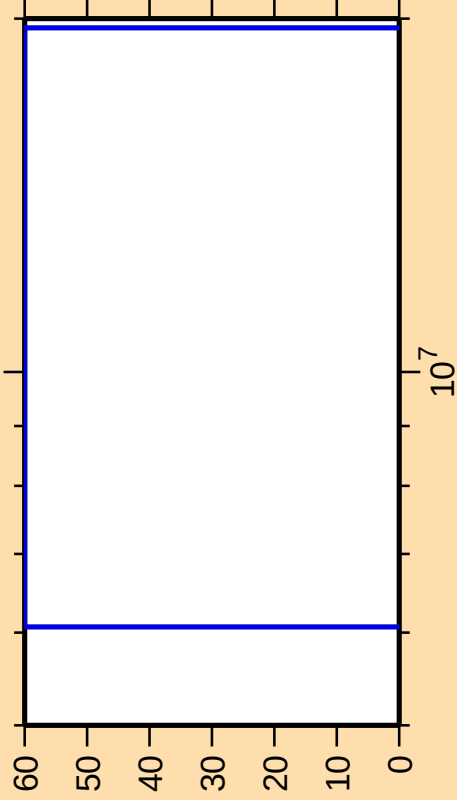
\Delta\sigma/\sigma vs. E for ^{148}\text{Ce}(n,n\alpha)
