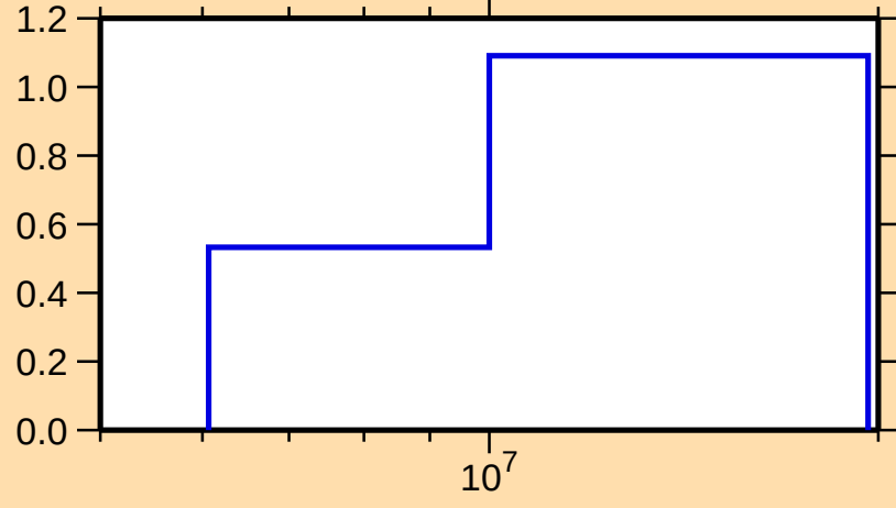
\sigma vs. E for ^{148}\text{Ce}(n,2n)
