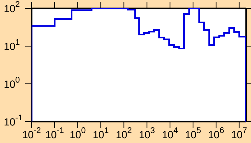
\Delta\sigma/\sigma vs. E for ^{148}\text{Ce}(n,\text{tot.})
