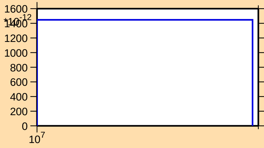
\sigma vs. E for ^{148}\text{Ce}(n,2n\alpha)
