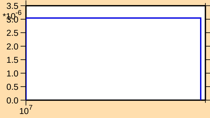
\sigma vs. E for ^{148}\text{Ce}(n,np)
