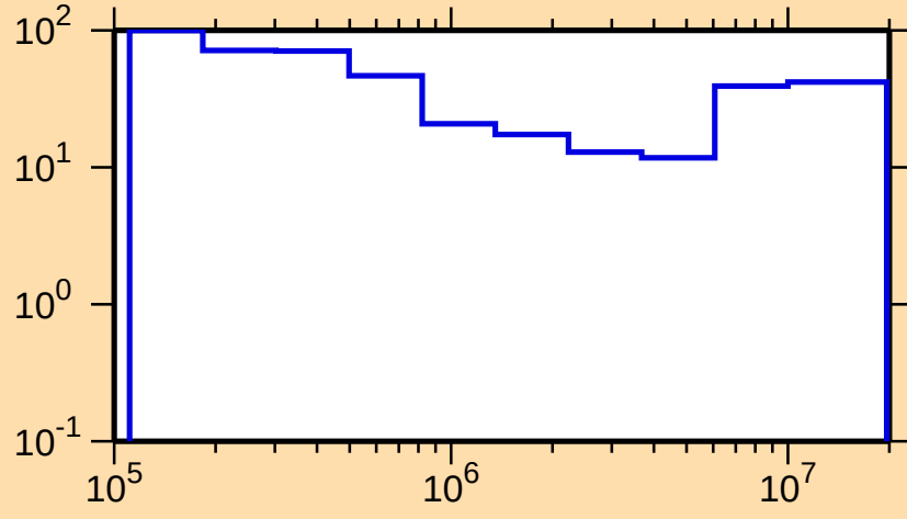
\Delta\sigma/\sigma vs. E for ^{148}\text{Ce}(n,\text{inel.})
