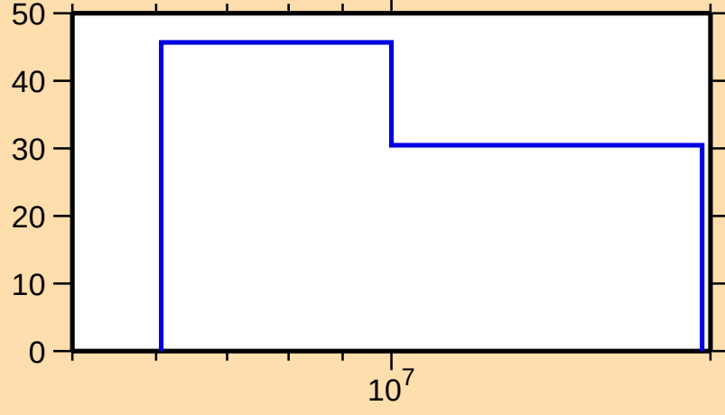
\Delta\sigma/\sigma vs. E for ^{148}\text{Ce}(n,\text{el.})
