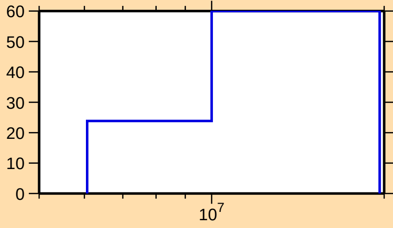
\Delta\sigma/\sigma vs. E for ^{148}\text{Ce}(n,2n)
