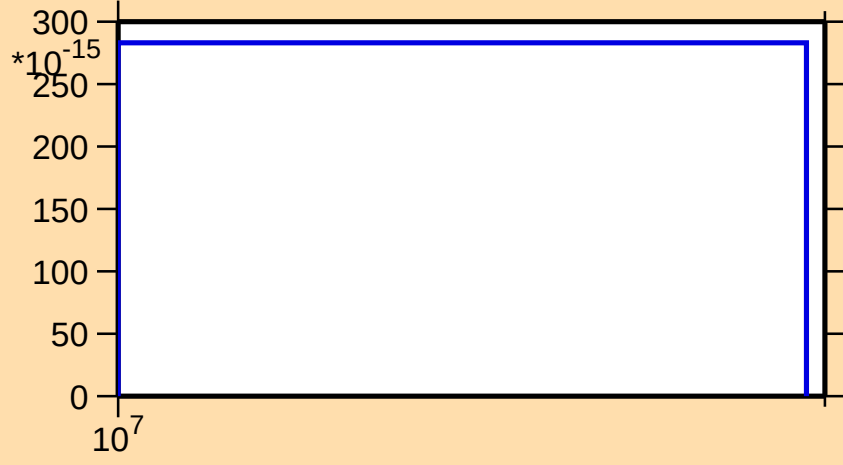
\sigma vs. E for ^{148}\text{Ce}(n,2np)
