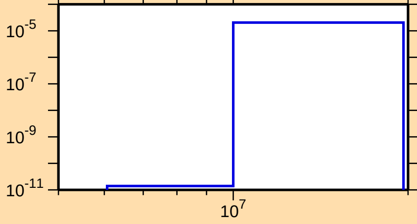
\sigma vs. E for ^{148}\text{Ce}(n,n\alpha)
