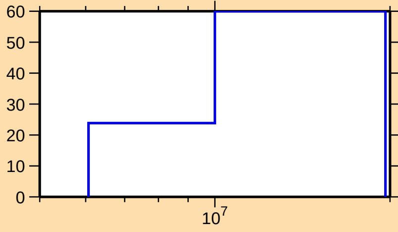
\Delta\sigma/\sigma vs. E for ^{148}\text{Ce}(n,2n)
