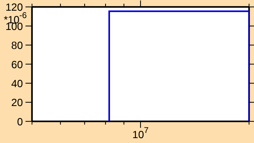
\sigma vs. E for ^{148}\text{Ce}(n,p)
