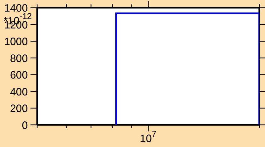
\sigma vs. E for ^{148}\text{Ce}(n,2n\alpha)
