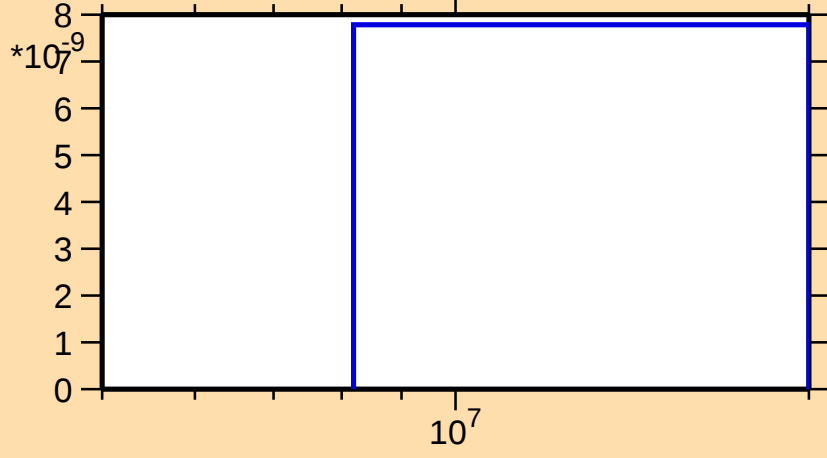
\sigma vs. E for ^{148}\text{Ce}(n,nt)
