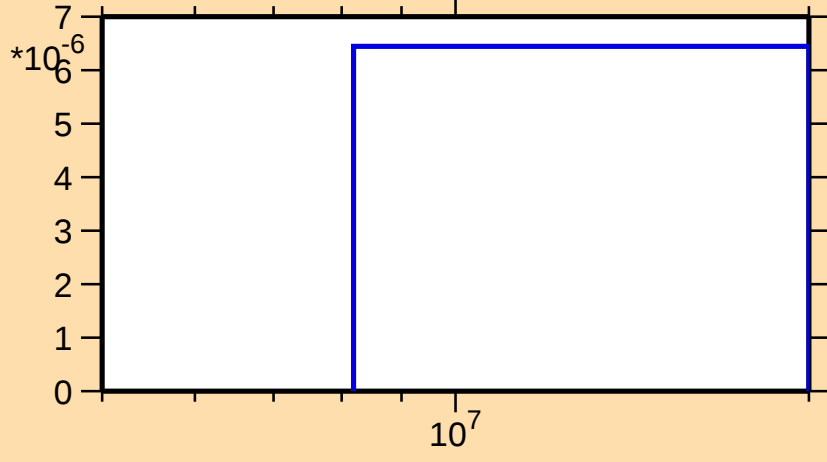
\sigma vs. E for ^{148}\text{Ce}(n,d)
