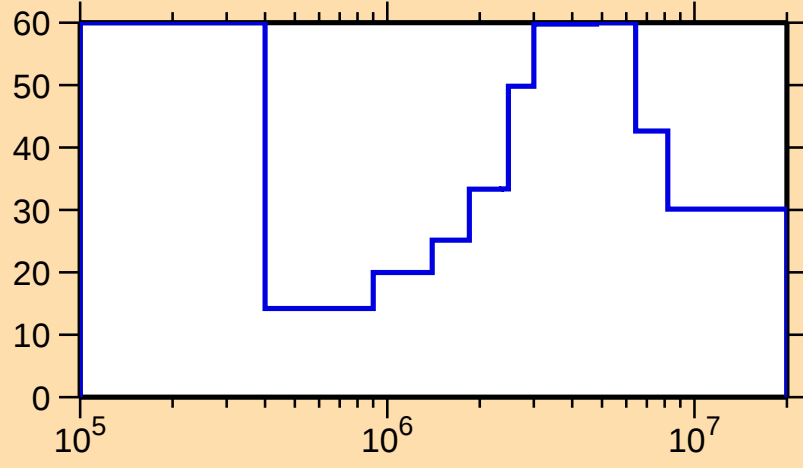
\Delta\sigma/\sigma vs. E for ^{148}\text{Ce}(n,\text{el.})
