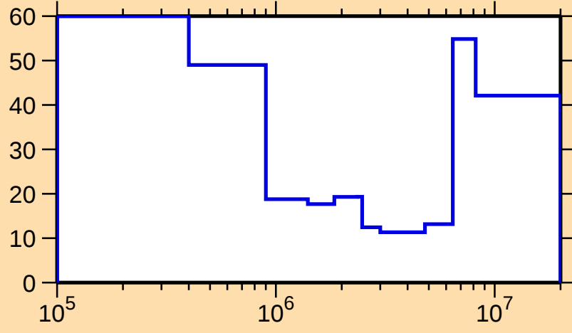
\Delta\sigma/\sigma vs. E for ^{148}\text{Ce}(n,\text{inel.})
