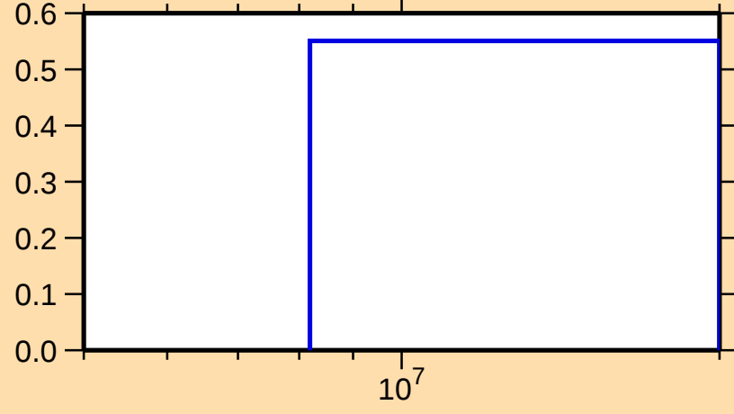
\sigma vs. E for ^{148}\text{Ce}(n,3n)
