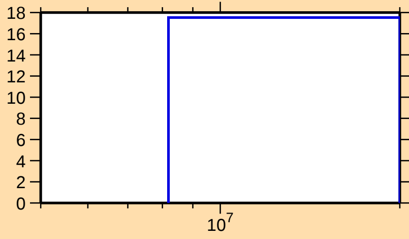
\Delta\sigma/\sigma vs. E for ^{148}\text{Ce}(n,\text{tot.})
