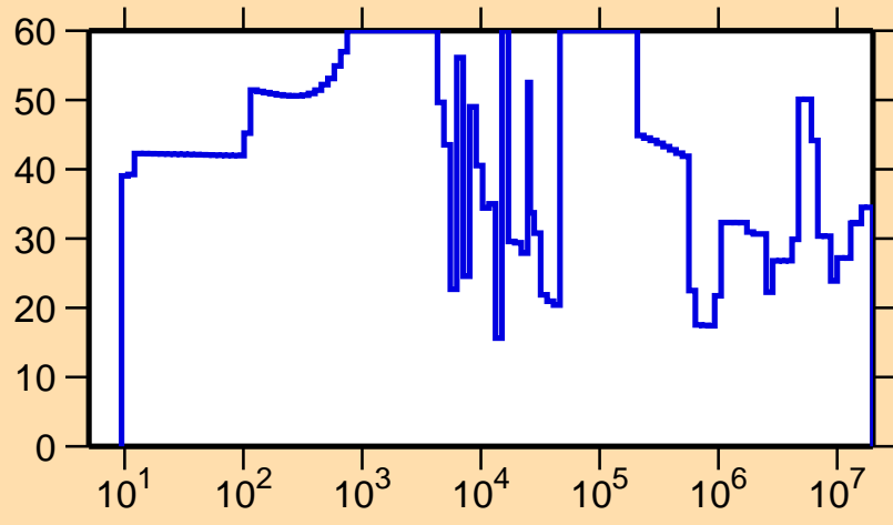
\Delta\sigma/\sigma vs. E for ^{150}\text{Ce}(n,\text{el.})
