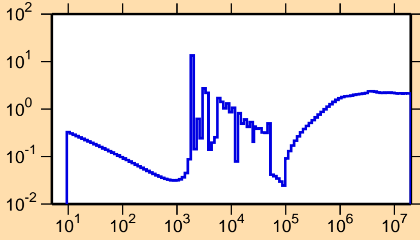
\sigma vs. E for ^{150}\text{Ce}(n,\text{nonel.})
