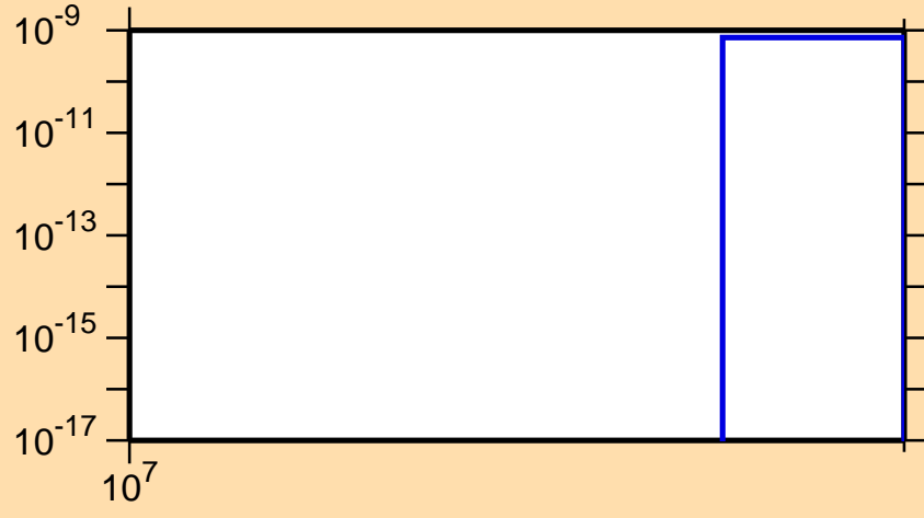
\sigma vs. E for ^{150}\text{Ce}(n,\text{nd})
