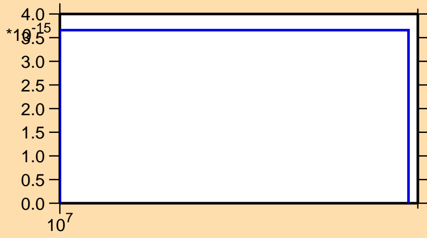
\sigma vs. E for ^{150}\text{Ce}(n,2np)
