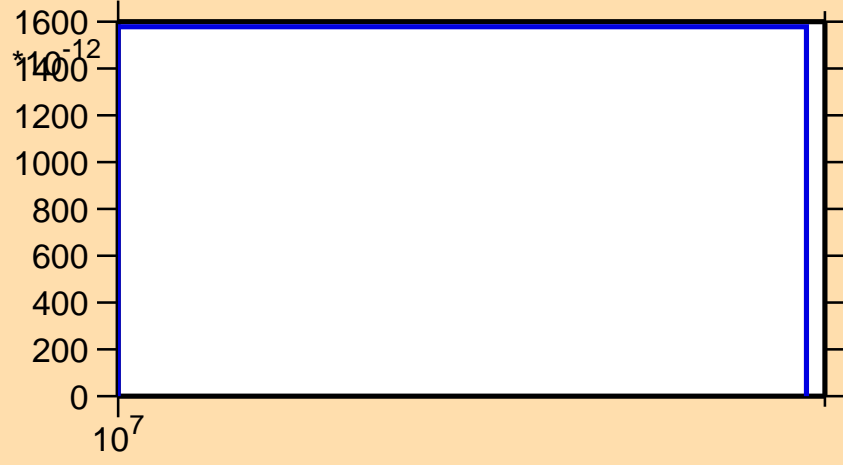
\sigma vs. E for ^{150}\text{Ce}(n,nt)
