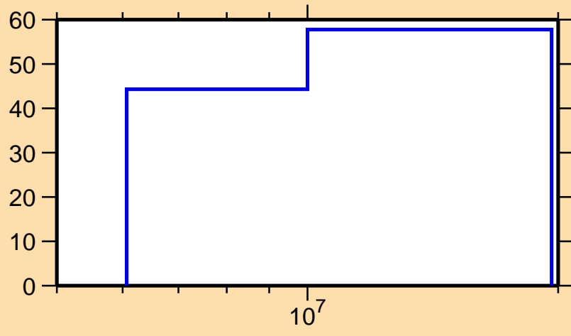
\Delta\sigma/\sigma vs. E for ^{150}\text{Ce}(n,2n)
