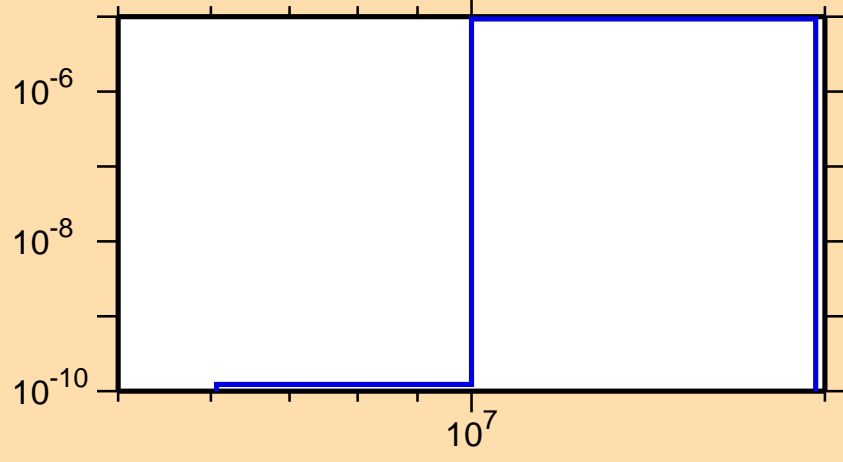
\sigma vs. E for ^{150}\text{Ce}(n,\alpha)
