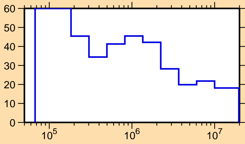
\Delta\sigma/\sigma vs. E for ^{150}\text{Ce}(n,\text{nonel.})
