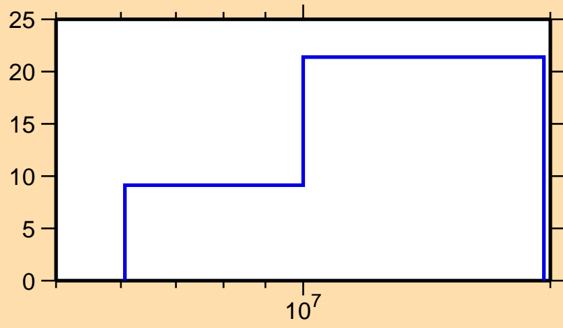
\Delta\sigma/\sigma vs. E for ^{150}\text{Ce}(n,\text{tot.})
