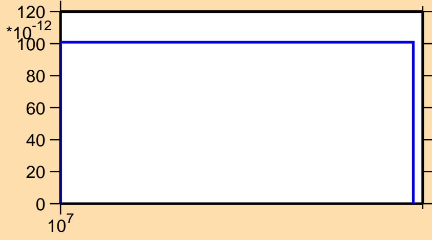
\sigma vs. E for ^{150}\text{Ce}(n,2n\alpha)
