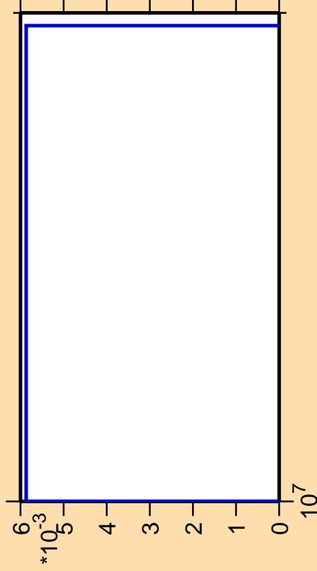
\Delta\sigma/\sigma vs. E for ^{150}\text{Ce}(n,2np)
