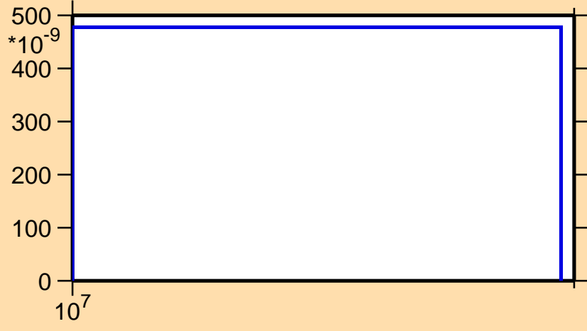
\sigma vs. E for ^{150}\text{Ce}(n,np)
