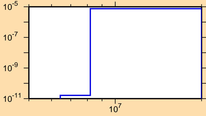
\sigma vs. E for ^{150}\text{Ce}(n,\alpha)
