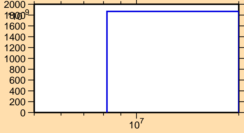
\sigma vs. E for ^{150}\text{Ce}(n,n\alpha)
