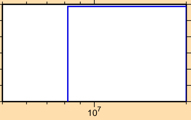
\sigma vs. E for ^{150}\text{Ce}(n,\text{nd})
