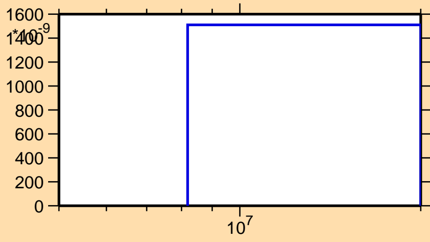
\sigma vs. E for ^{150}\text{Ce}(n,t)
