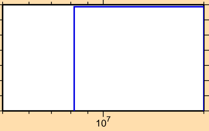
\sigma vs. E for ^{150}\text{Ce}(n,d)
