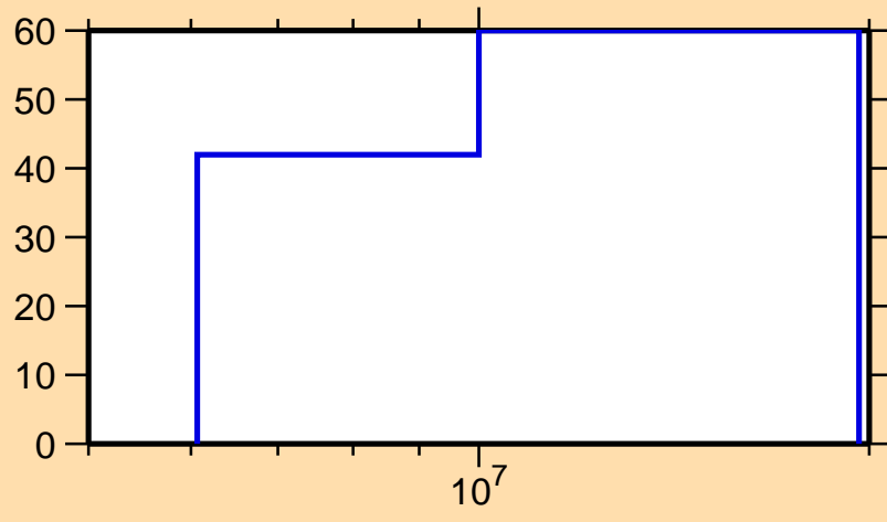
\Delta\sigma/\sigma vs. E for ^{151}\text{Ce}(n,p)
