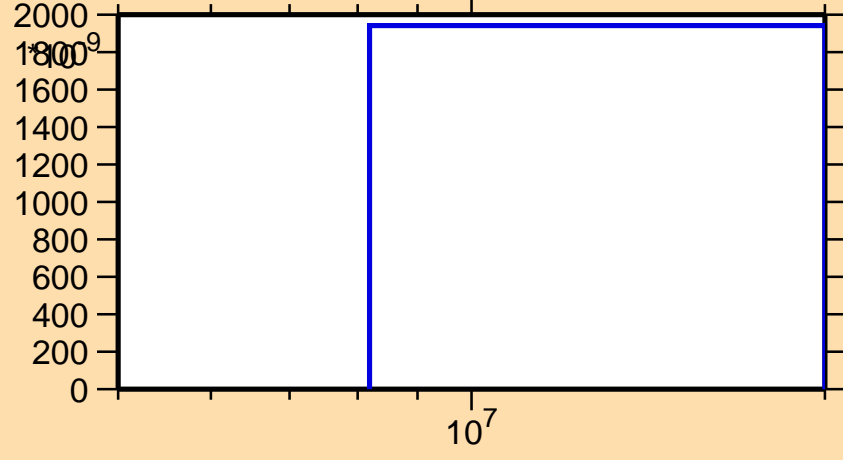
\sigma vs. E for ^{151}\text{Ce}(n,t)
