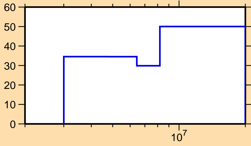
\Delta\sigma/\sigma vs. E for ^{151}\text{Ce}(n,2n)
