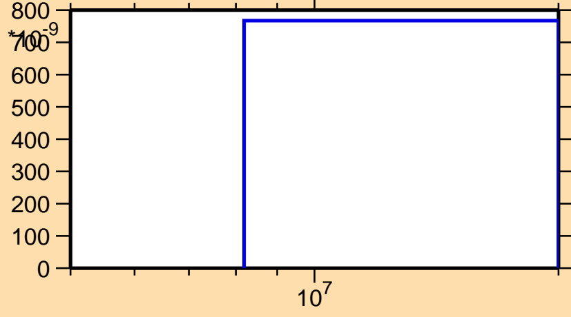
\sigma vs. E for ^{151}\text{Ce}(n,d)
