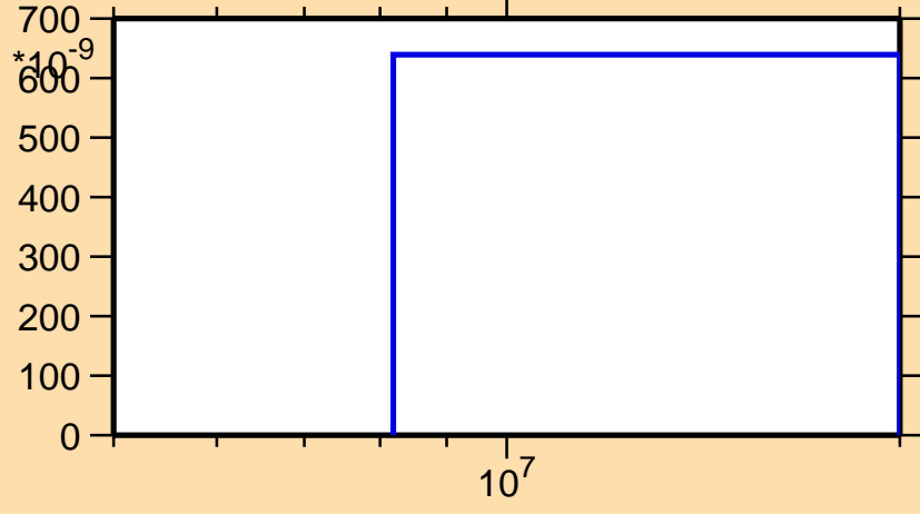
\sigma vs. E for ^{151}\text{Ce}(n,n\alpha)
