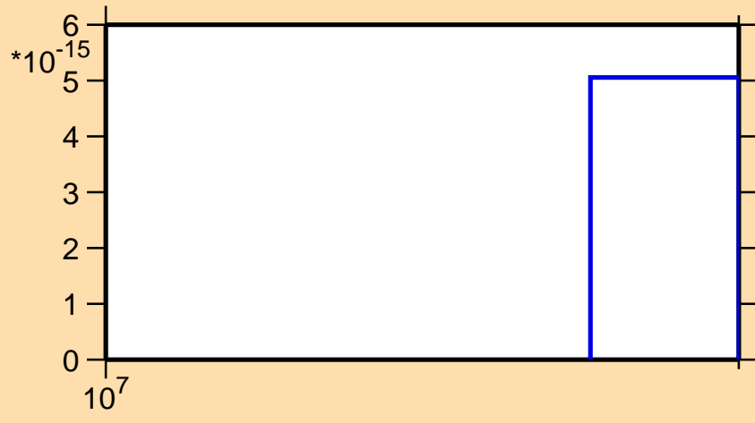
\sigma vs. E for ^{152}\text{Ce}(n,2np)
