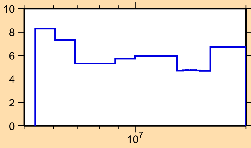
\Delta\sigma/\sigma vs. E for ^{152}\text{Ce}(n,\text{nonel.})
