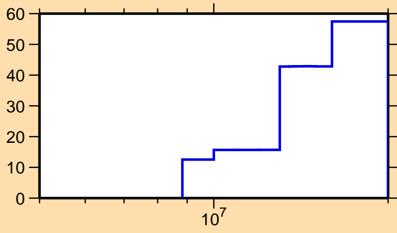
\Delta\sigma/\sigma vs. E for ^{152}\text{Ce}(n,2n)
