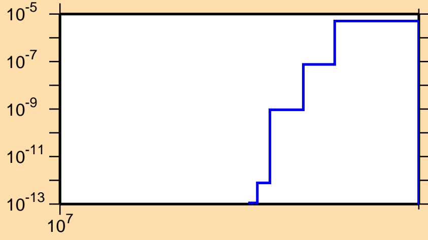
\sigma vs. E for ^{152}\text{Ce}(n,np)
