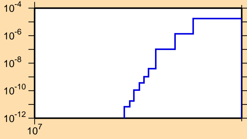
\sigma vs. E for ^{152}\text{Ce}(n,d)
