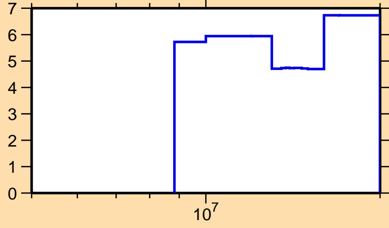
\Delta\sigma/\sigma vs. E for ^{152}\text{Ce}(n,\text{nonel.})
