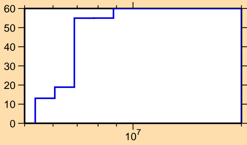
\Delta\sigma/\sigma vs. E for ^{152}\text{Ce}(n,\text{inel.})
