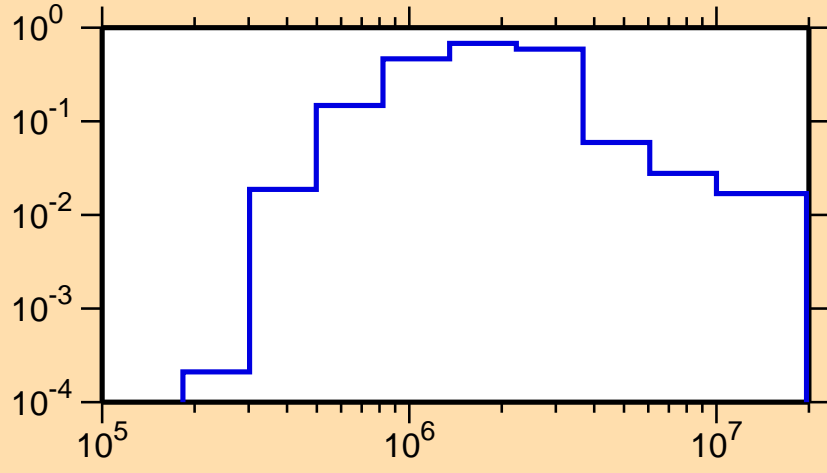
\sigma vs. E for ^{152}\text{Ce}(n,n_2)
