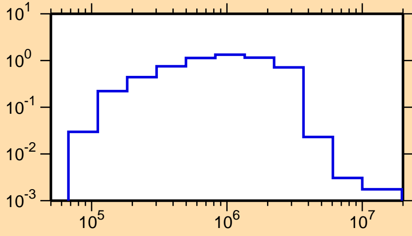
\sigma vs. E for ^{152}\text{Ce}(n,n_1)
