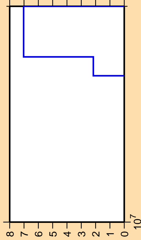
\Delta\sigma/\sigma vs. E for ^{239}\text{Cf} (mt 45)
