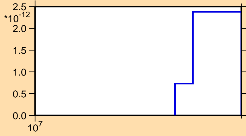
\sigma vs. E for ^{239}\text{Cf} (mt 45)
