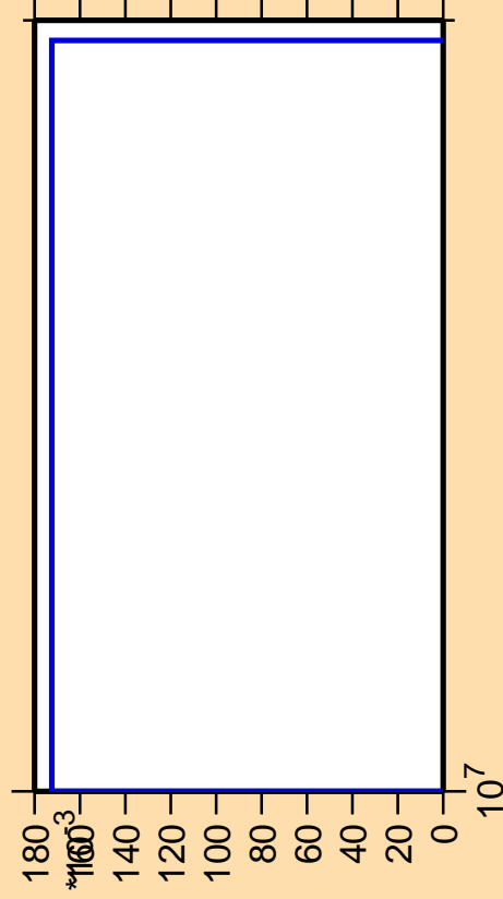
\Delta\sigma/\sigma vs. E for ^{239}\text{Cf} (mt 45)
