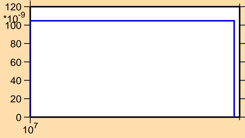
\sigma vs. E for ^{239}\text{Cf}(n,3n)
