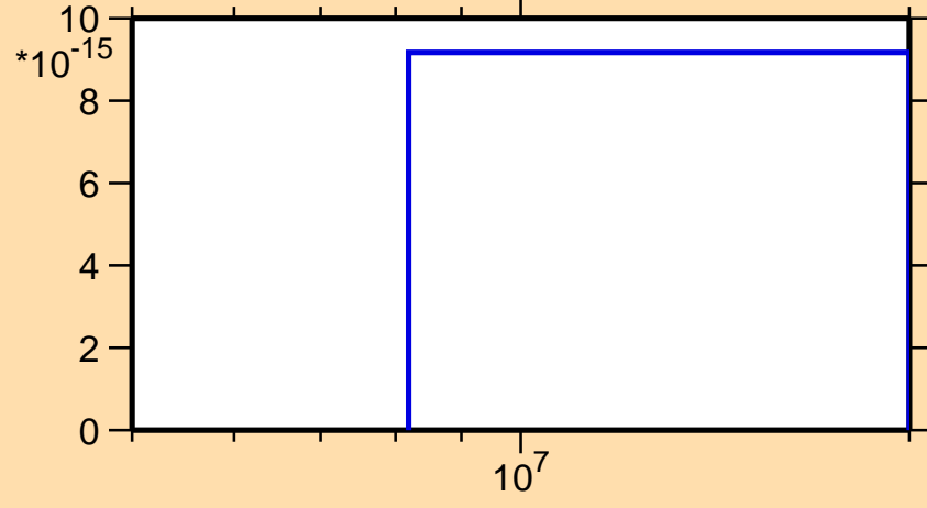
\sigma vs. E for ^{239}\text{Cf}(\text{mt } 34)
