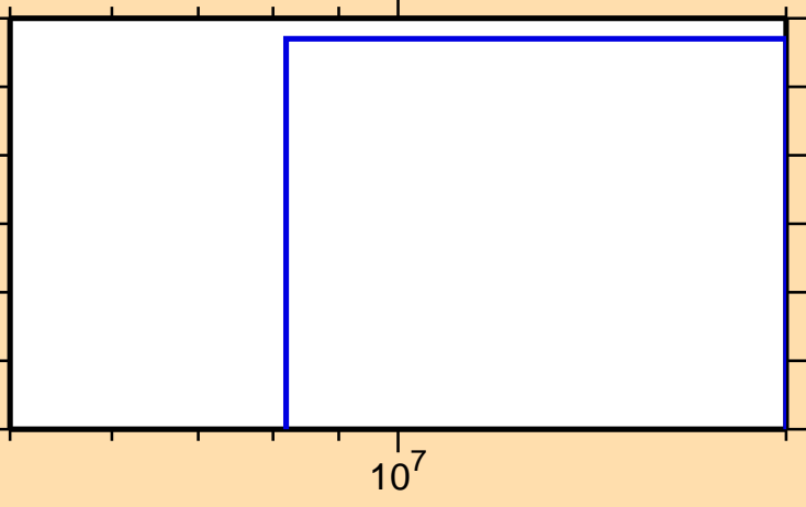
\sigma vs. E for ^{239}\text{Cf}(\text{mt117})
