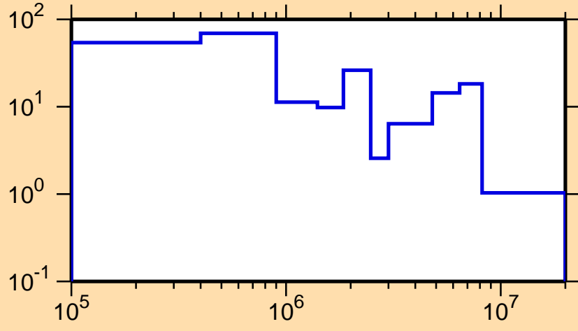
\Delta\sigma/\sigma vs. E for ^{239}\text{Cf}(n,\text{tot.})
