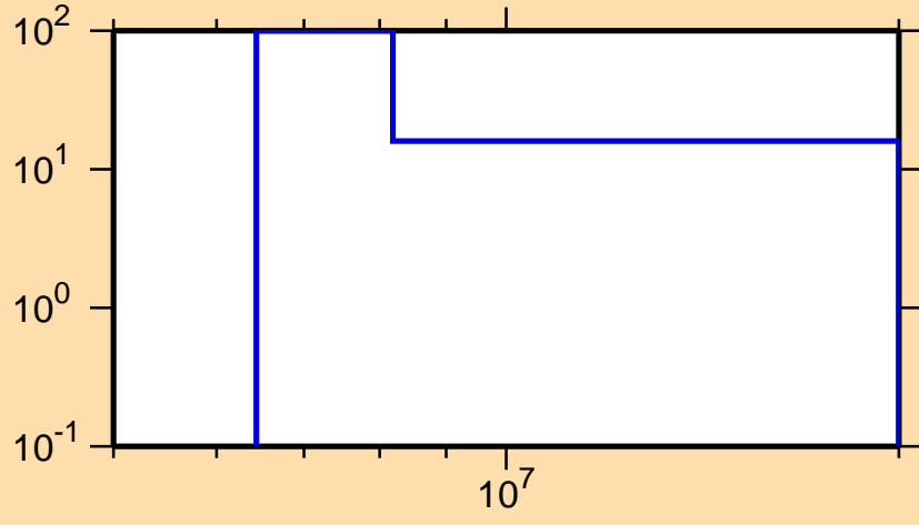
\Delta\sigma/\sigma vs. E for ^{239}\text{Cf}(n,2n)
