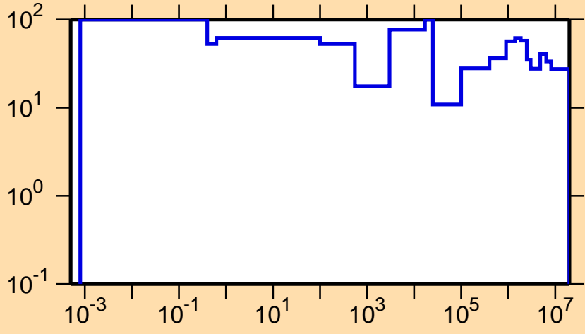
\Delta\sigma/\sigma vs. E for ^{239}\text{Cf}(n,f)
