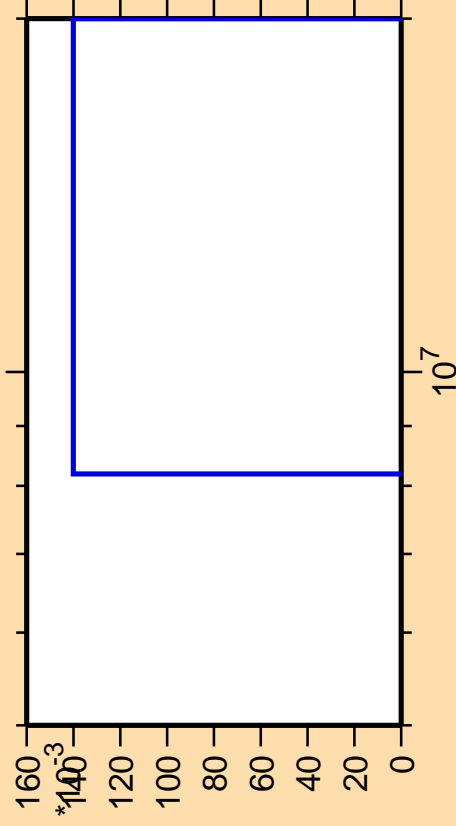
\Delta\sigma/\sigma vs. E for ^{239}\text{Cf}(\text{mt } 45)
