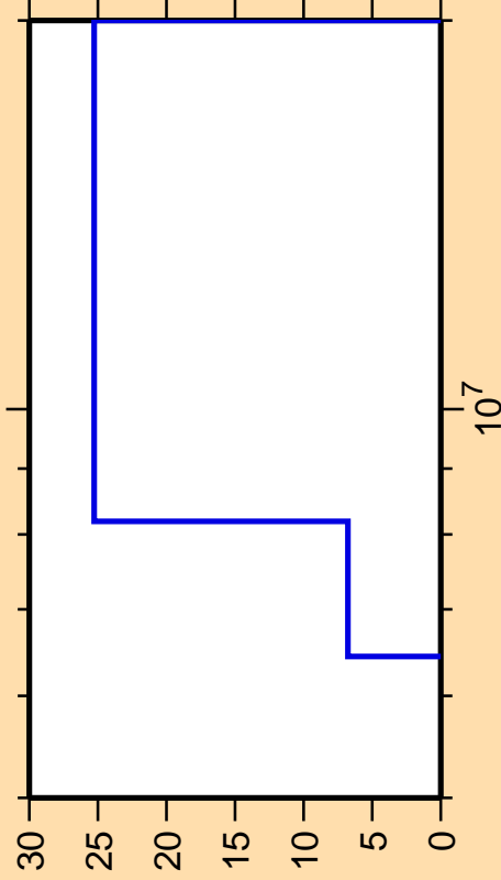
\Delta\sigma/\sigma vs. E for ^{239}\text{Cf}(n,p\alpha)
