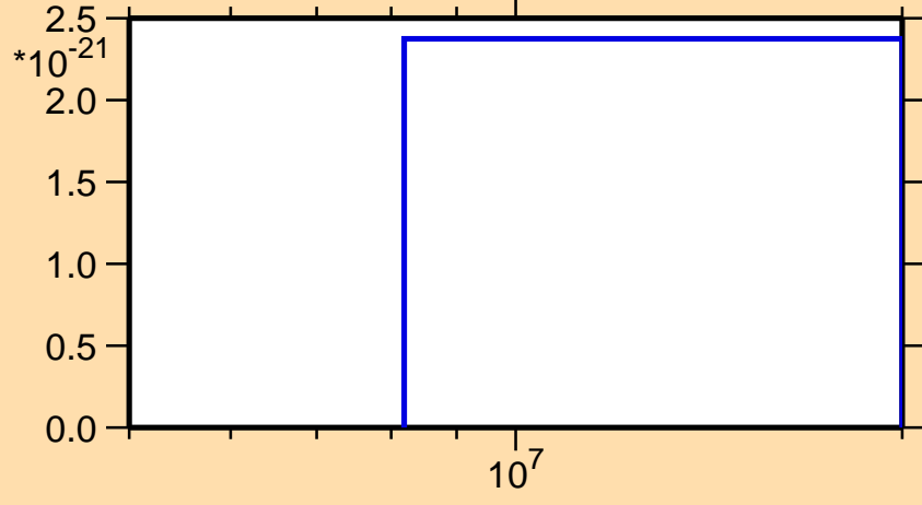
\sigma vs. E for ^{239}\text{Cf}(\text{mt } 42)
