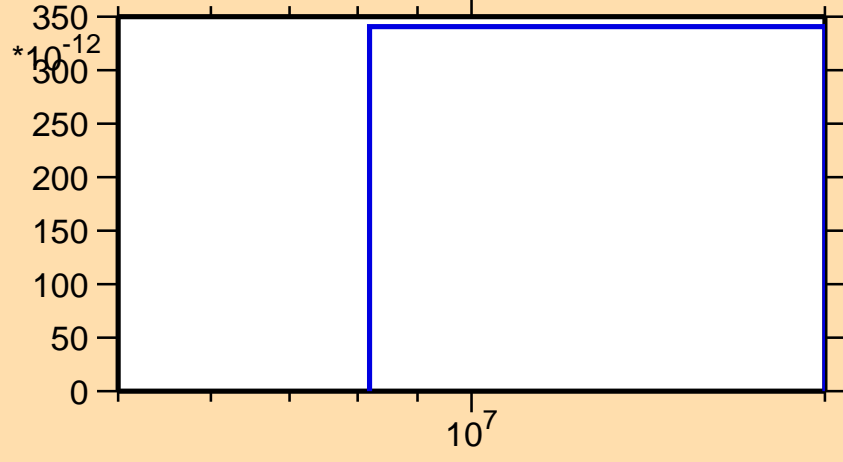
\sigma vs. E for ^{239}\text{Cf}(n,2np)
