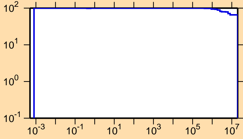
\Delta\sigma/\sigma vs. E for ^{239}\text{Cf}(n,\gamma)
