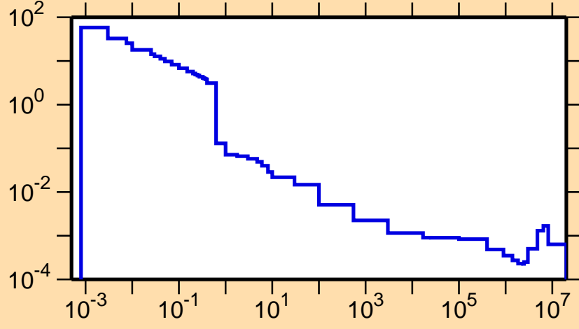
\sigma vs. E for ^{239}\text{Cf}(n,\gamma)
