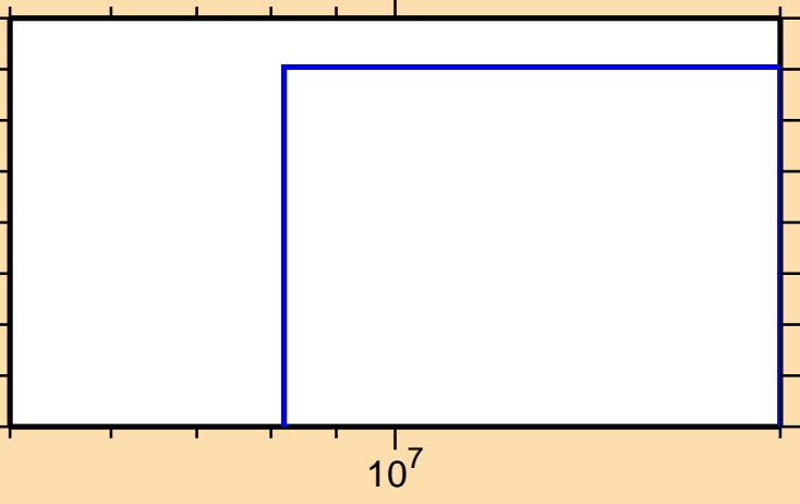
\sigma vs. E for ^{239}\text{Cf}(n,\text{He3})
