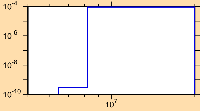
\sigma vs. E for ^{239}\text{Cf}(n,np)
