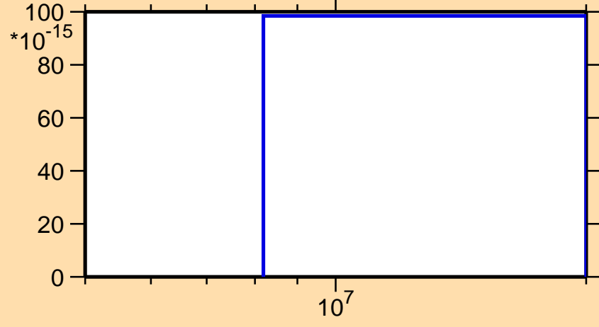
\sigma vs. E for ^{239}\text{Cf}(\text{mt } 45)
