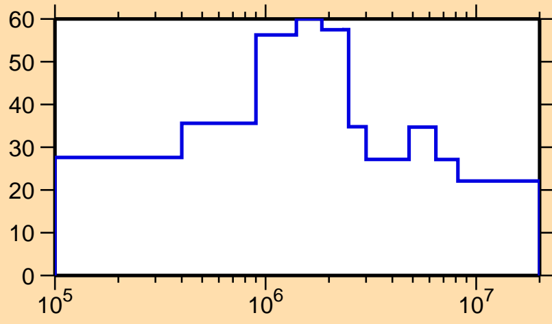
\Delta\sigma/\sigma vs. E for ^{239}\text{Cf}(n,\text{nonel.})
