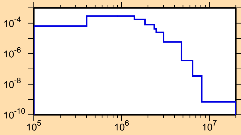
\sigma vs. E for ^{239}\text{Cf}(n,n_1)
