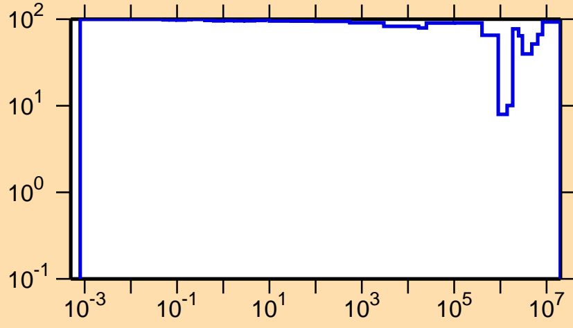
\Delta\sigma/\sigma vs. E for ^{239}\text{Cf}(n,p)
