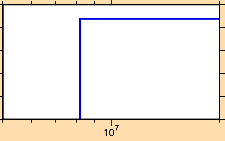
\sigma vs. E for ^{239}\text{Cf}(n,3n)
