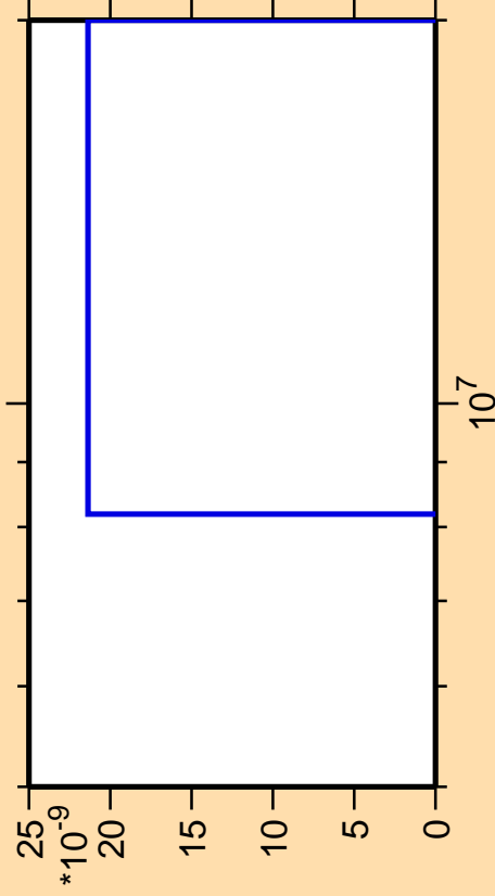
\Delta\sigma/\sigma vs. E for ^{239}\text{Cf}(\text{mt } 42)
