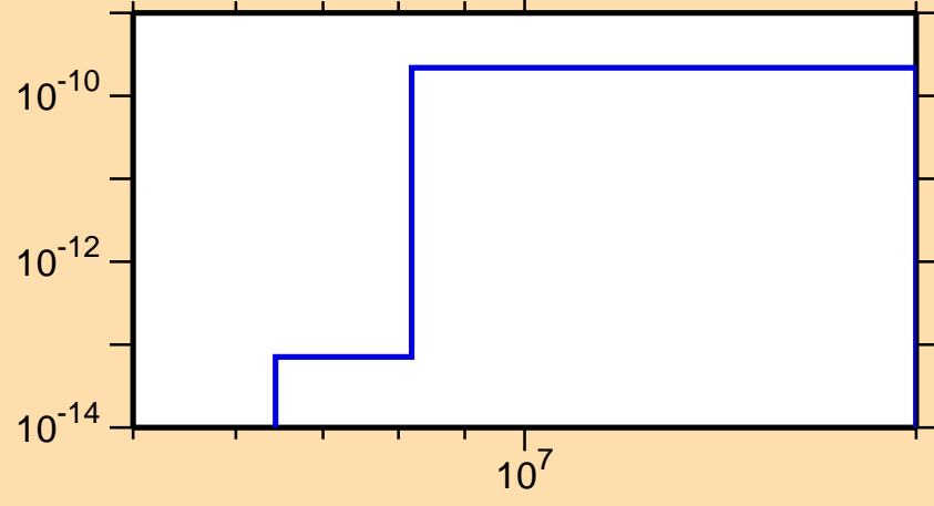
\sigma vs. E for ^{239}\text{Cf}(n,2n\alpha)
