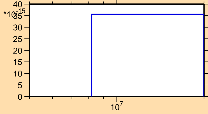
\sigma vs. E for ^{239}\text{Cf}(n,3n\alpha)
