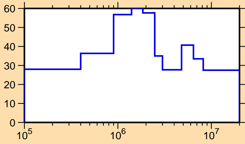
\Delta\sigma/\sigma vs. E for ^{239}\text{Cf}(n,f)
