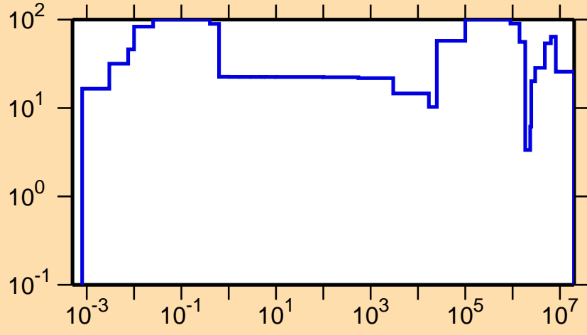
\Delta\sigma/\sigma vs. E for ^{239}\text{Cf}(n,\text{el.})
