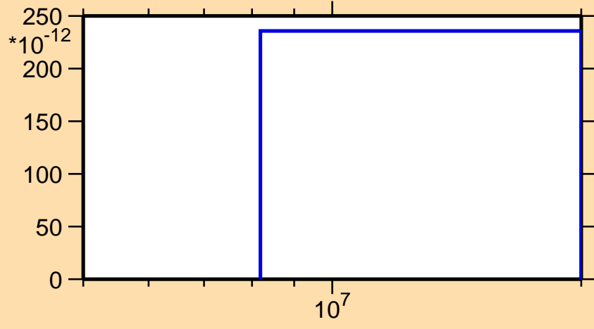
\sigma vs. E for ^{239}\text{Cf}(n,nd)
