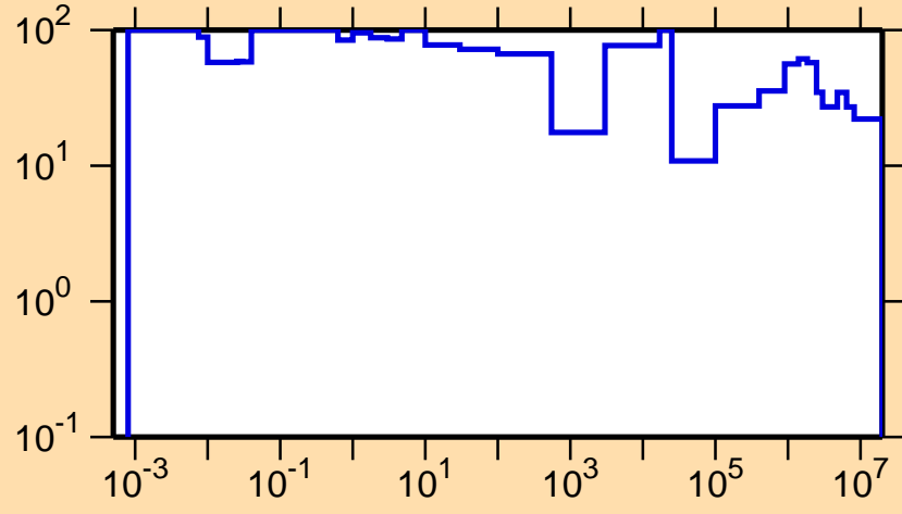
\Delta\sigma/\sigma vs. E for ^{239}\text{Cf}(n,\text{nonel.})
