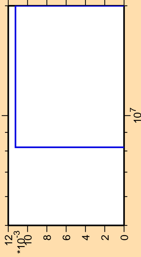
\Delta\sigma/\sigma vs. E for ^{239}\text{Cf}(n,3n\alpha)
