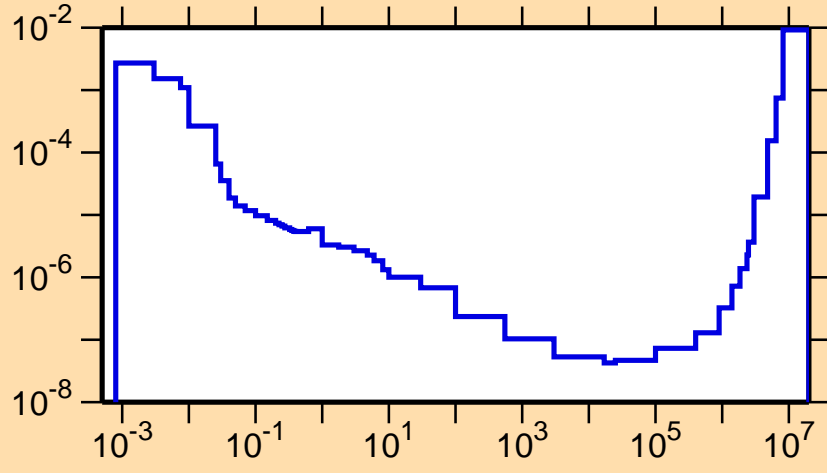
\sigma vs. E for ^{239}\text{Cf}(n,p)
