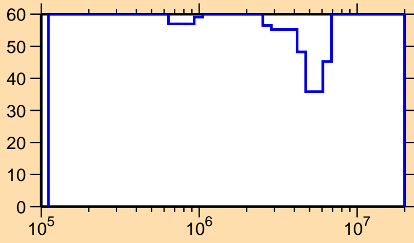
\Delta\sigma/\sigma vs. E for ^{240}\text{Cf}(n,n\text{cont.})
