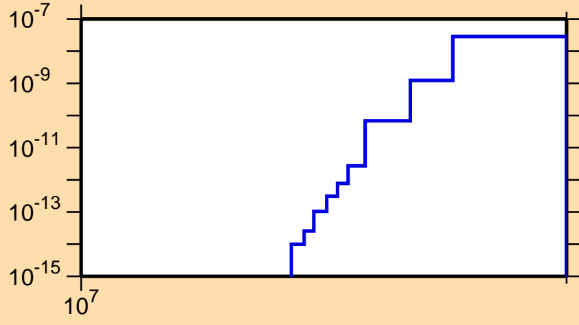
\sigma vs. E for ^{240}\text{Cf}(n,nd)
