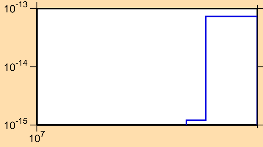
\sigma vs. E for ^{240}\text{Cf} (mt 34)
