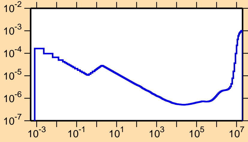
\sigma vs. E for ^{240}\text{Cf}(n,\alpha)
