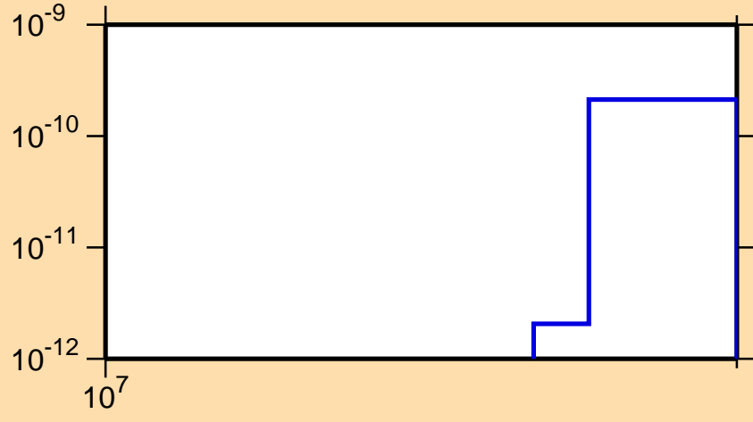
\sigma vs. E for ^{240}\text{Cf}(n,nt)
