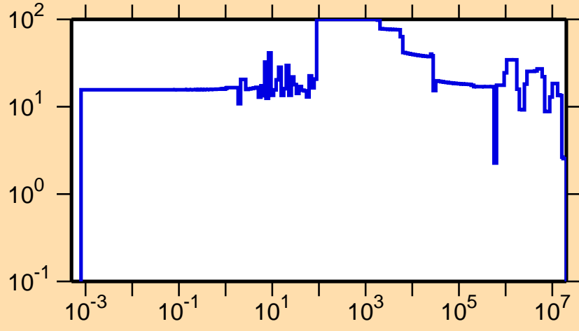
\Delta\sigma/\sigma vs. E for ^{240}\text{Cf}(n,el.)
