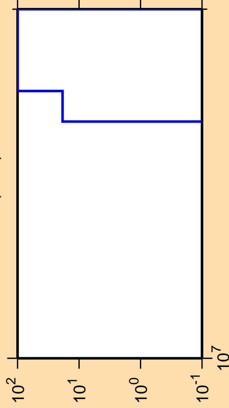
\Delta\sigma/\sigma vs. E for ^{240}\text{Cf}(n,nt)
