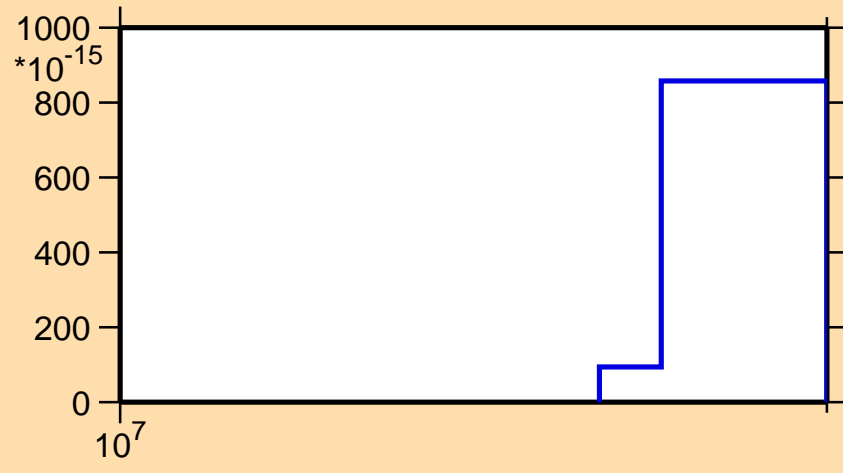
\sigma vs. E for ^{240}\text{Cf}(n,3n\alpha)
