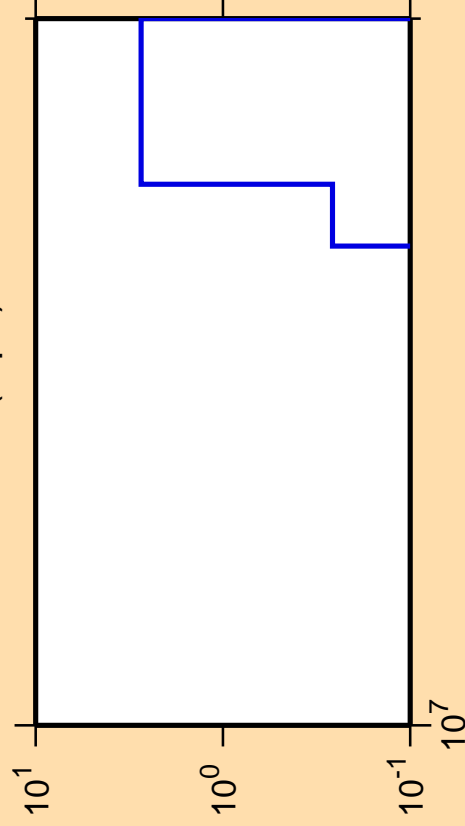
\Delta\sigma/\sigma vs. E for ^{240}\text{Cf}(n,\text{pd})
