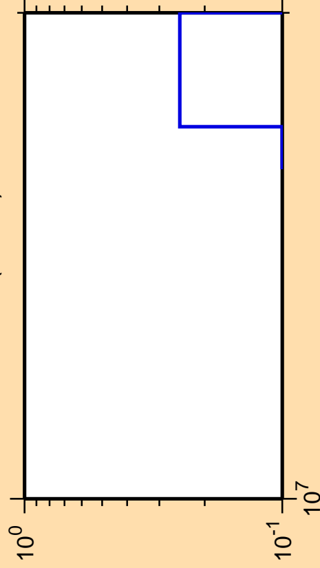
\Delta\sigma/\sigma vs. E for ^{240}\text{Cf} (mt 34)
