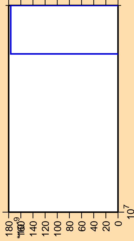
\Delta\sigma/\sigma vs. E for ^{240}\text{Cf} (mt 42)
