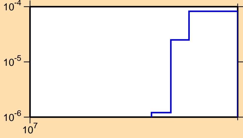
\sigma vs. E for ^{240}\text{Cf}(n,3n)
