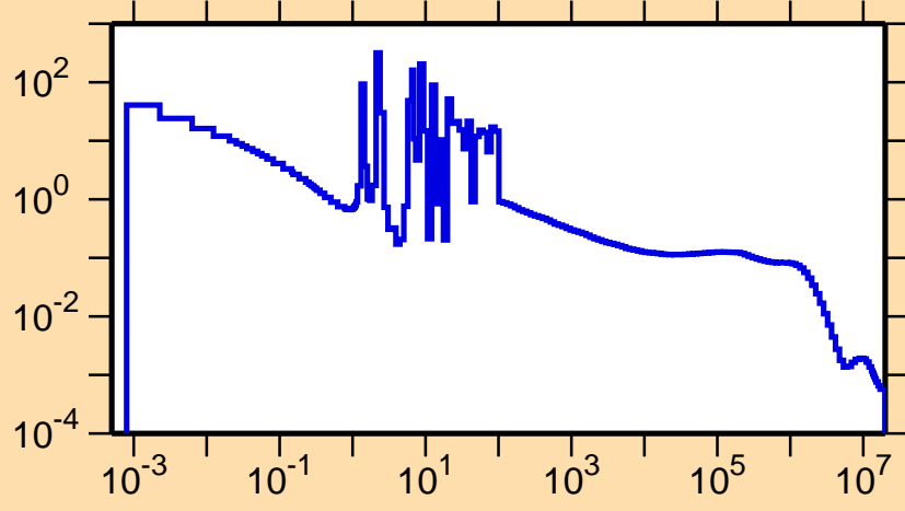
\sigma vs. E for ^{240}\text{Cf}(n,\gamma)
