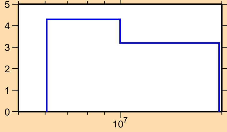
\Delta\sigma/\sigma vs. E for ^{240}\text{Cf}(n,\text{nonel.})
