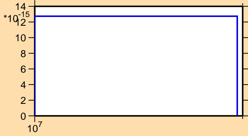
\sigma vs. E for ^{240}\text{Cf}(n,pd)
