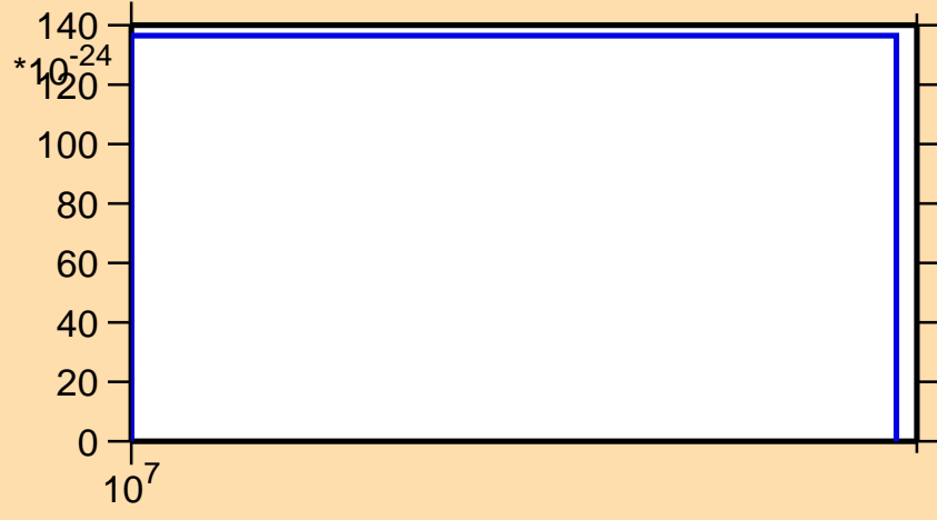
\sigma vs. E for ^{240}\text{Cf} (mt 42)
