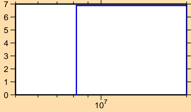
\Delta\sigma/\sigma vs. E for ^{240}\text{Cf}(n,\text{tot.})
