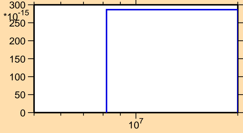
\sigma vs. E for ^{240}\text{Cf}(\text{mt } 45)
