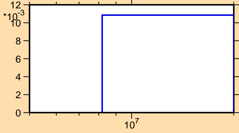
\sigma vs. E for ^{240}\text{Cf}(n,2n)
