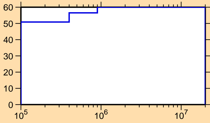
\Delta\sigma/\sigma vs. E for ^{240}\text{Cf}(n,n_1)
