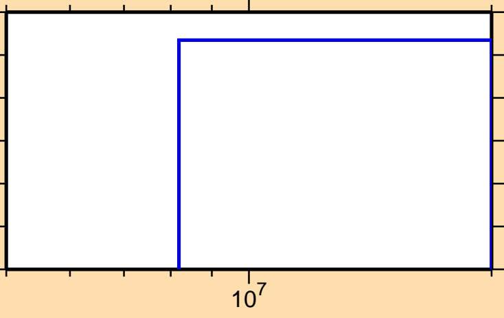
\sigma vs. E for ^{240}\text{Cf}(n,pd)
