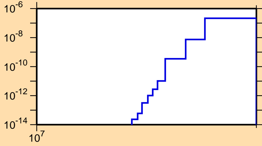
\sigma vs. E for ^{242}\text{Cf}(n,nd)
