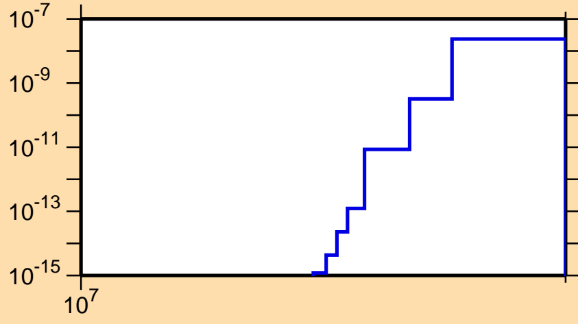
\sigma vs. E for ^{242}\text{Cf}(n,nt)
