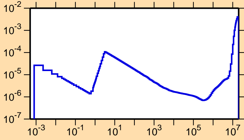
\sigma vs. E for ^{242}\text{Cf}(n,\alpha)
