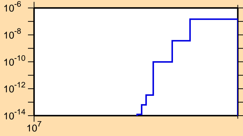
\sigma vs. E for ^{242}\text{Cf}(n,2np)
