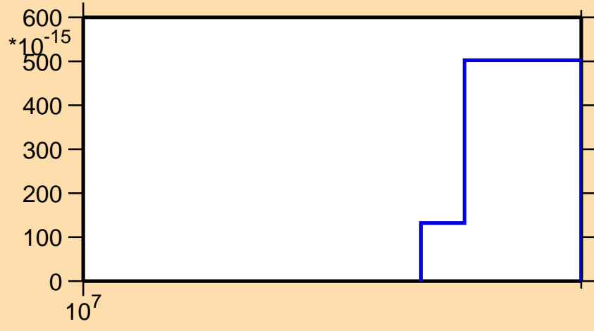
\sigma vs. E for ^{242}\text{Cf} (mt 45)
