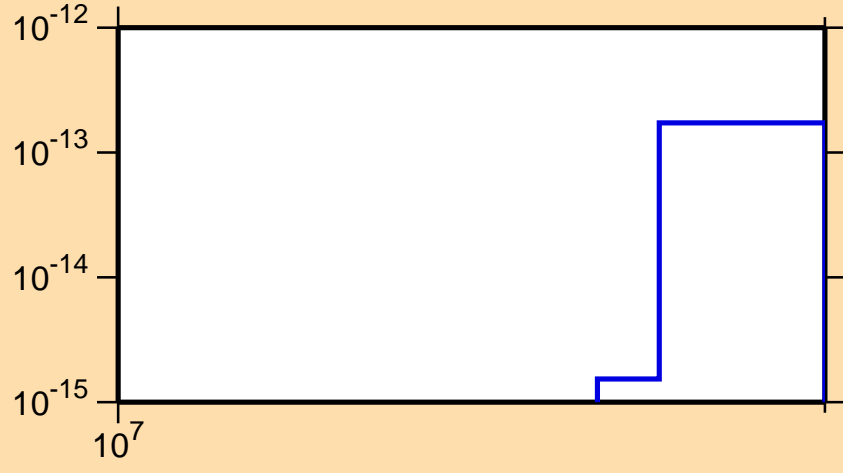
\sigma vs. E for ^{242}\text{Cf}(\text{mt } 34)
