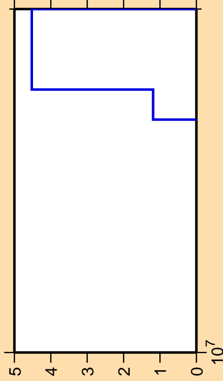
\Delta\sigma/\sigma vs. E for ^{242}\text{Cf} (mt 45)
