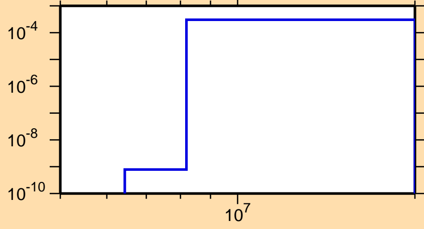
\sigma vs. E for ^{242}\text{Cf}(n,np)
