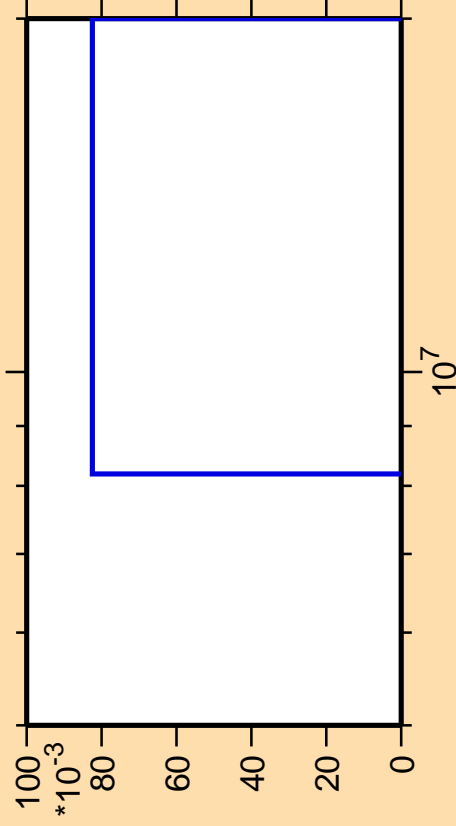
\Delta\sigma/\sigma vs. E for ^{242}\text{Cf}(\text{mt } 45)
