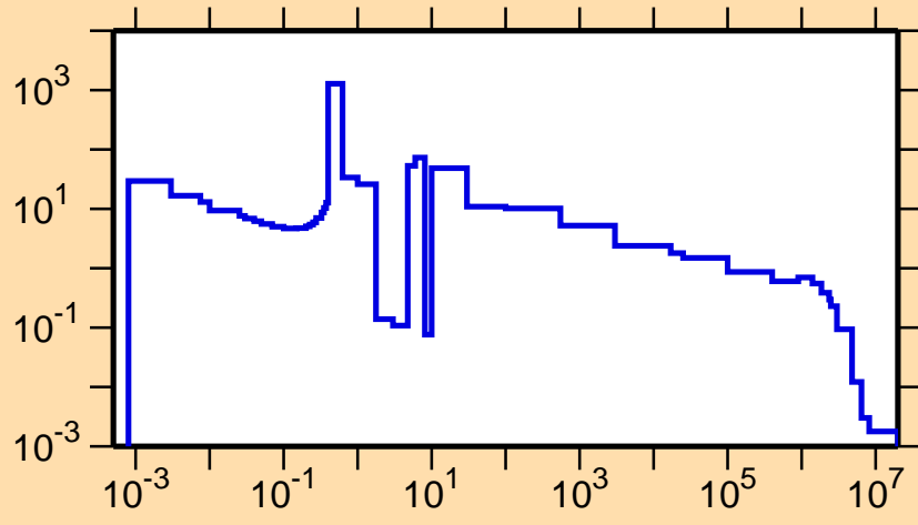
\sigma vs. E for ^{242}\text{Cf}(n,\gamma)
