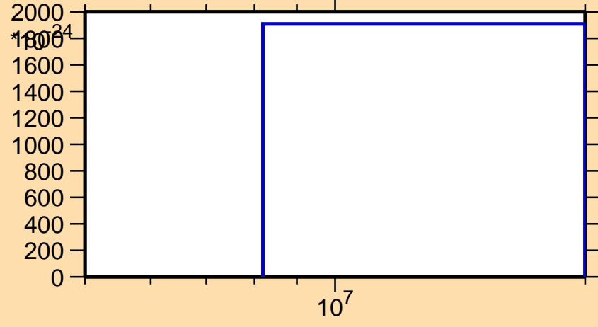
\sigma vs. E for ^{242}\text{Cf}(\text{mt } 42)
