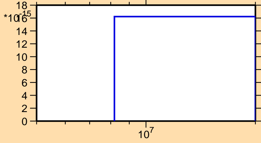
\sigma vs. E for ^{242}\text{Cf}(\text{mt } 45)
