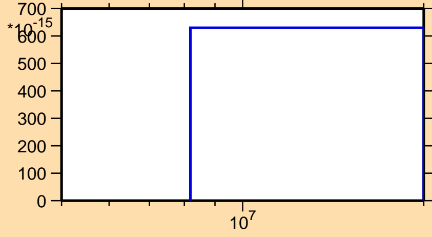
\sigma vs. E for ^{242}\text{Cf}(n,3n\alpha)
