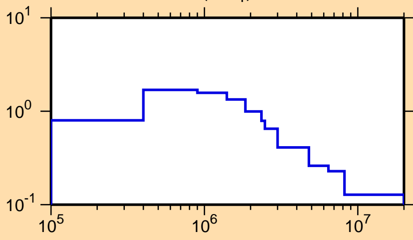
\sigma vs. E for ^{242}\text{Cf}(n,n_1)
