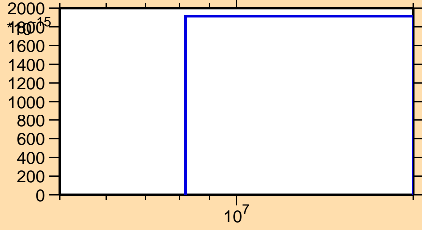
\sigma vs. E for ^{242}\text{Cf}(n,p\alpha)
