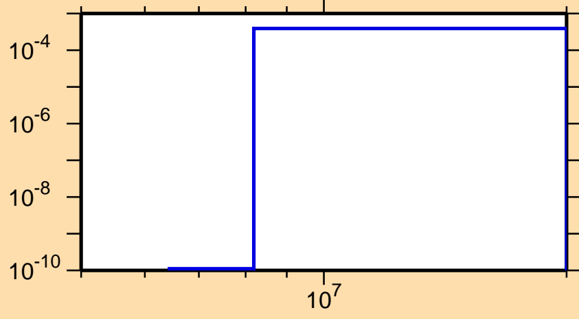
\sigma vs. E for ^{242}\text{Cf}(n,d)
