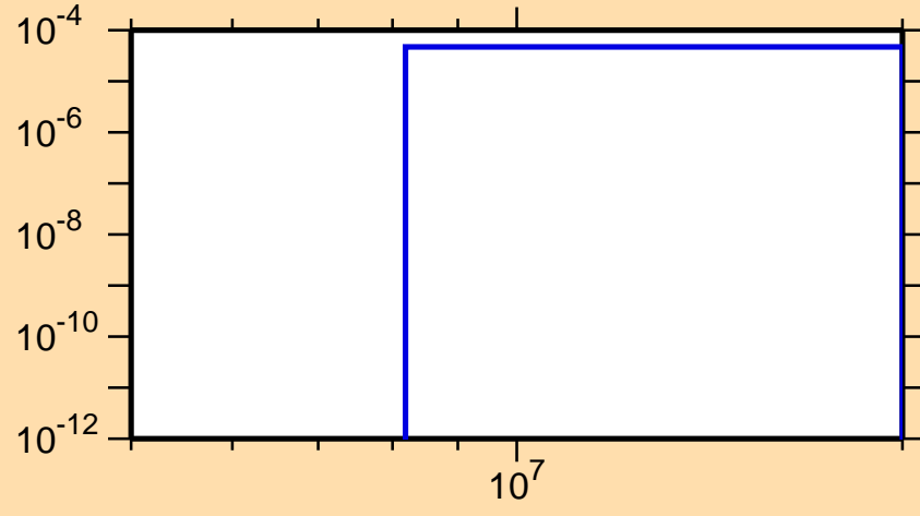
\sigma vs. E for ^{242}\text{Cf}(n,t)
