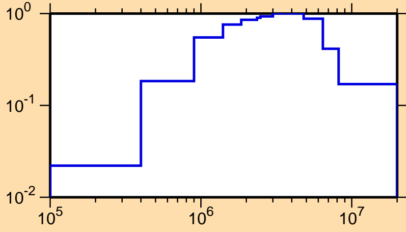
\sigma vs. E for ^{242}\text{Cf}(n,n\text{cont.})
