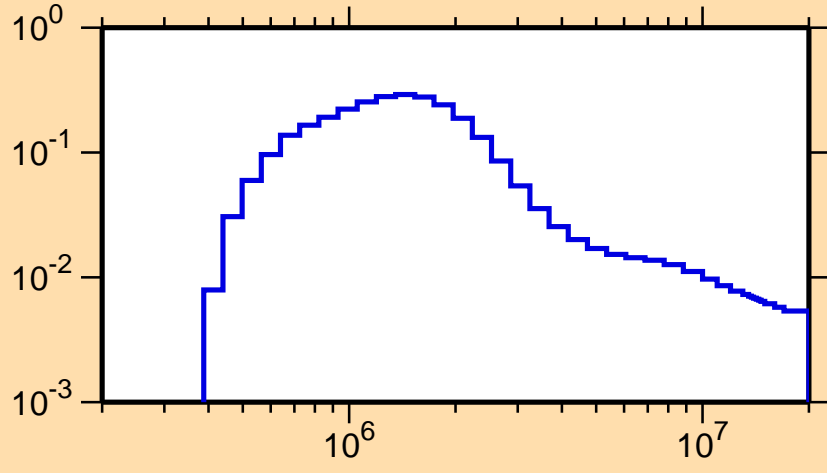
\sigma vs. E for ^{244}\text{Cf}(n,n_3)
