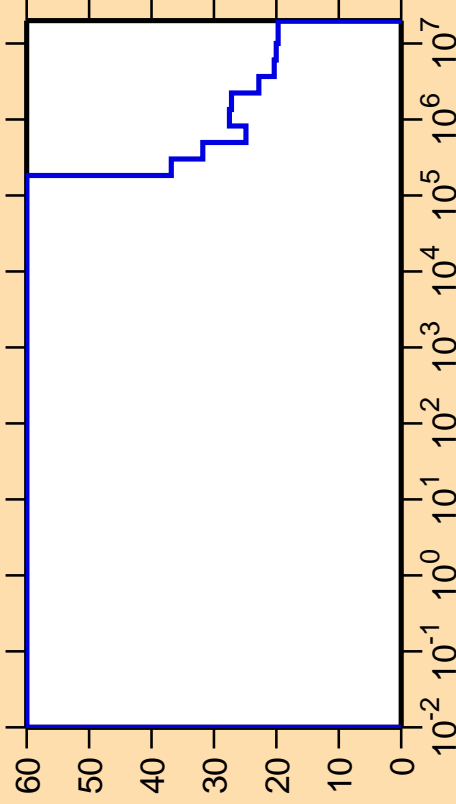
\Delta\sigma/\sigma vs. E for ^{244}\text{Cf}(n,\text{nonel.})
