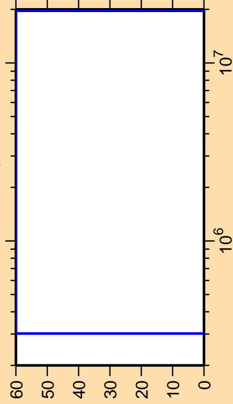
\Delta\sigma/\sigma vs. E for ^{244}\text{Cf}(n,n_3)
