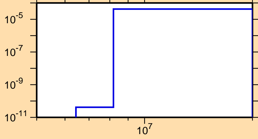
\sigma vs. E for ^{244}\text{Cf}(n,np)
