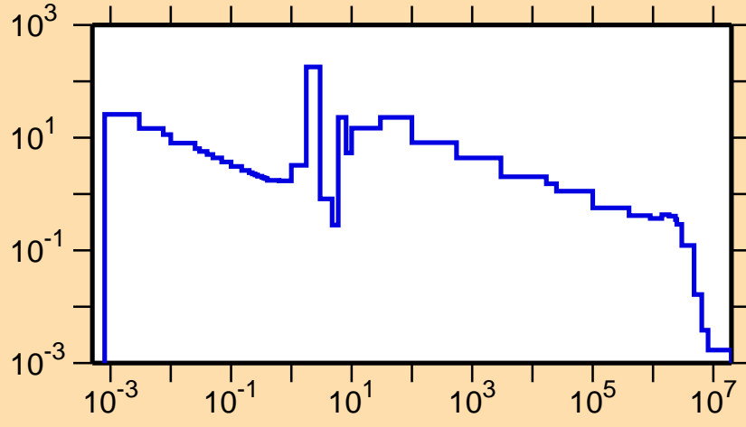
\sigma vs. E for ^{244}\text{Cf}(n,\gamma)
