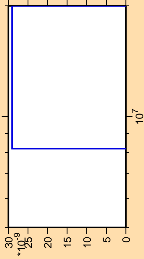
\Delta\sigma/\sigma vs. E for ^{244}\text{Cf}(\text{mt } 42)
