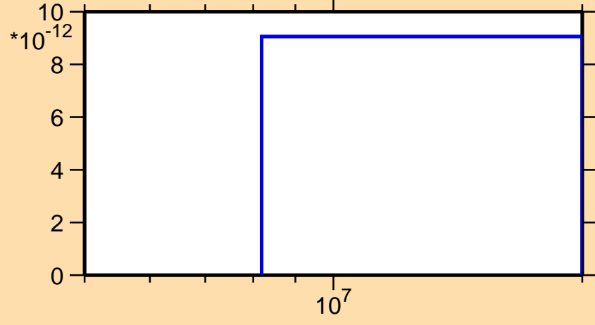
\sigma vs. E for ^{244}\text{Cf}(n,3n\alpha)
