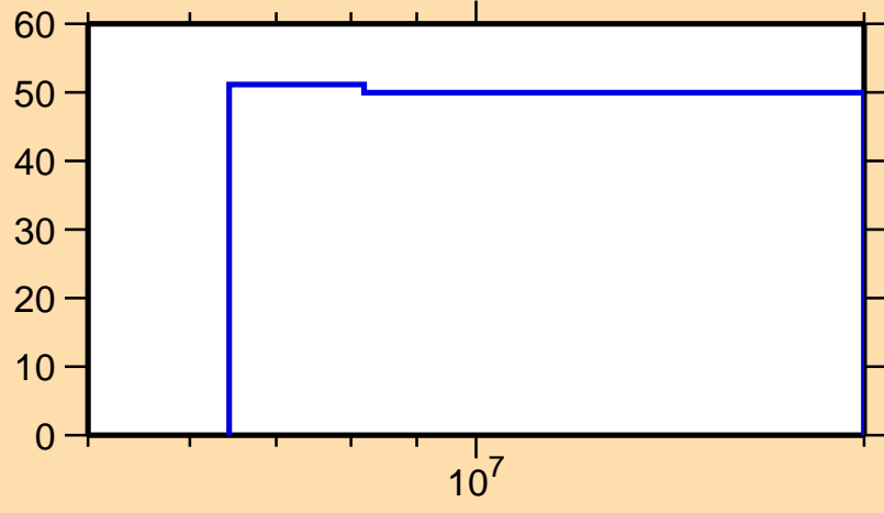
\Delta\sigma/\sigma vs. E for ^{244}\text{Cf}(n,\text{inel.})
