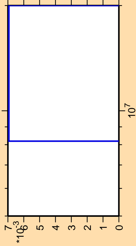
\Delta\sigma/\sigma vs. E for ^{244}\text{Cf}(\text{mt } 34)
