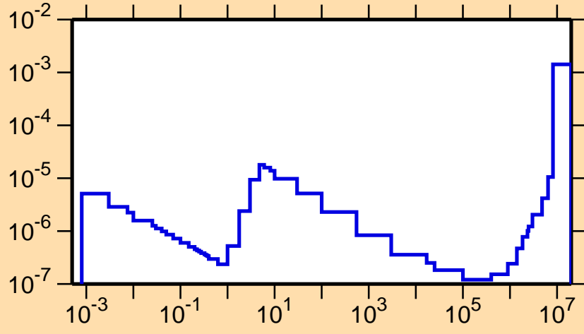
\sigma vs. E for ^{244}\text{Cf}(n,\alpha)
