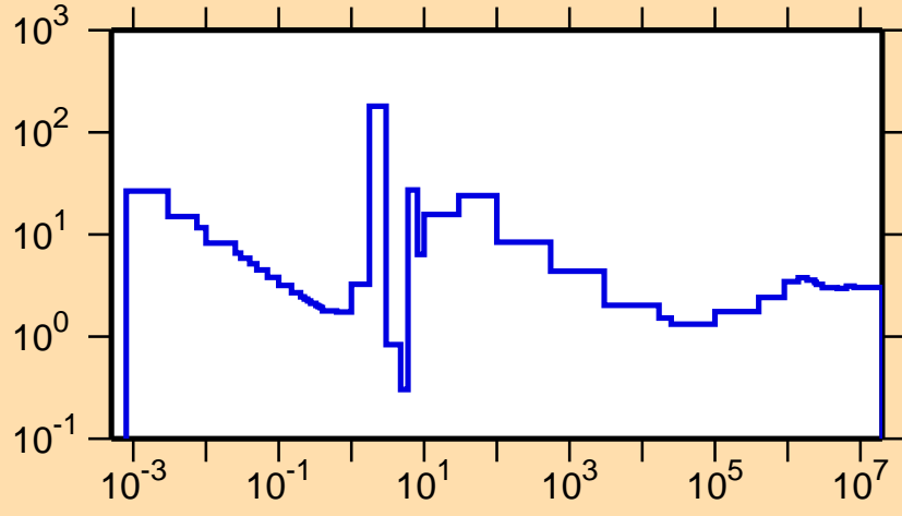
\sigma vs. E for ^{244}\text{Cf}(n,\text{nonel.})
