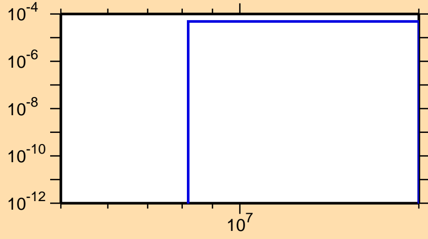
\sigma vs. E for ^{244}\text{Cf}(n,t)
