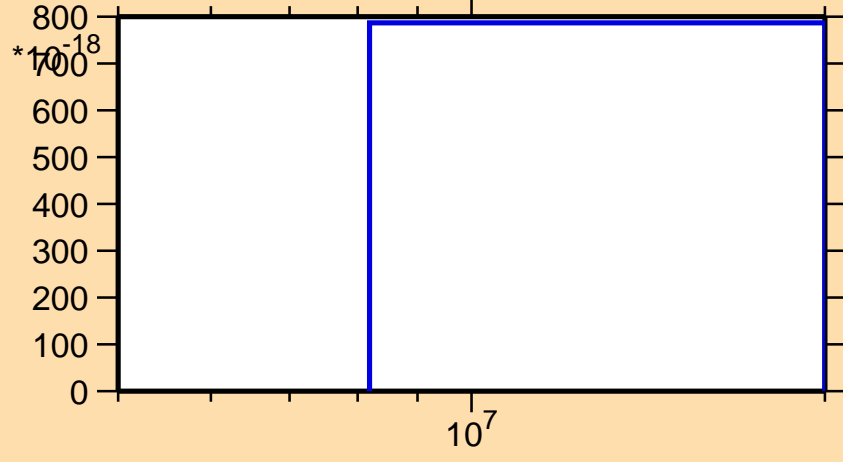
\sigma vs. E for ^{244}\text{Cf}(\text{mt } 34)
