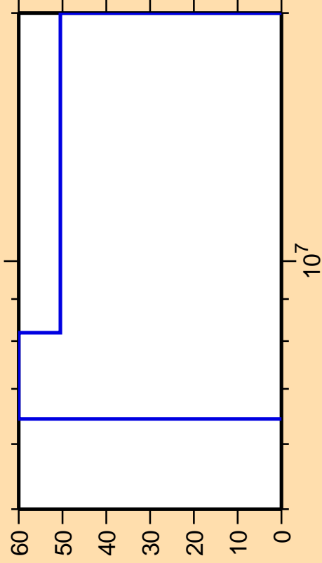
\Delta\sigma/\sigma vs. E for ^{244}\text{Cf}(n,f)
