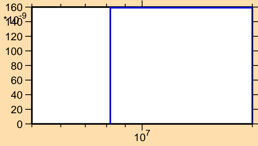
\sigma vs. E for ^{244}\text{Cf}(\text{mt117})
