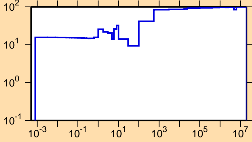
\Delta\sigma/\sigma vs. E for ^{244}\text{Cf}(n,\gamma)
