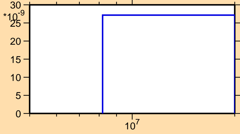
\sigma vs. E for ^{244}\text{Cf}(\text{mt } 45)
