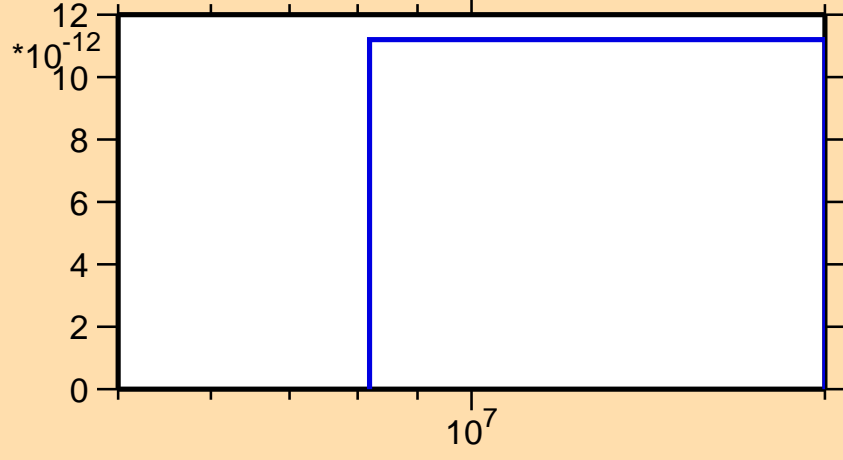
\sigma vs. E for ^{244}\text{Cf}(n,p\alpha)
