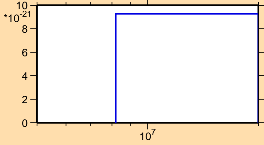
\sigma vs. E for ^{244}\text{Cf}(\text{mt } 42)
