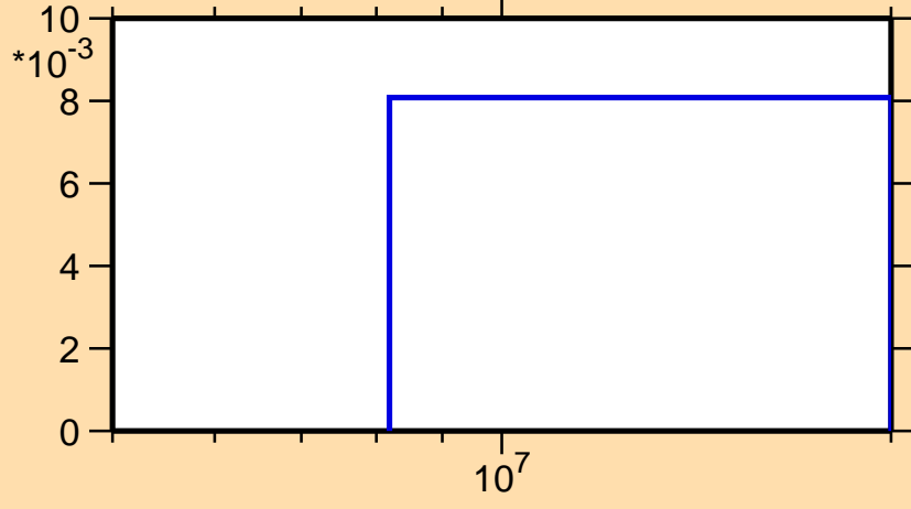
\sigma vs. E for ^{244}\text{Cf}(n,3n)
