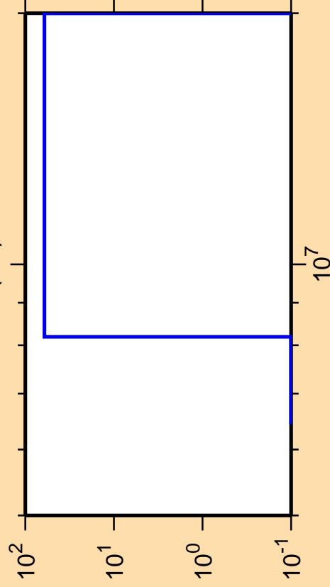
\Delta\sigma/\sigma vs. E for ^{244}\text{Cf}(n,t)
