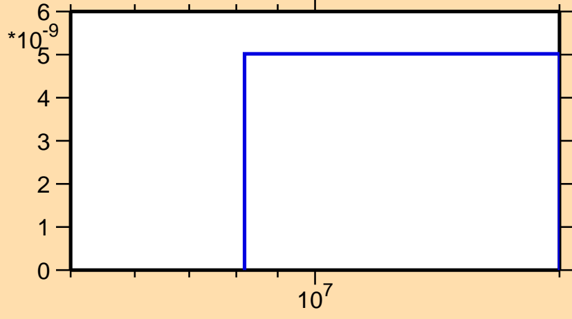
\sigma vs. E for ^{244}\text{Cf}(n,nd)
