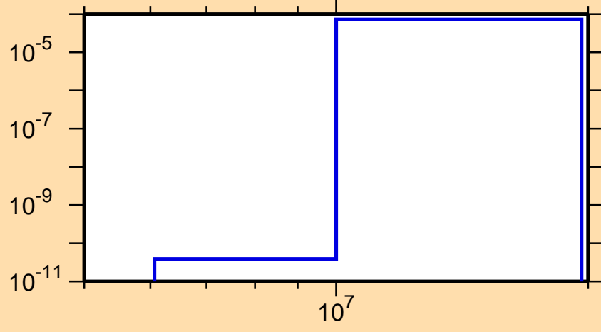
\sigma vs. E for ^{245}\text{Cf}(n,t)
