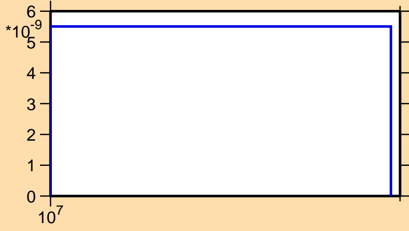
\sigma vs. E for ^{245}\text{Cf}(n,2np)
