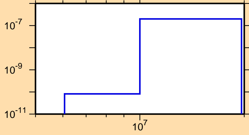
\sigma vs. E for ^{245}\text{Cf}(n,2n\alpha)
