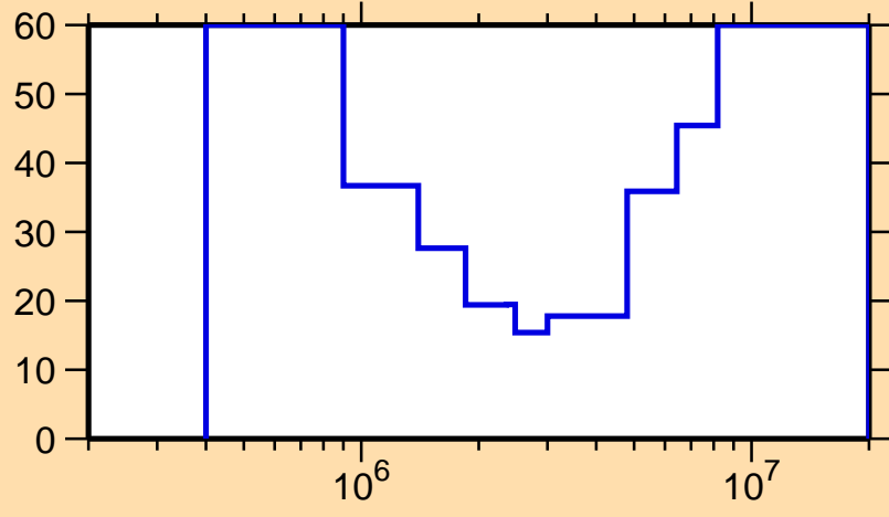
\Delta\sigma/\sigma vs. E for ^{245}\text{Cf}(n,n\text{cont.})
