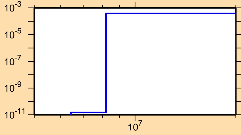
\sigma vs. E for ^{245}\text{Cf}(n,d)
