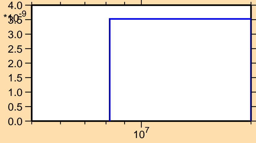
\sigma vs. E for ^{245}\text{Cf}(n,nt)
