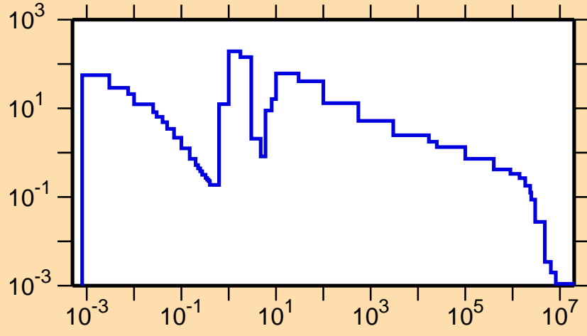
\sigma vs. E for ^{245}\text{Cf}(n,\gamma)
