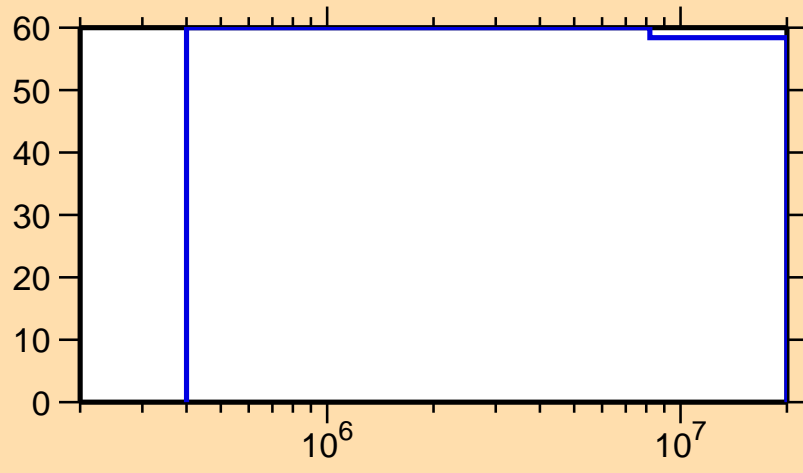
\Delta\sigma/\sigma vs. E for ^{245}\text{Cf}(n,f)
