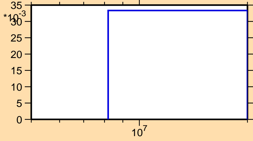
\sigma vs. E for ^{245}\text{Cf}(n,3n)
