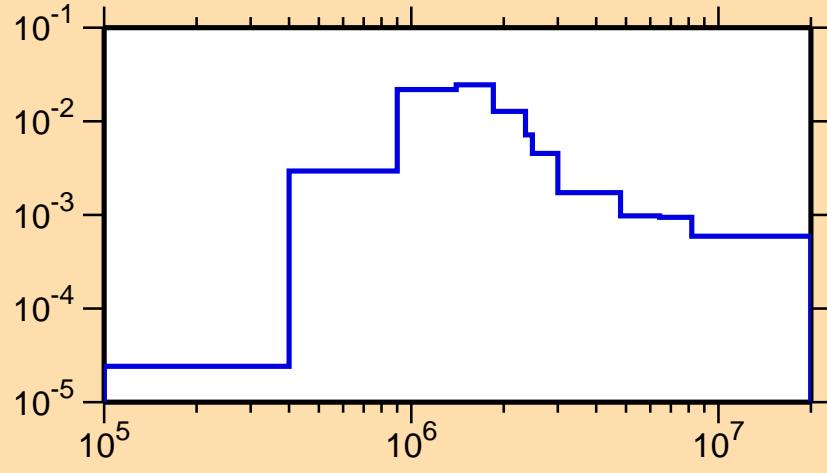
\sigma vs. E for ^{245}\text{Cf}(n,n_4)
