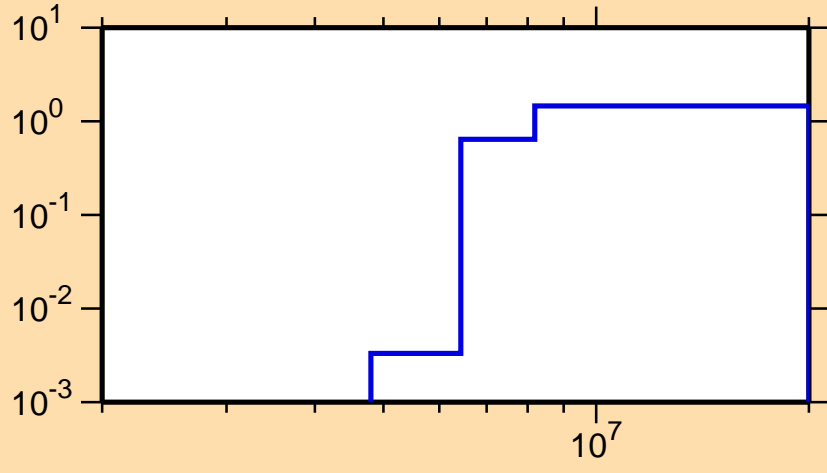
\sigma vs. E for ^{245}\text{Cf}(n,2n)
