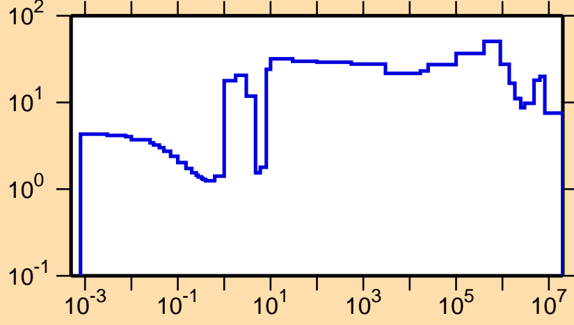
\Delta\sigma/\sigma vs. E for ^{245}\text{Cf}(n,el.)
