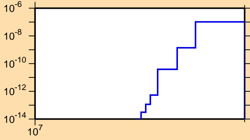
\sigma vs. E for ^{247}\text{Cf}(n,nt)
