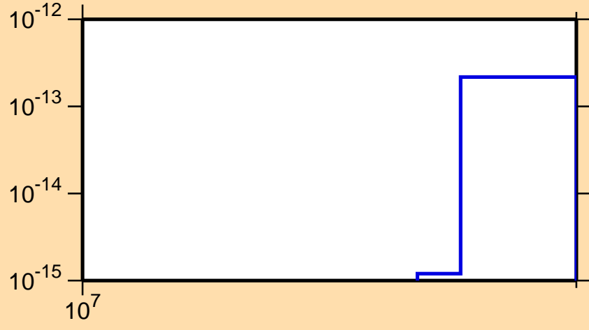
\sigma vs. E for ^{247}\text{Cf}(\text{mt } 34)
