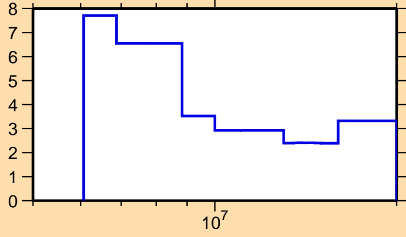
\Delta\sigma/\sigma vs. E for ^{247}\text{Cf}(n,\text{tot.})
