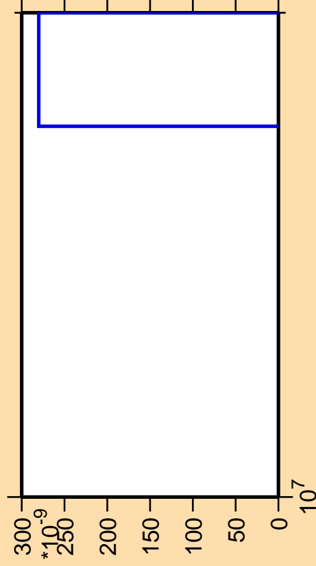
\Delta\sigma/\sigma vs. E for ^{247}\text{Cf}(\text{mt } 42)
