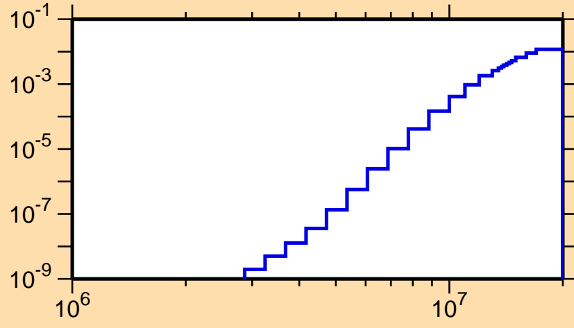
\sigma vs. E for ^{247}\text{Cf}(n,p)
