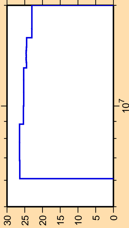
\Delta\sigma/\sigma vs. E for ^{247}\text{Cf}(n,n_1)
