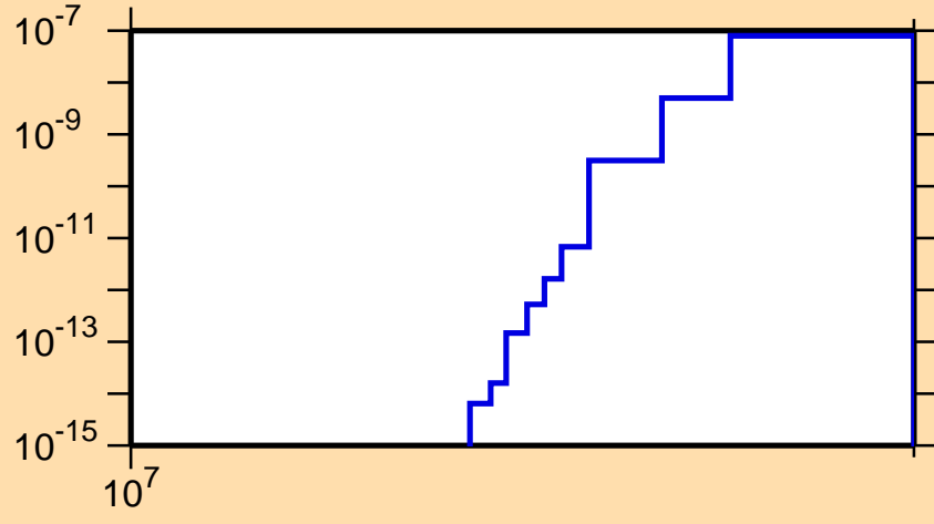
\sigma vs. E for ^{247}\text{Cf}(n,2np)
