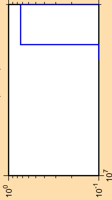
\Delta\sigma/\sigma vs. E for ^{247}\text{Cf}(\text{mt } 34)
